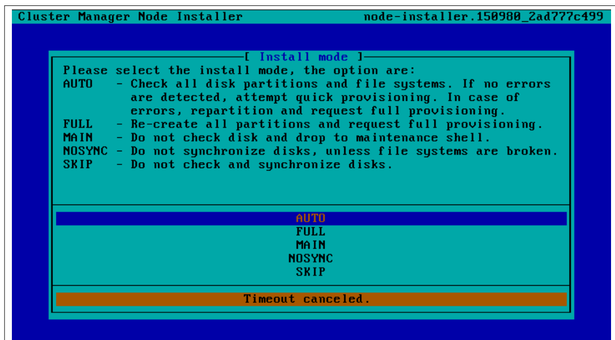
Figure 5.17: Install-mode Setting Option During Node-Installer Run
