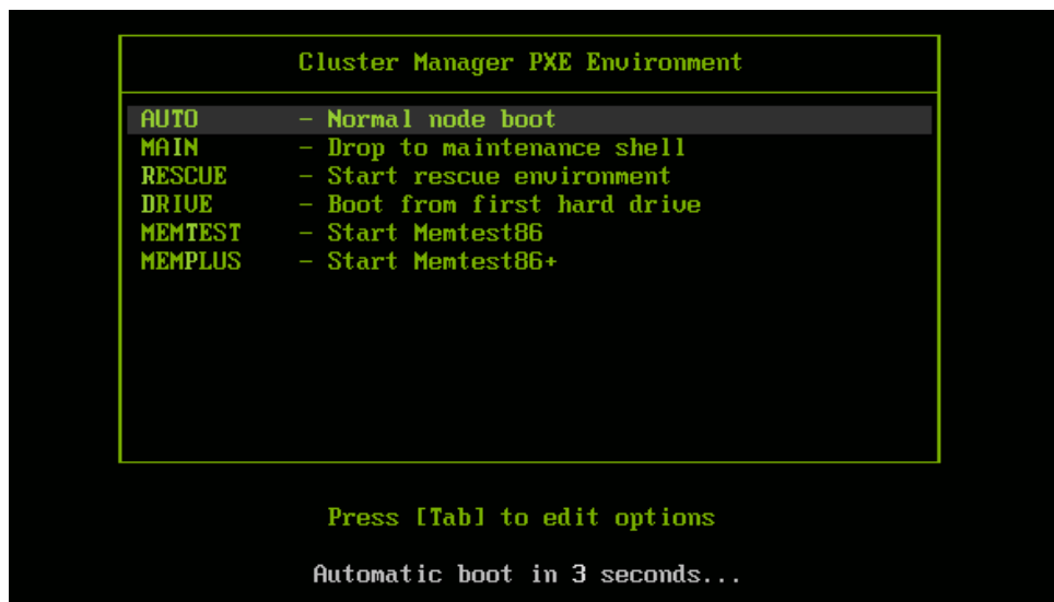
Figure 5.16: PXE Menu With Install-mode Set To AUTO
