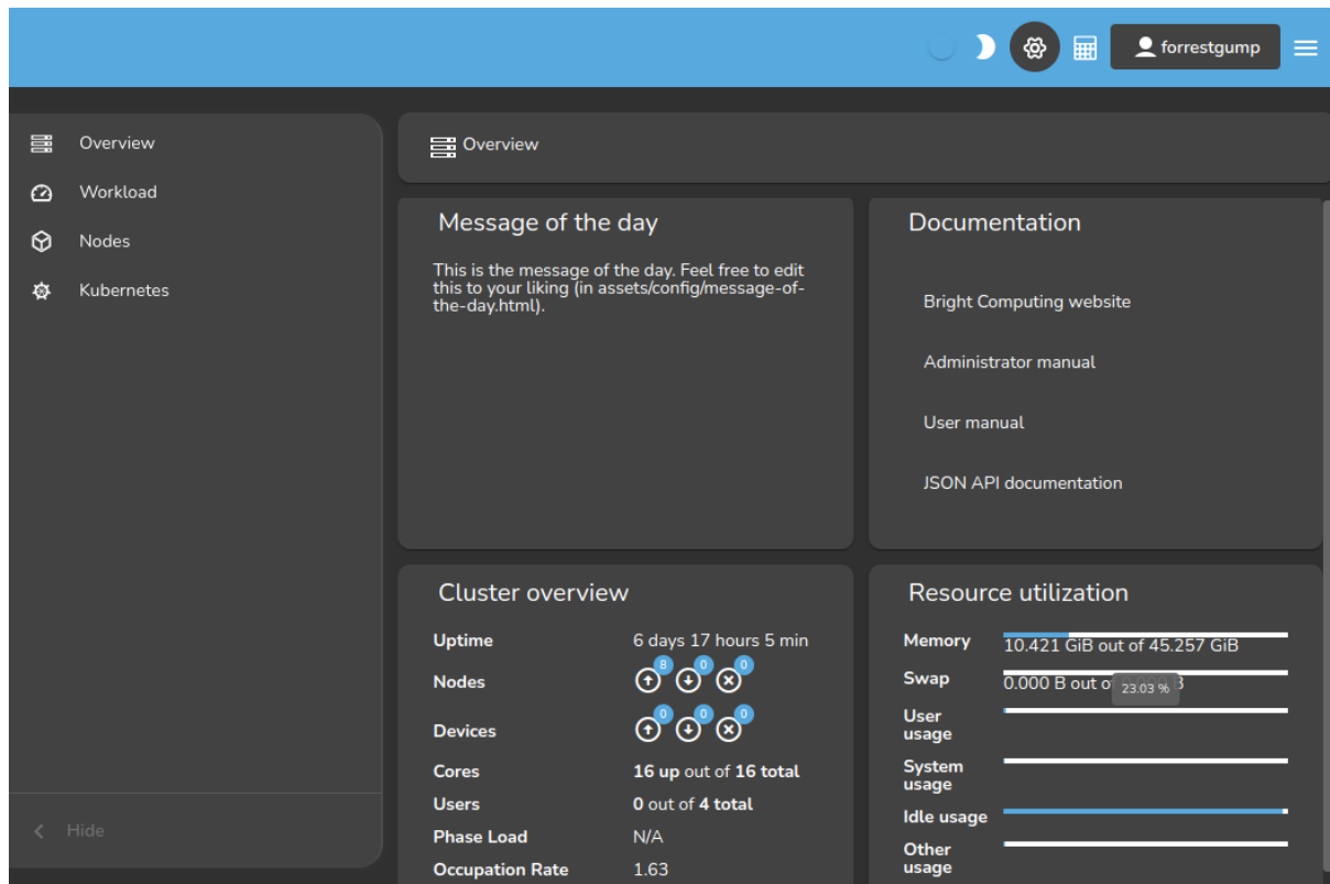
Figure 10.35: User Portal: Overview Page
