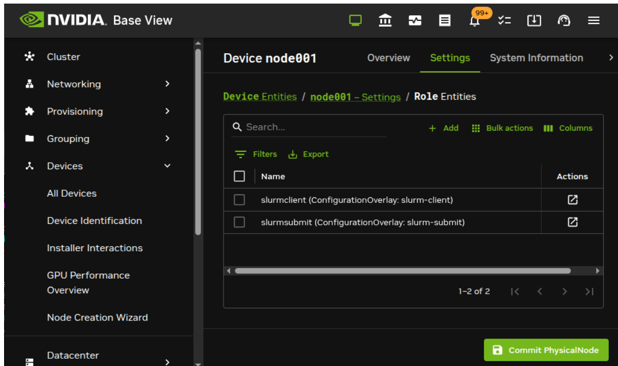
Figure 7.19: Roles seen on regular node in Base View
