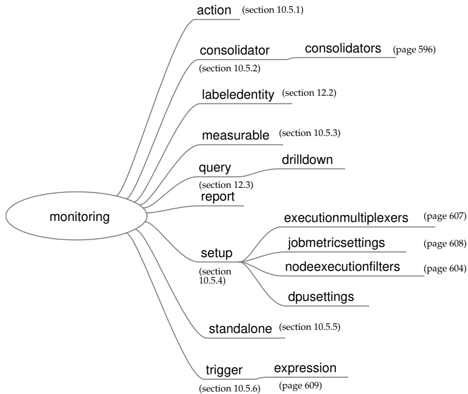
Figure 10.27: Submodes Under monitoring Mode
