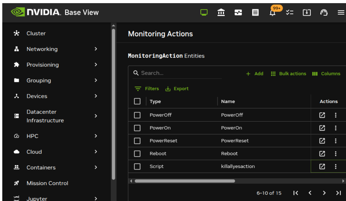
Figure 10.2: Base View Monitoring Configuration: Adding An Action
