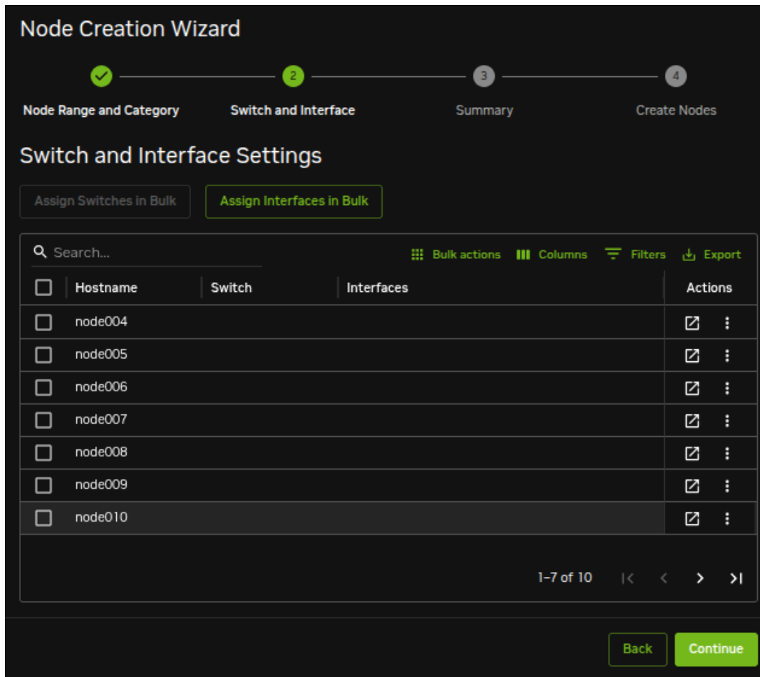
Figure 5.20: Node Creation Wizard: Switch And Interface Screen
