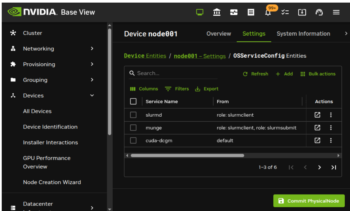
Figure 7.17: Services seen on regular node in Base View
