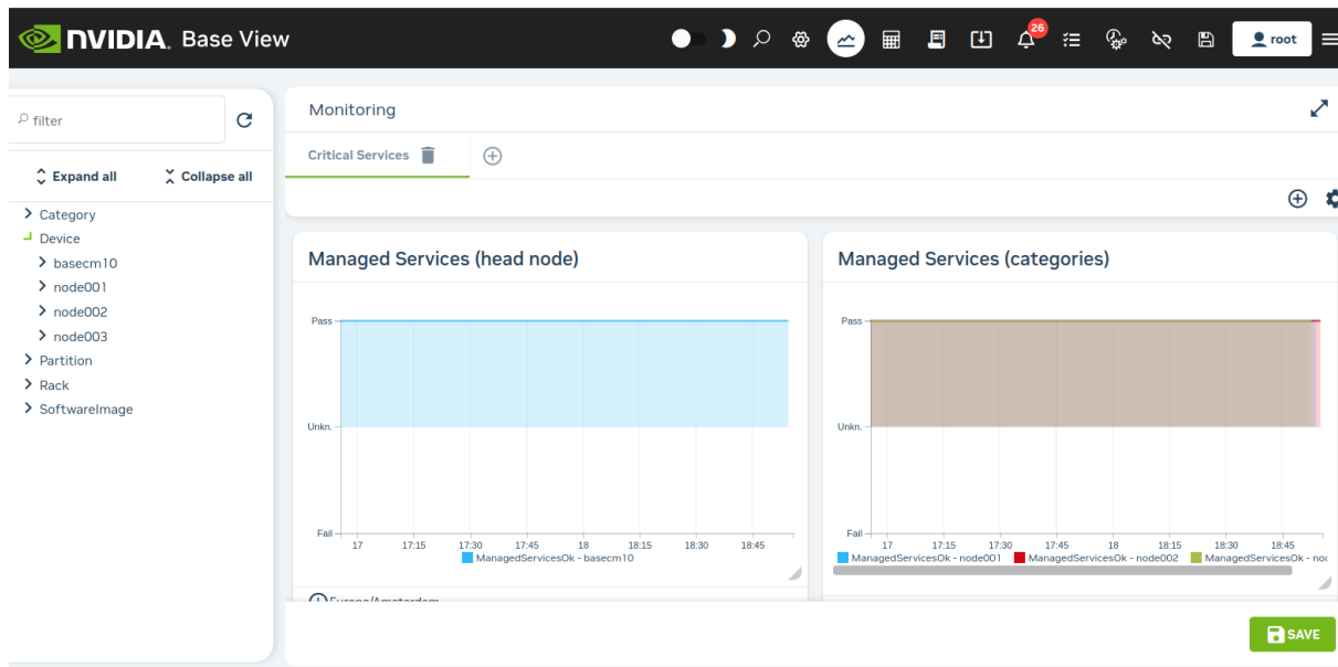
Figure 10.7: Base View Monitoring Window: Default Plot Panels
