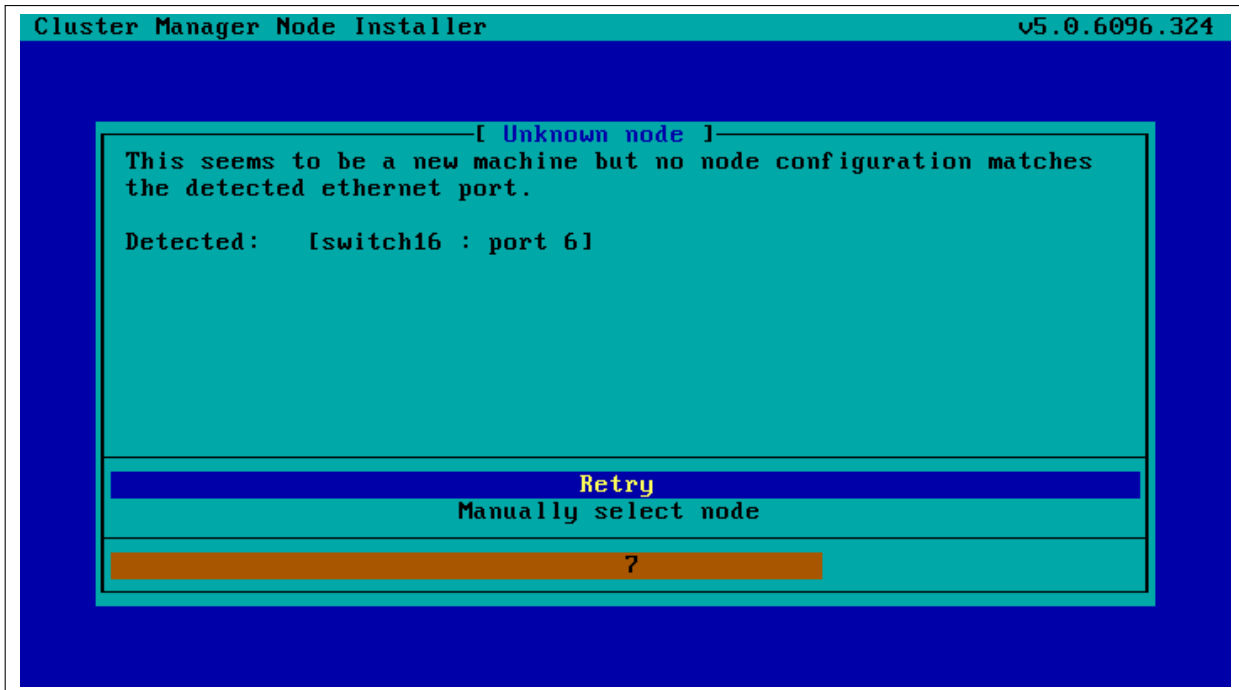
Figure 5.11: Scenarios: Unknown Node, Ethernet Port Detected
