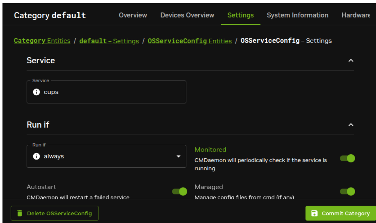
Figure 3.23: Setting up a service using Base View
