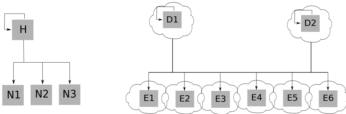
Figure 10.31: Sampling Flow For Offloaded Monitoring With Non-HA Edge Director Nodes
