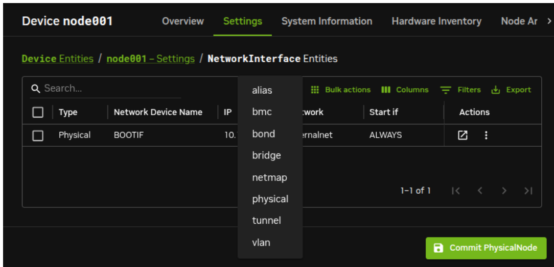
Figure 3.10: Configuring a VLAN via Base View
