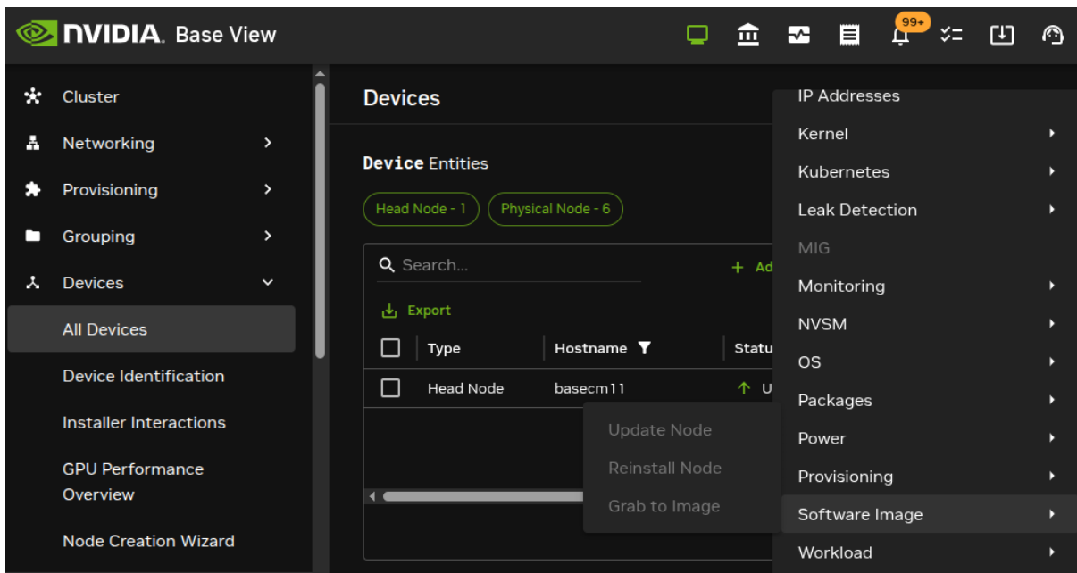
Figure 4.2: Actions button, accessing the power operations
