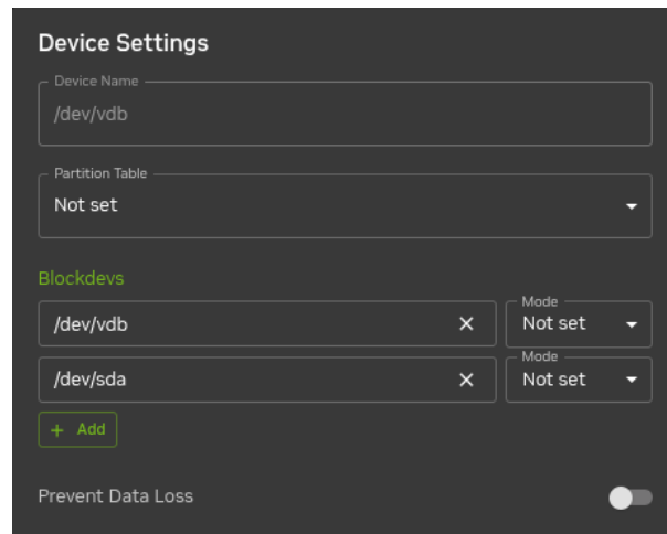
Figure 3.18: Editing disk layouts with Base View
