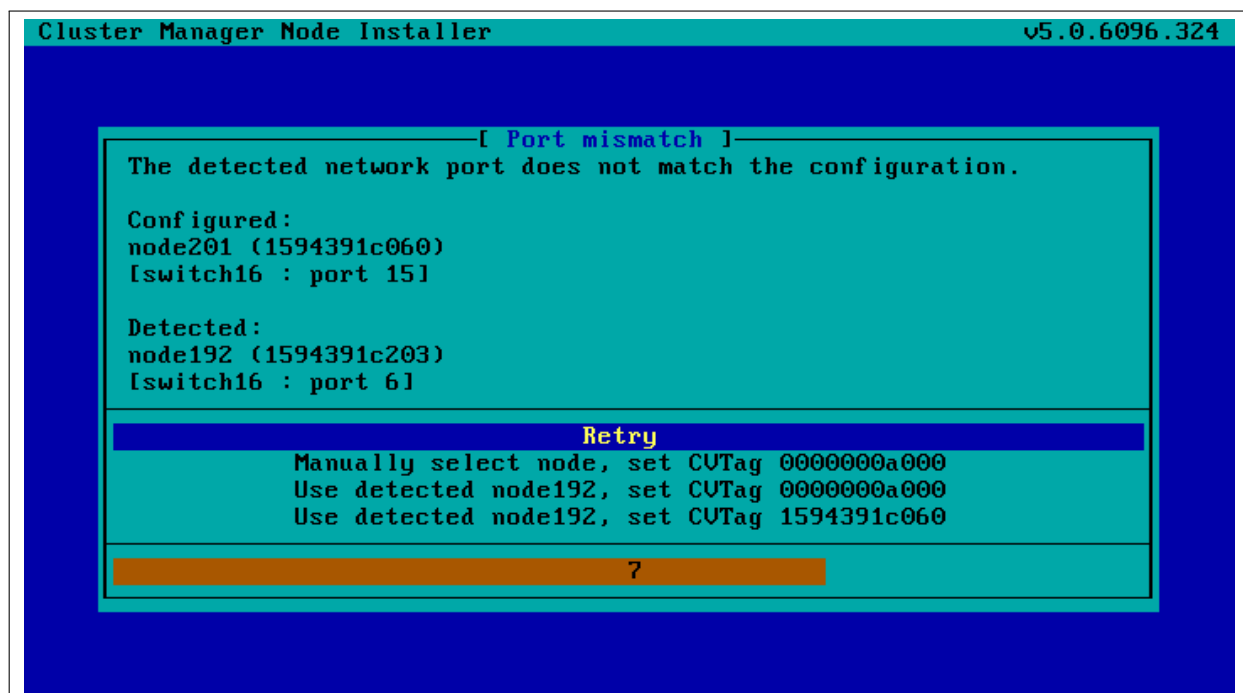
Figure 5.13: Scenarios: Port Mismatch Dialog
