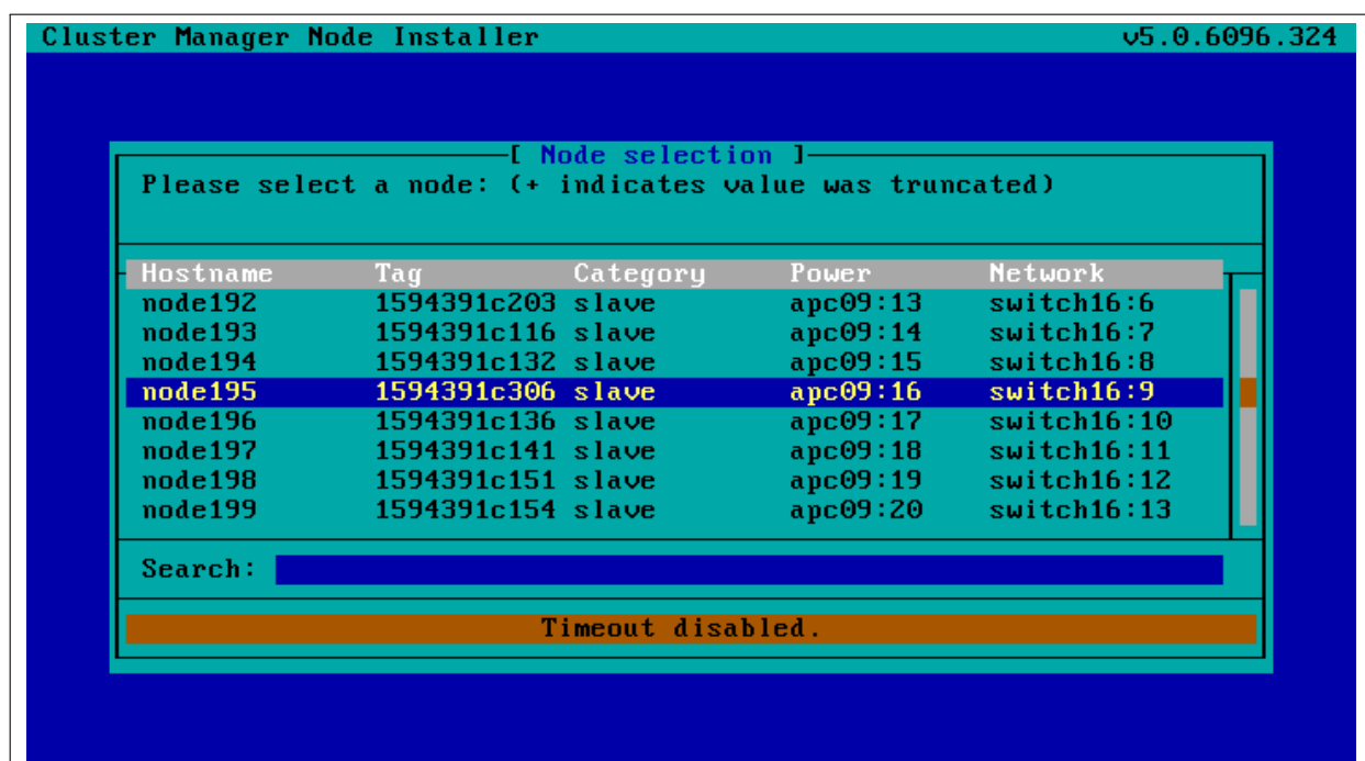
Figure 5.10: Scenarios: Node Selection Sub-Dialog
