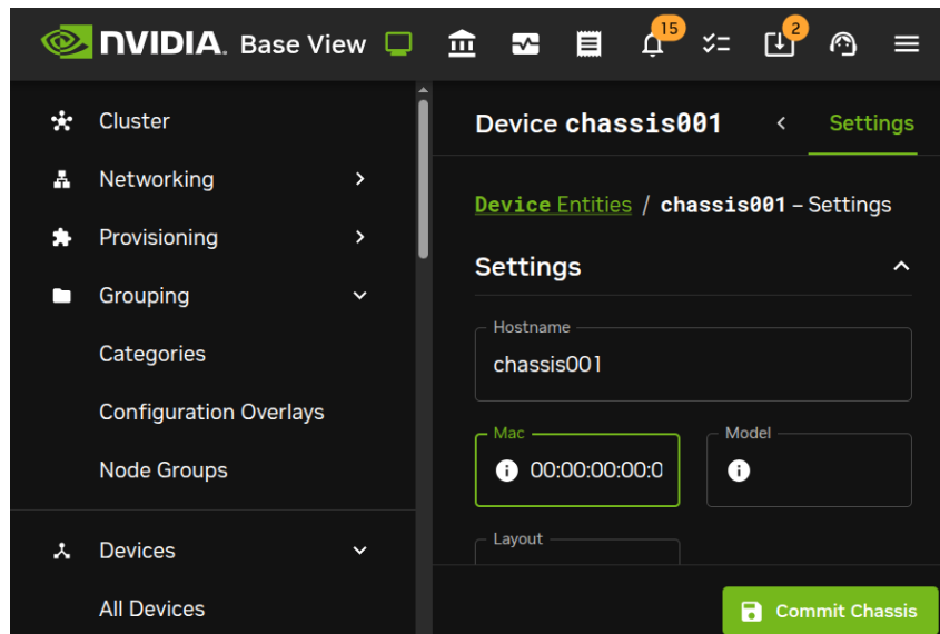
Figure 3.28: Base View chassis configuration
