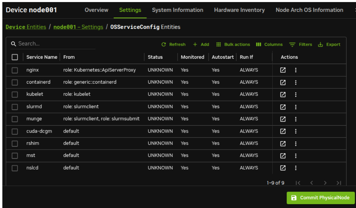
Figure 3.22: Operating system service configuration list window for nodes in Base View
