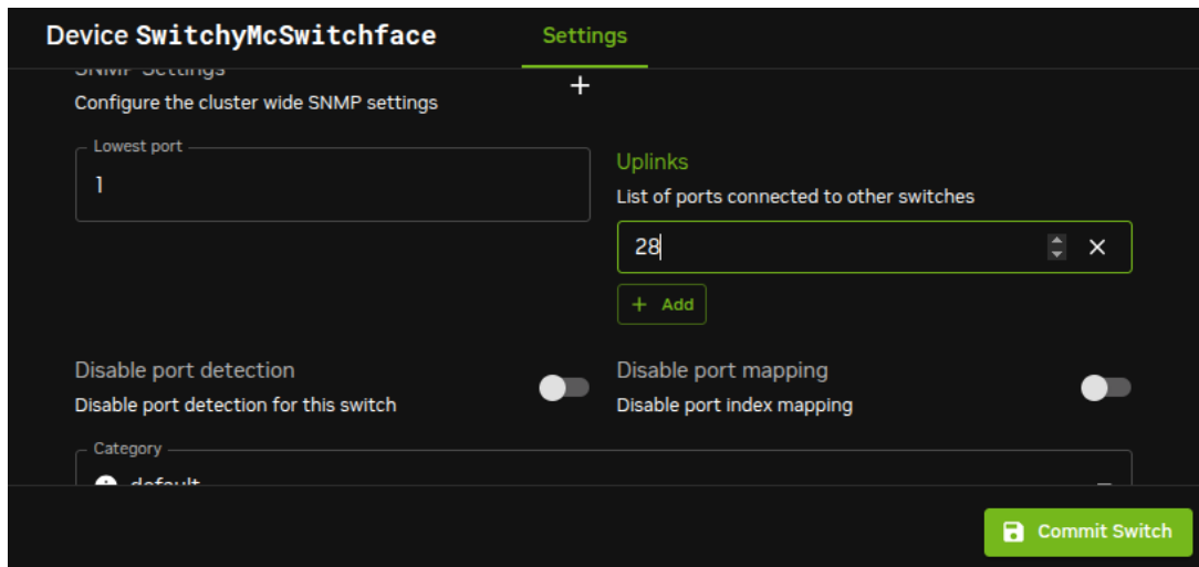
Figure 3.16: Notifying CMDaemon about uplinks with Base View
