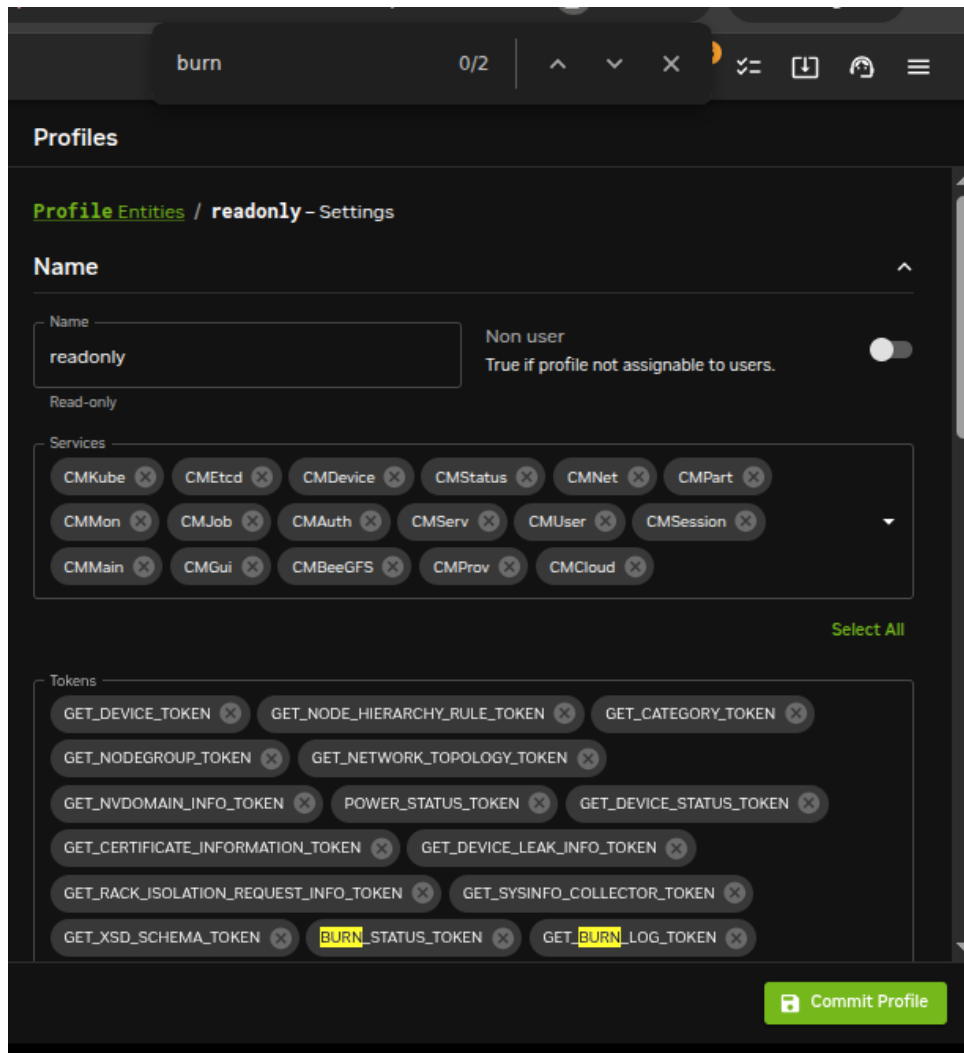
Figure 6.3: Base View Profile Token Management
