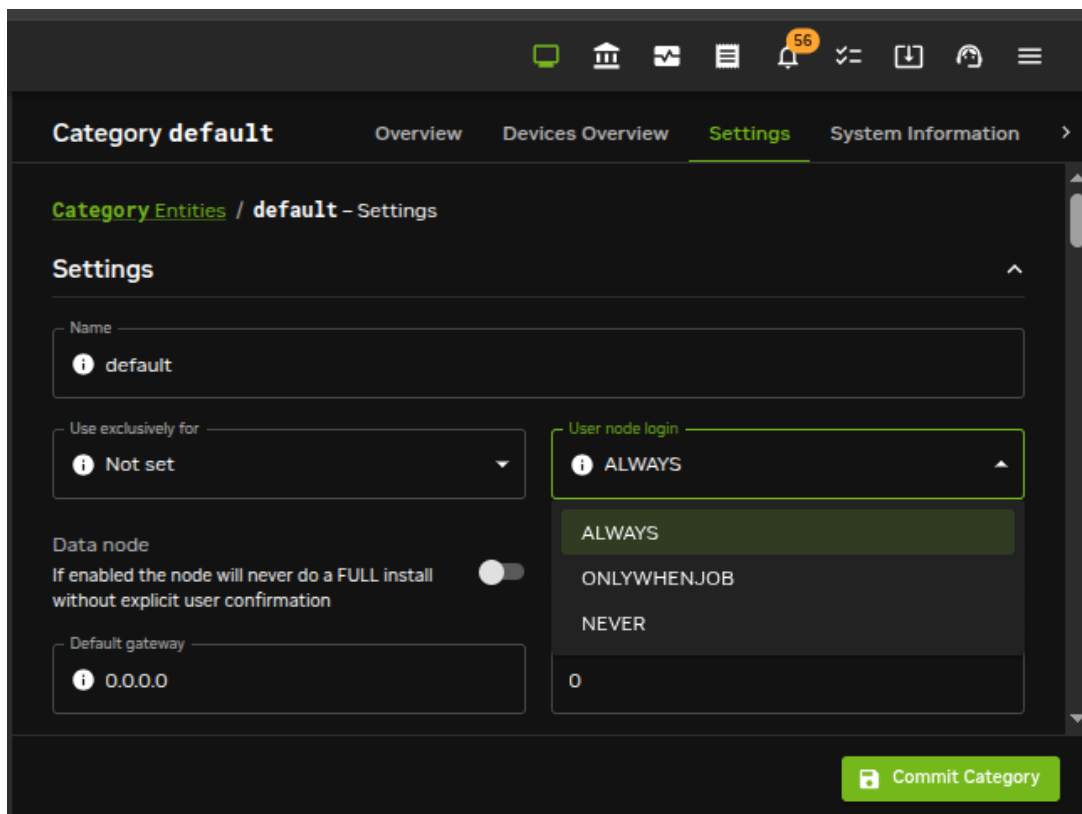
Figure 7.1: Disallowing user logins to nodes via Base View
