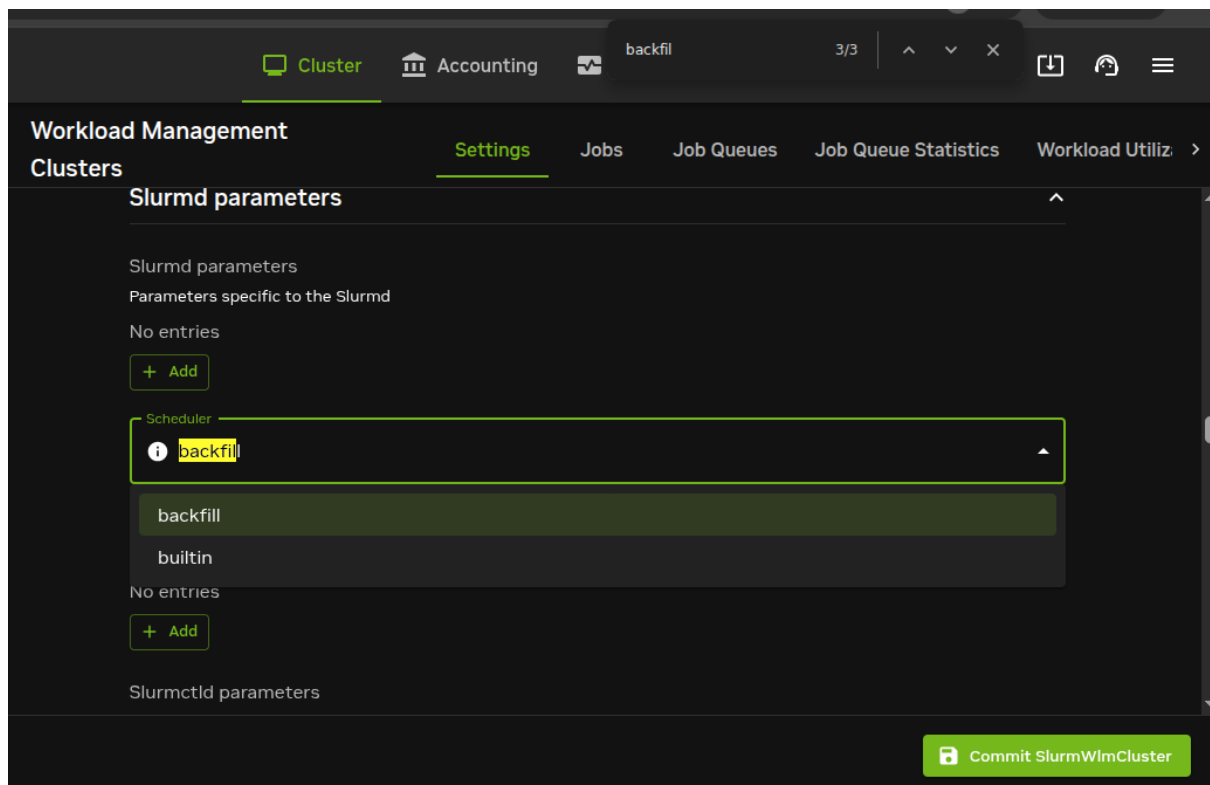
Figure 7.15: Workload management role assignment options on a head node
