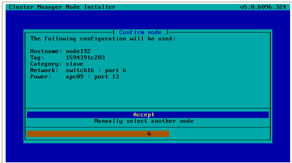
Figure 5.9: Scenarios: Configuration Found, Confirm Node Configuration
