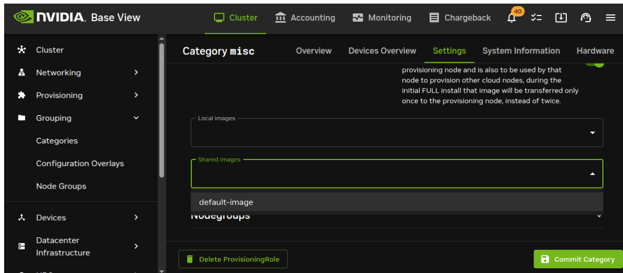
Figure 5.6: Base View: Configuring A provisioning Role
