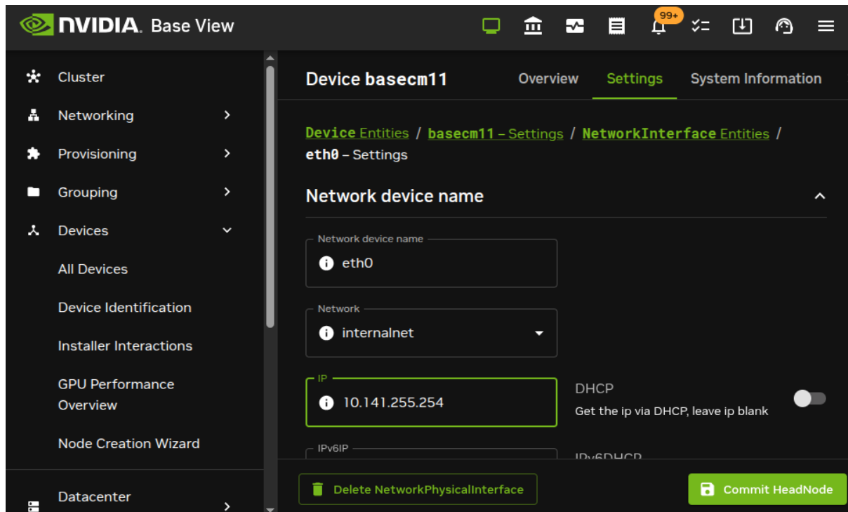
Figure 3.8: Setting The IP Address On A Head Node In Base View
