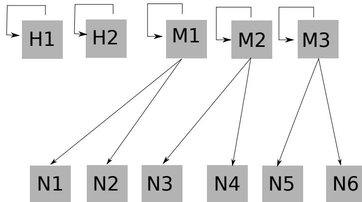
Figure 10.28: Monitoring Sampling Flow For Offloaded Monitoring With Dedicated Monitoring Nodes
