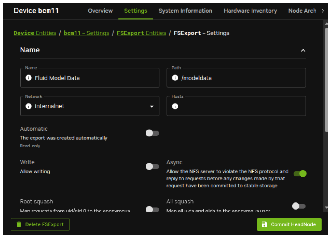
Figure 3.20: Setting up an NFS export using Base View
