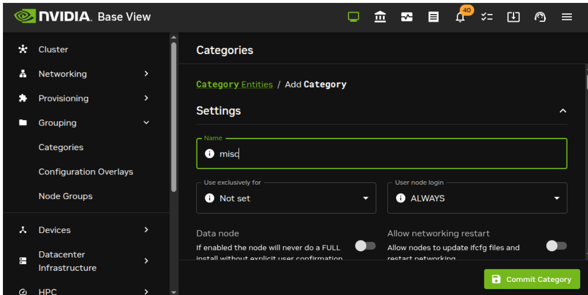
Figure 5.3: Base View: Adding A misc Category
