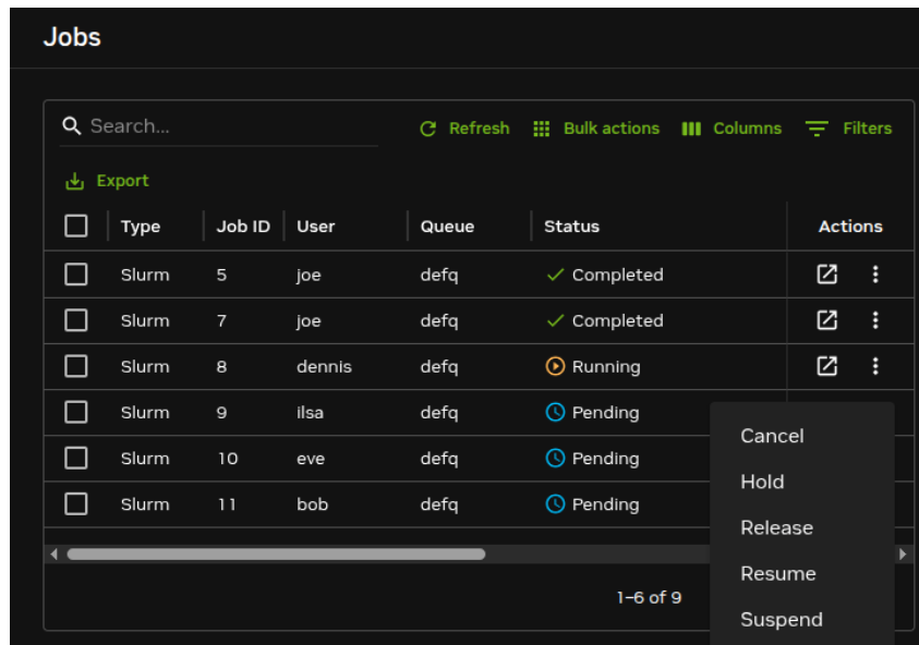
Figure 7.30: Workload manager job management window
