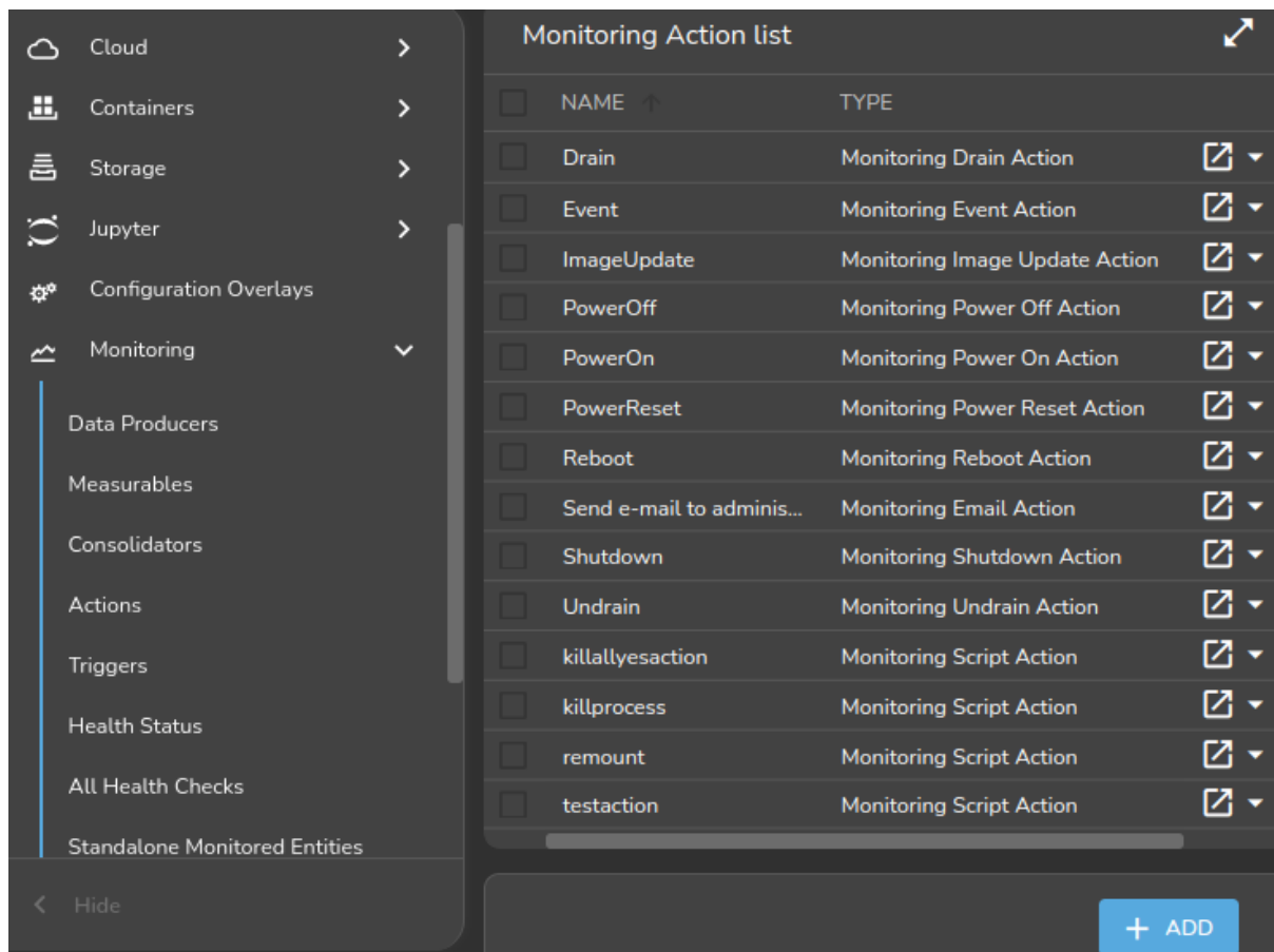
Figure 10.18: Base View Monitoring Configuration: Actions
