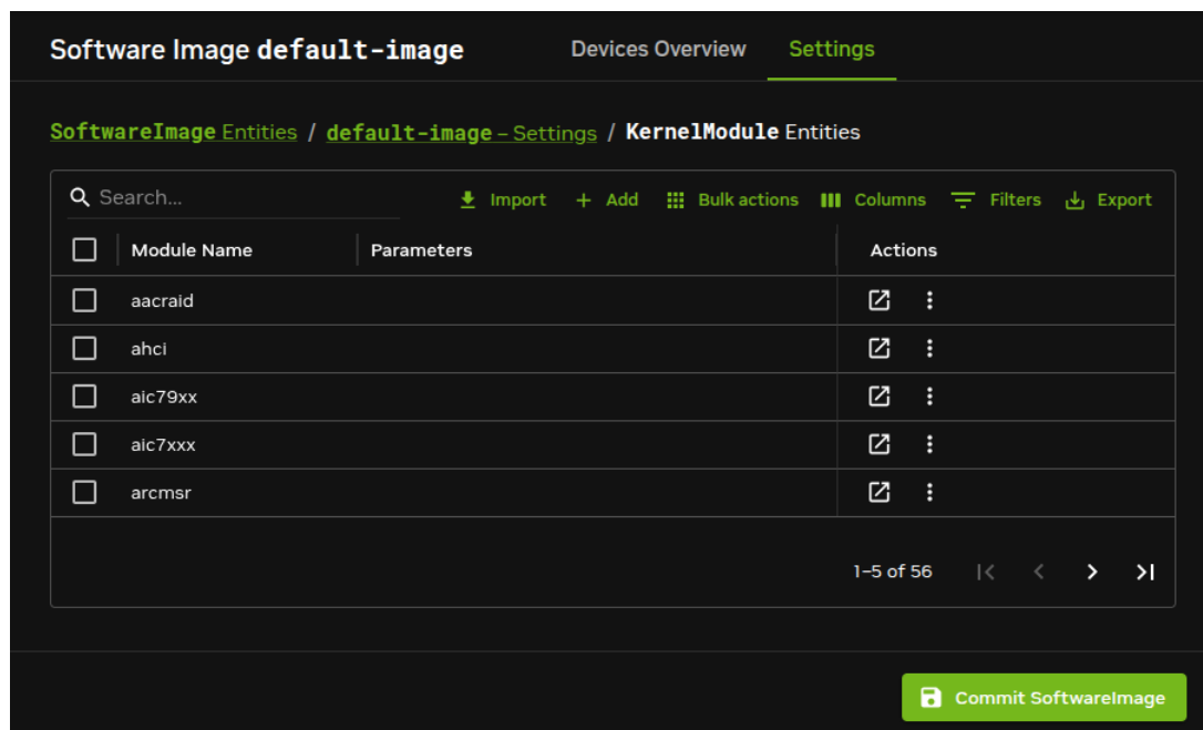
Figure 5.7: Base View: Selecting Kernel Modules For Software Images
