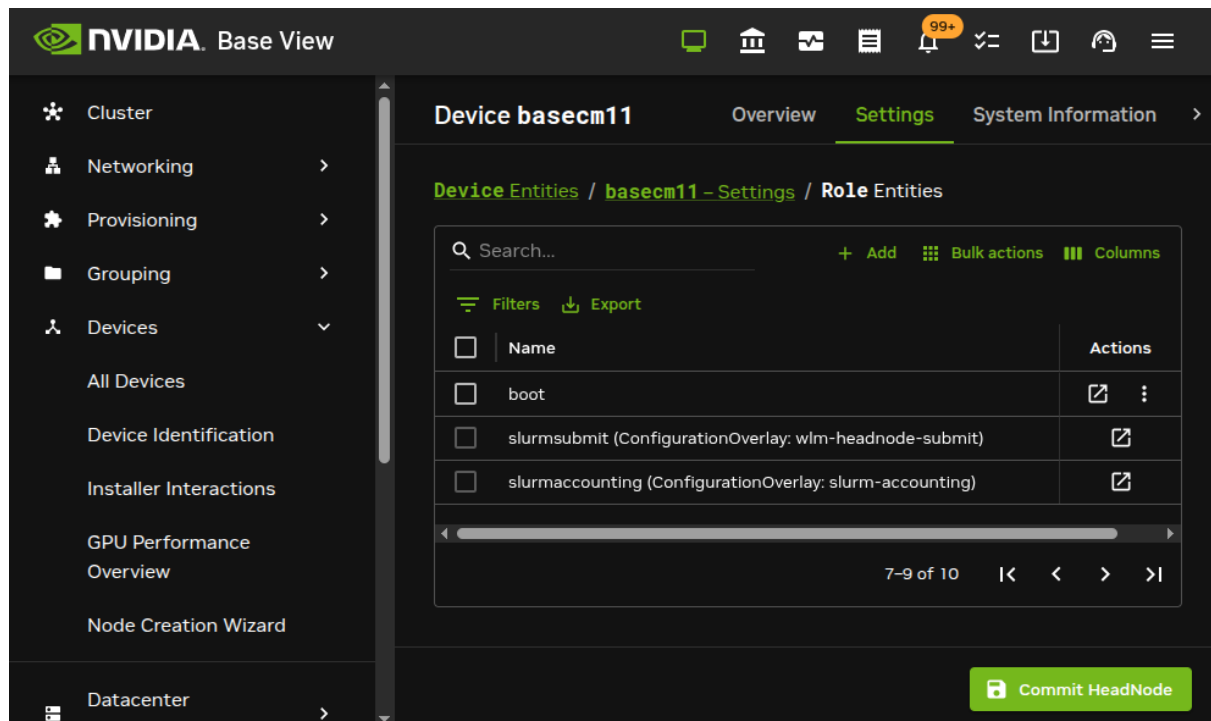
Figure 7.18: Roles seen on head node in Base View
