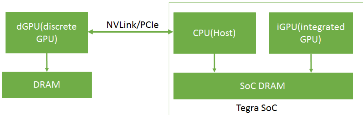
Figure 1. dGPU-connected Tegra Memory System
