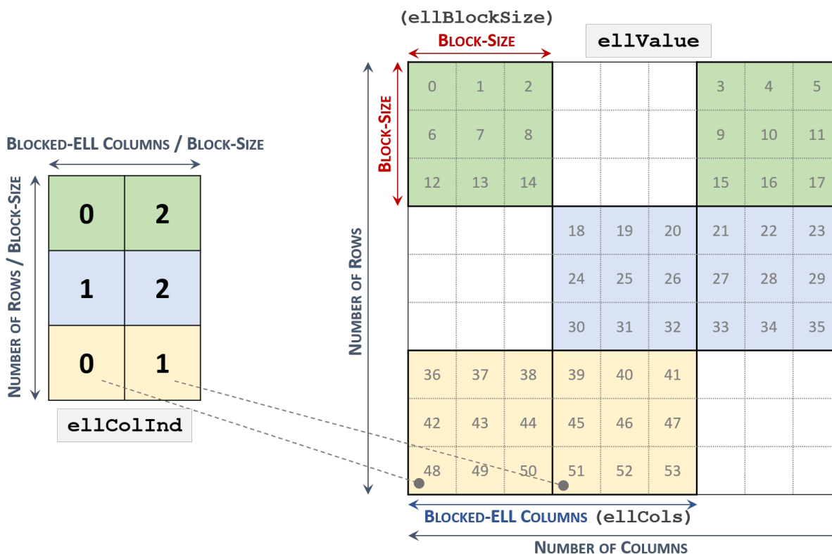
Figure 1. Blocked-ELL representation
