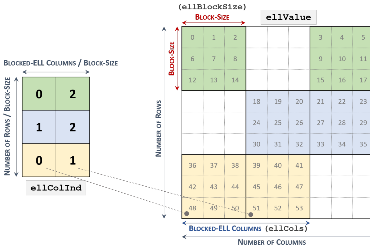
Figure 1. Blocked-ELL representation
