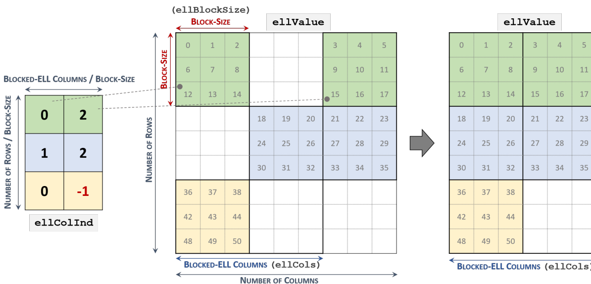
Figure 1. Blocked-ELL representation
