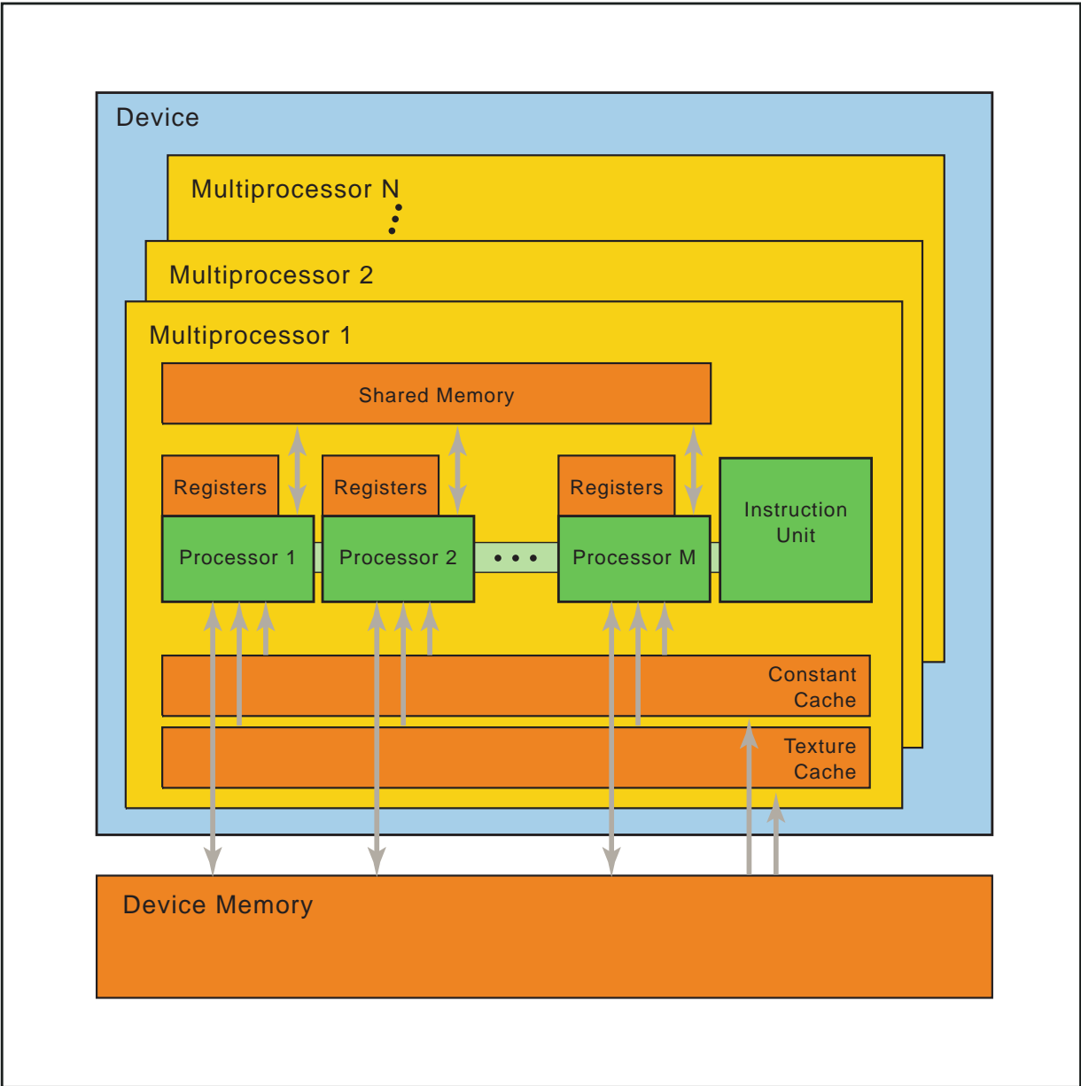
Figure 3. Hardware Model
