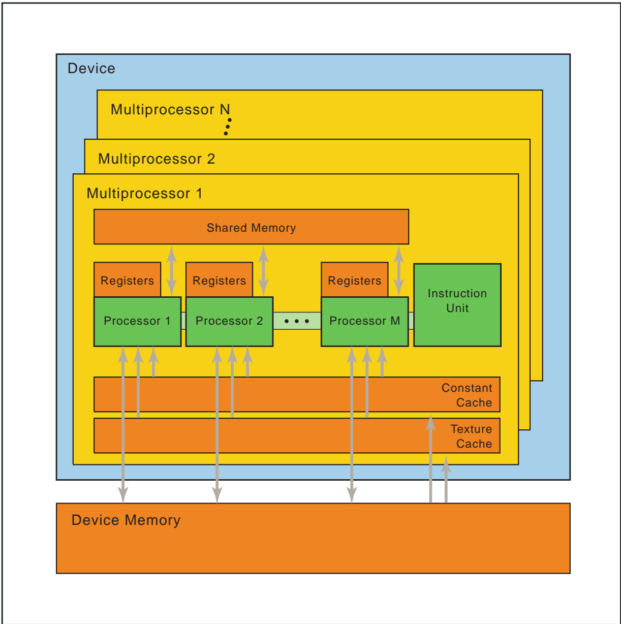
Figure 3. Hardware Model
