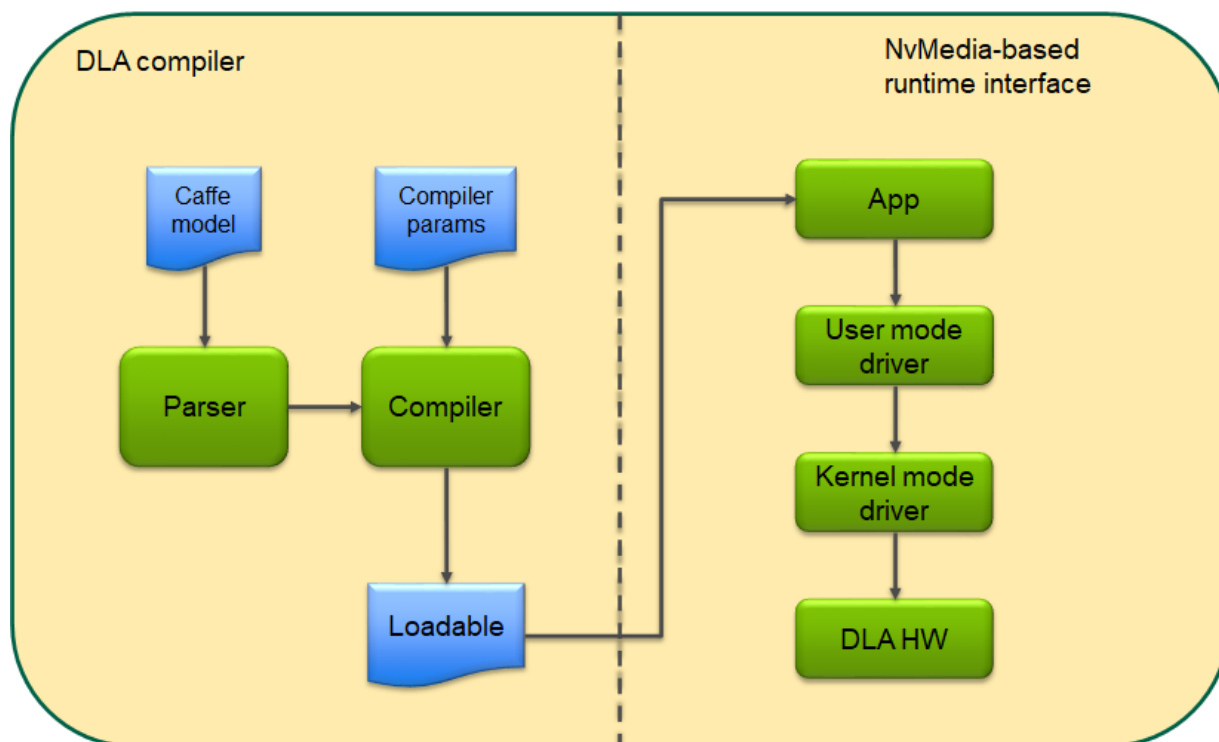
Figure 4. DLA SW stack
