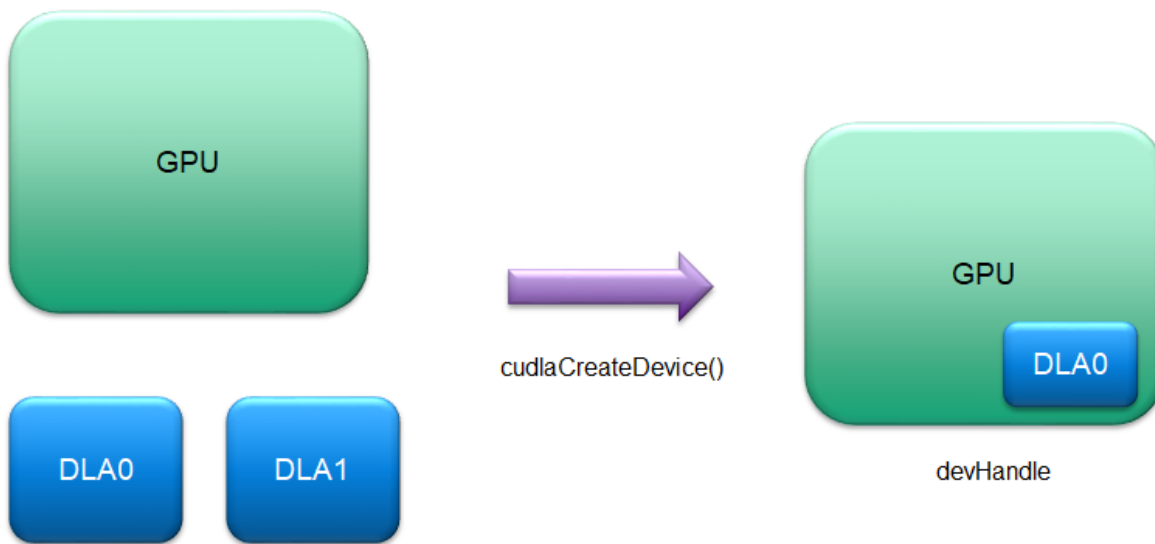
Figure 5. Device model
