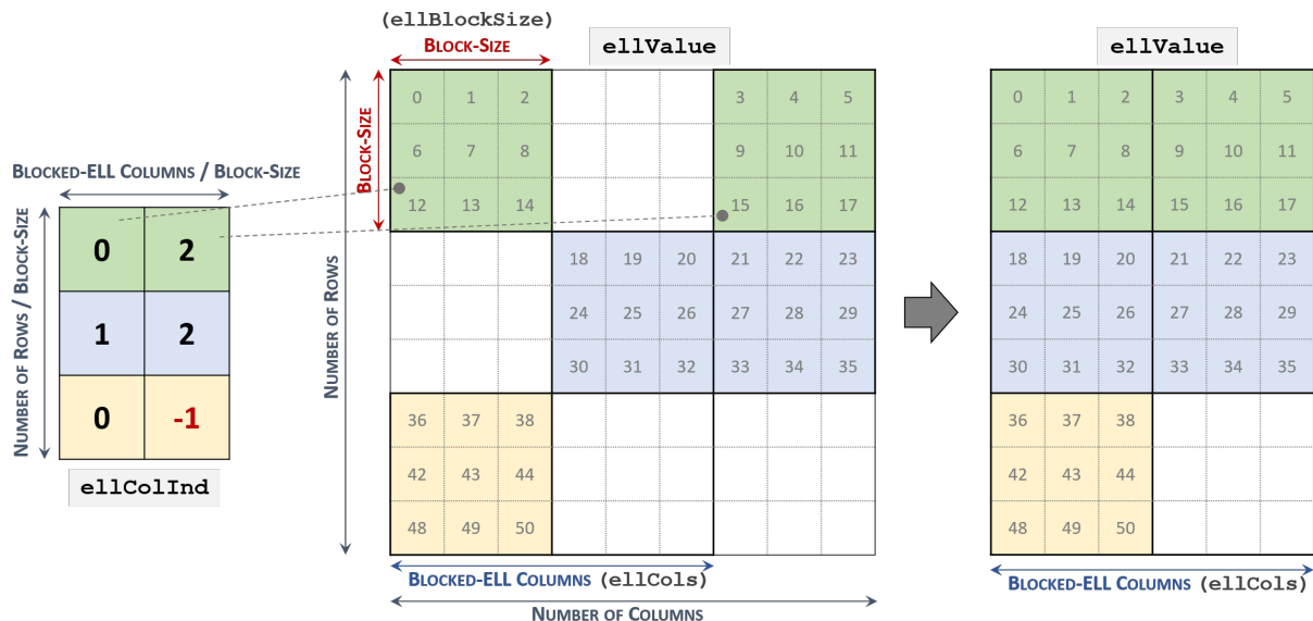
Figure 1. Blocked-ELL representation
