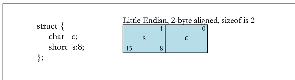
Figure 4. Storage Unit Sharing
