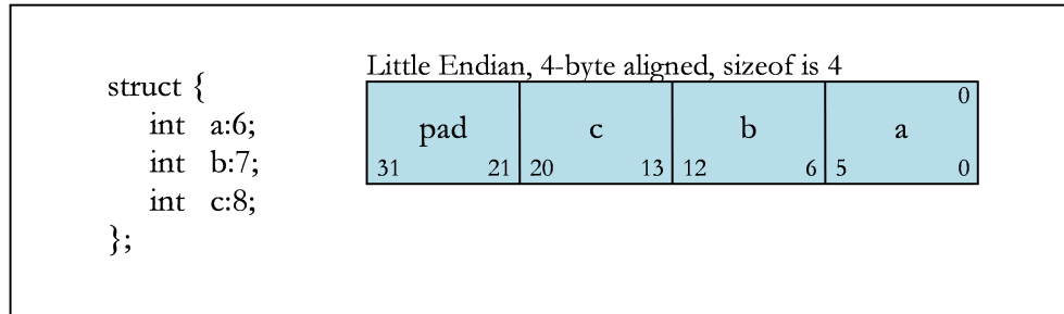
Figure 2. Bit-field Allocation
