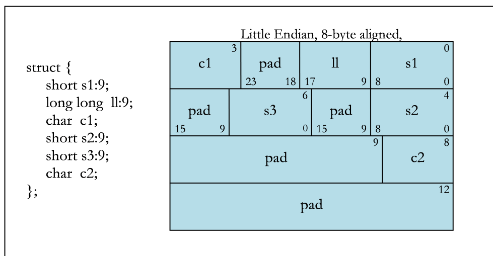
Figure 3. Boundary Alignment
