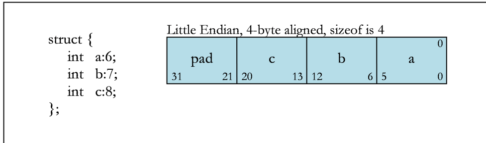
Figure 2. Bit-field Allocation
