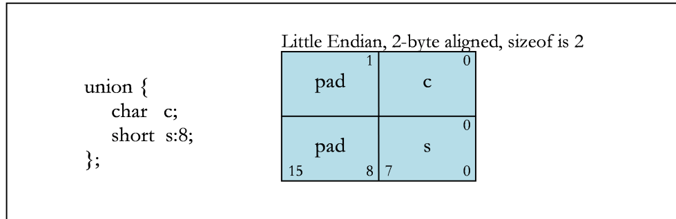
Figure 5. Union Allocation
