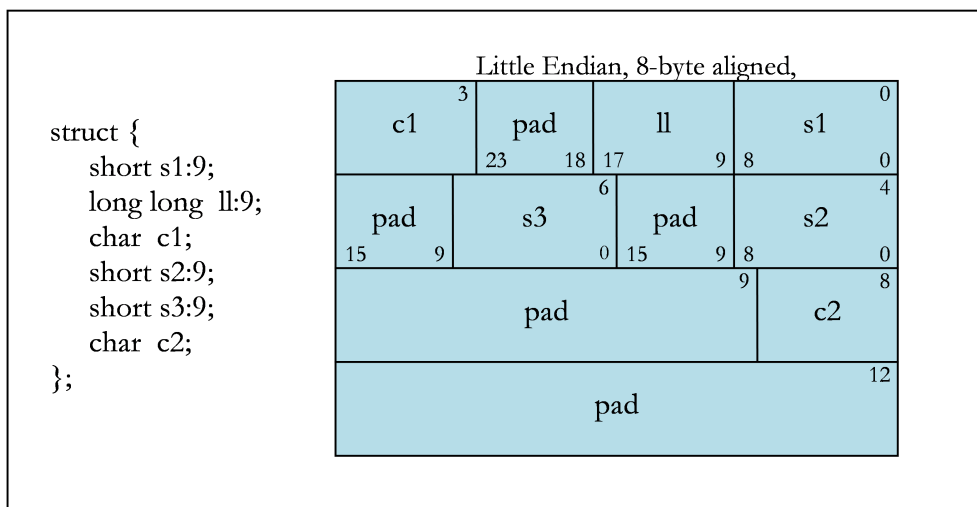
Figure 3. Boundary Alignment
