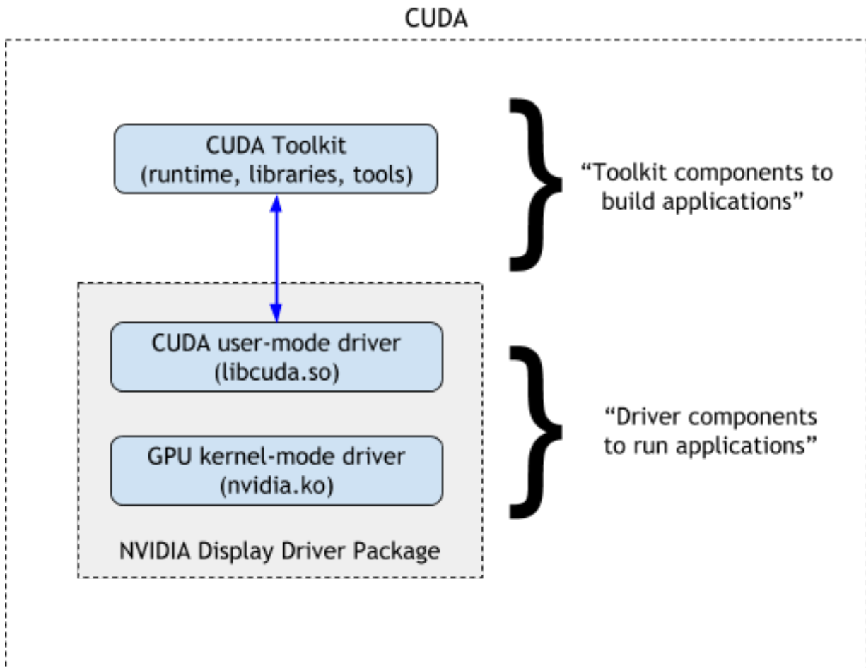
Figure 17. Components of CUDA
