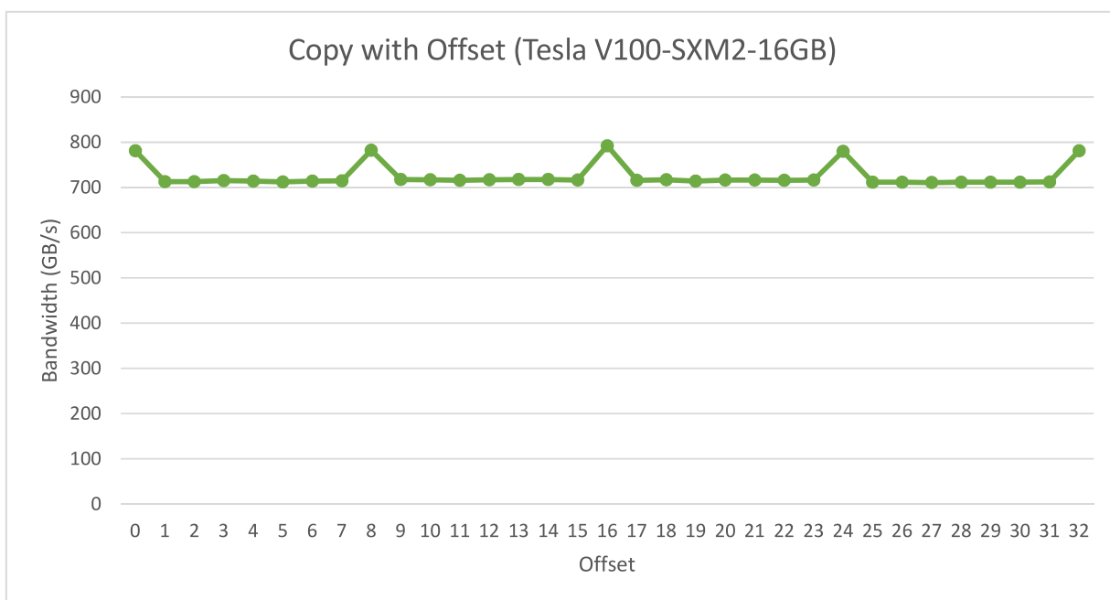
Figure 5. Performance of offsetCopy kernel
