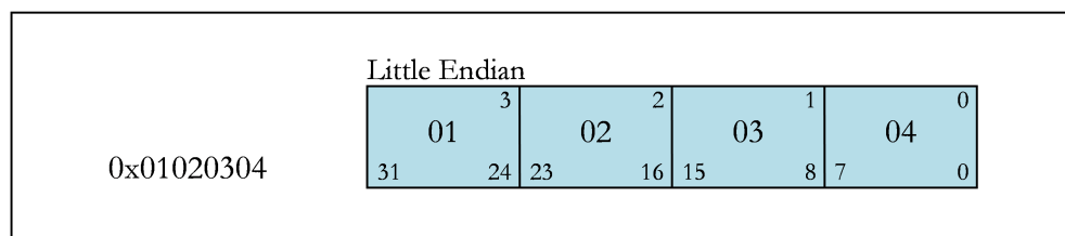
Figure 1. Bit Numbering
