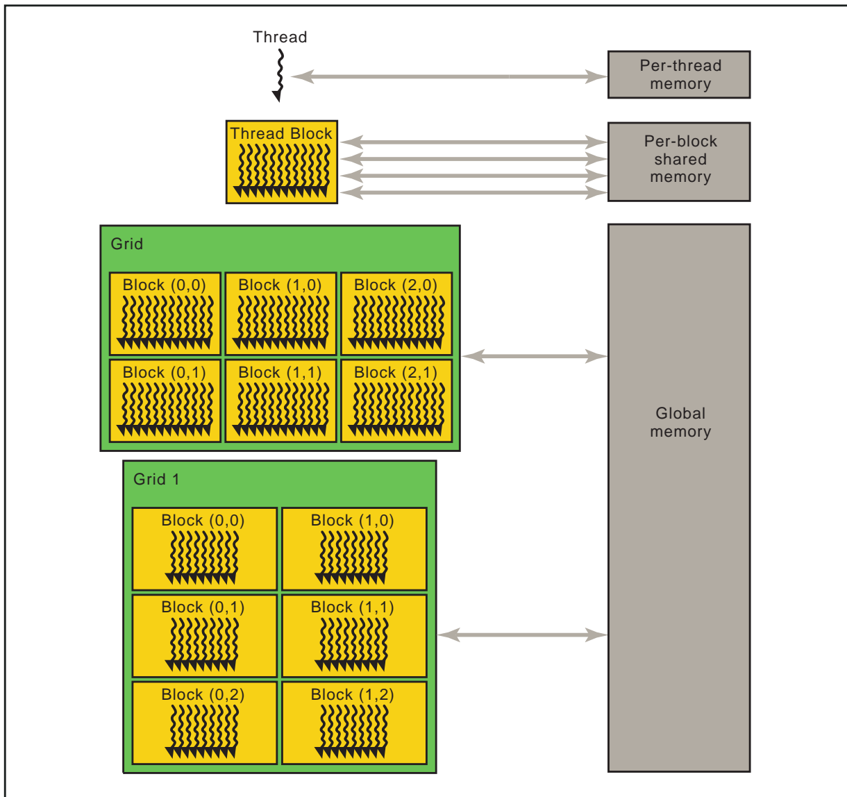
Figure 2. Memory Hierarchy
