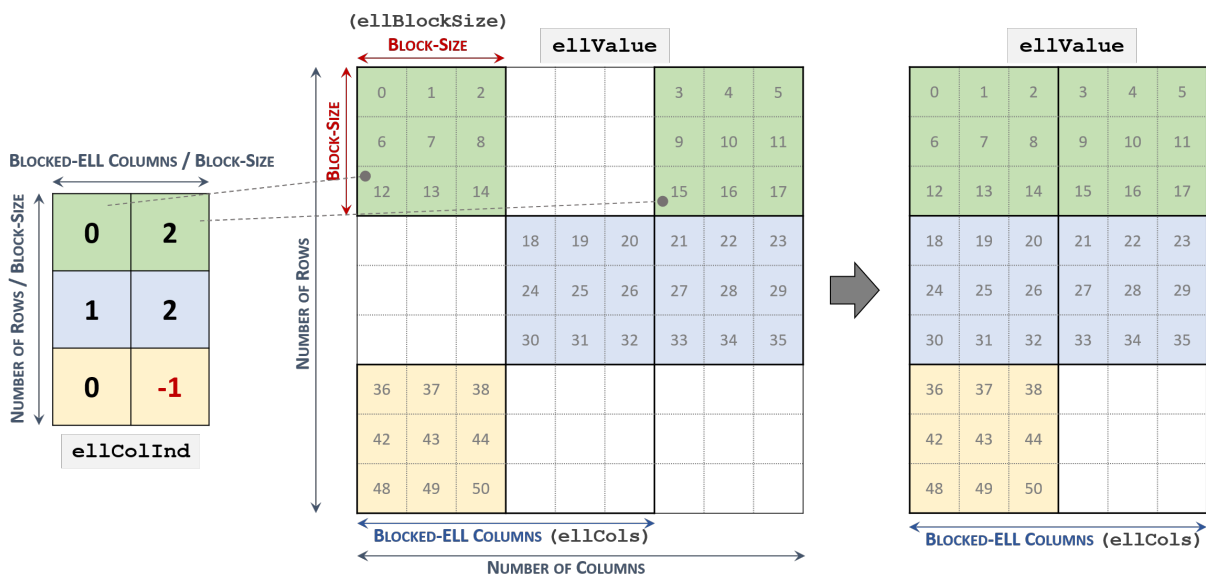
Figure 1. Blocked-ELL representation
