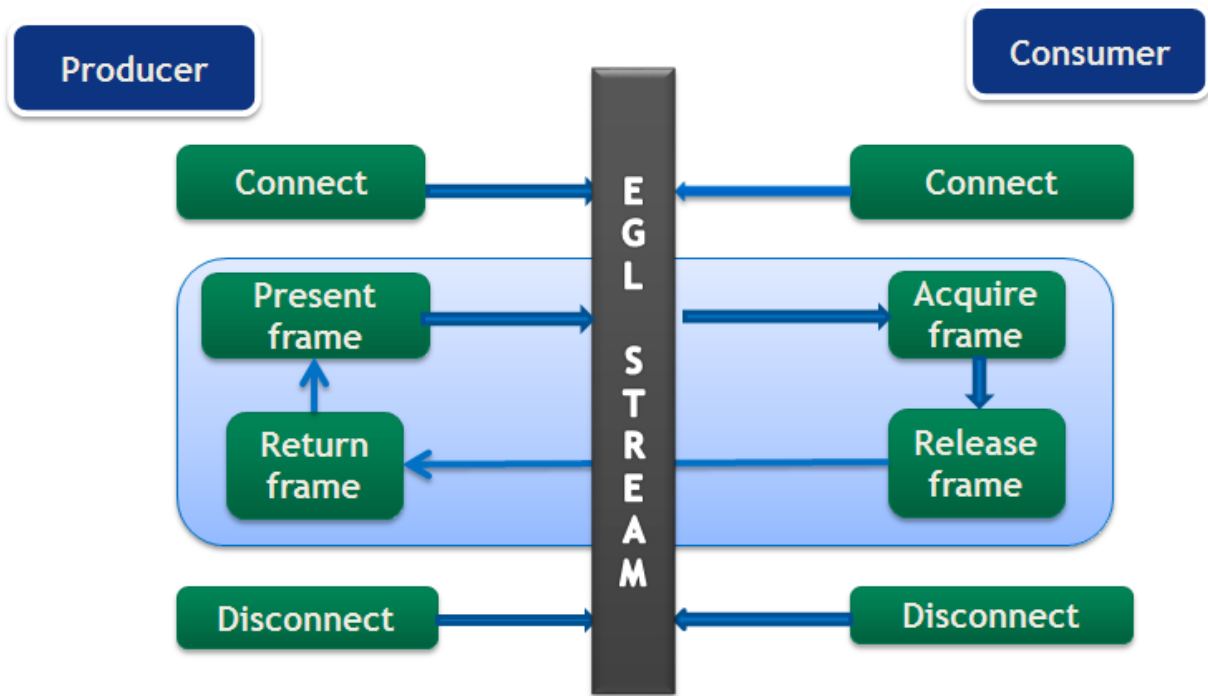
Figure 2. EGLStream Flow
