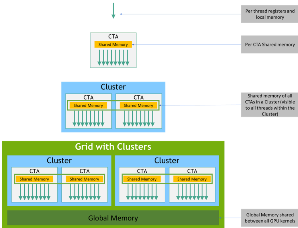
Figure 3. Memory Hierarchy
