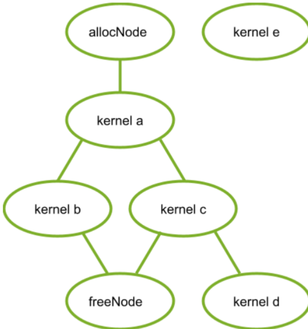
Figure 21. Kernel Nodes
