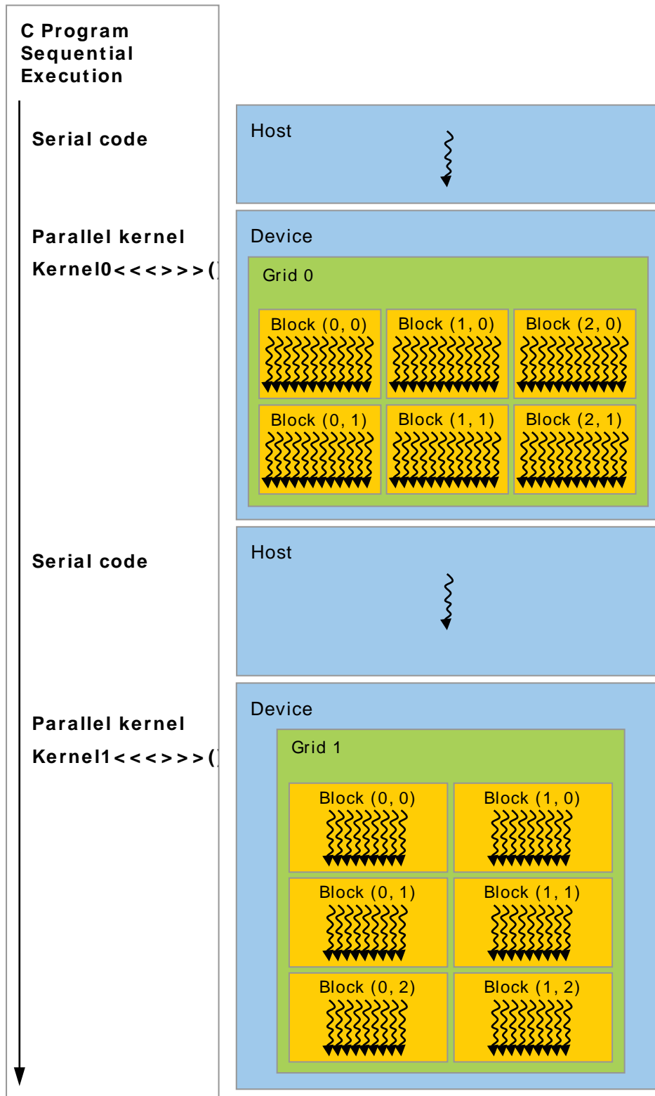
Figure 7. Heterogeneous Programming
