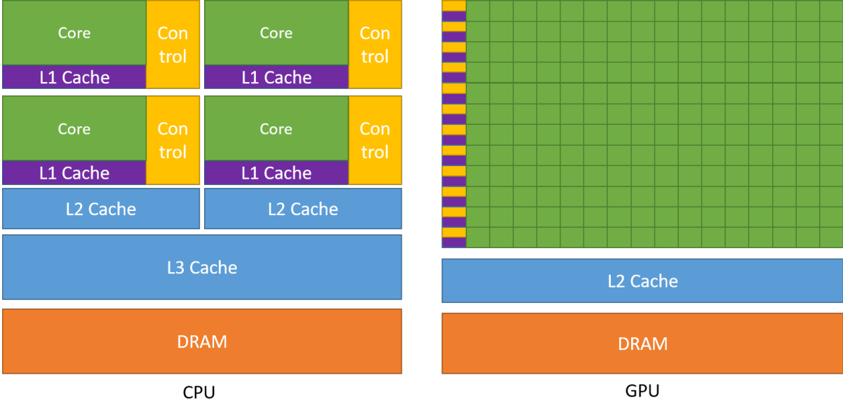
Fig. 1: The GPU Devotes More Transistors to Data Processing
