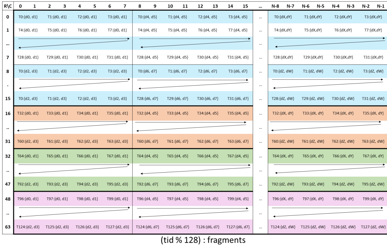
Figure 119: WGMMA .m64nNk16 register fragment layout for accumulator matrix D.
