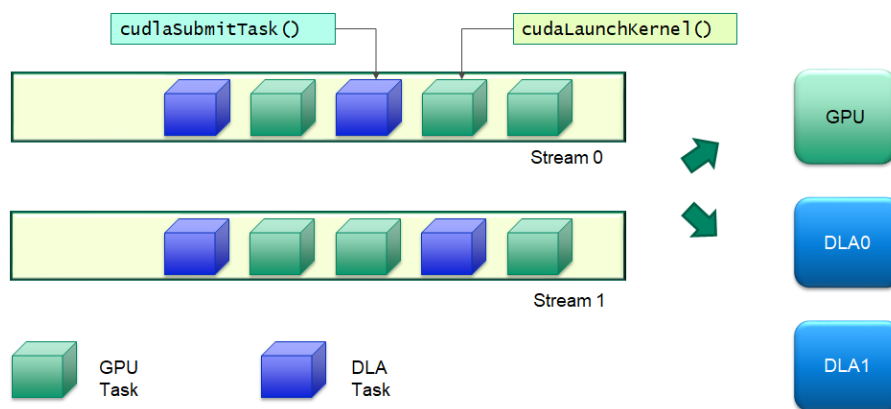
Fig. 5: cuDLA task execution model
