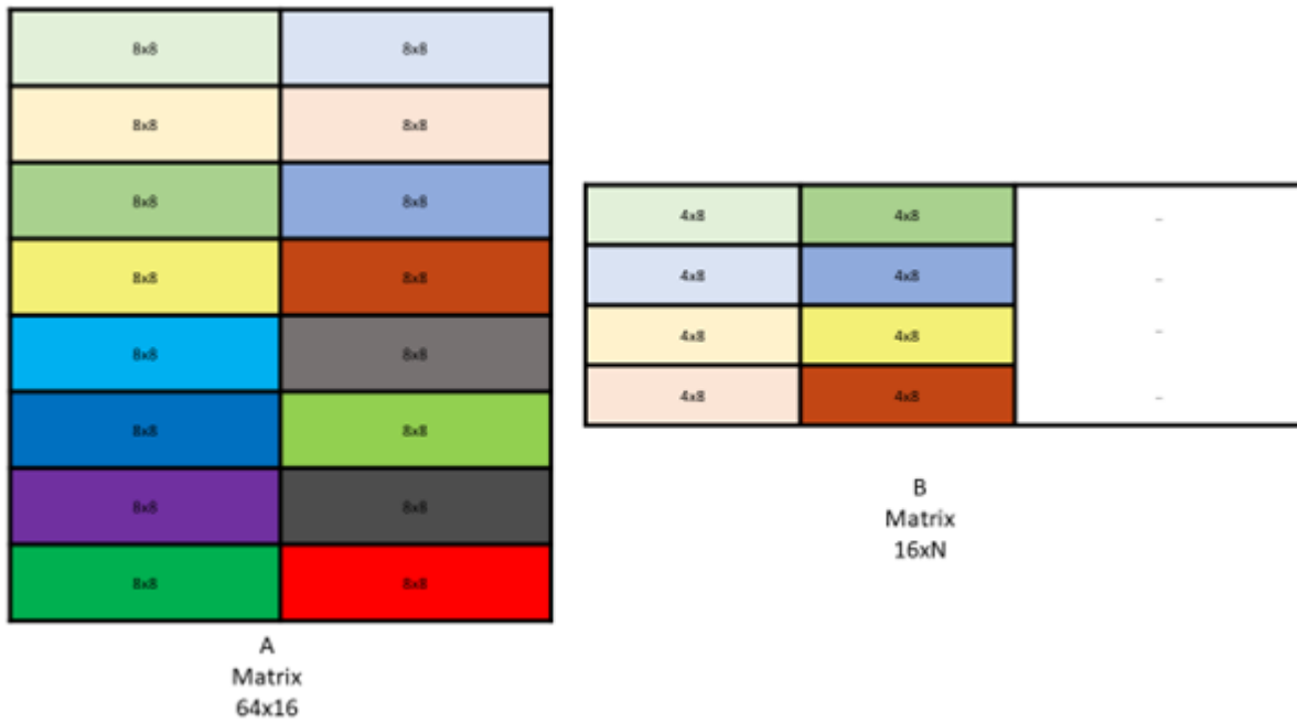
Figure 158: Sparse WGMMA .m64nNk16 core matrices for A and B
