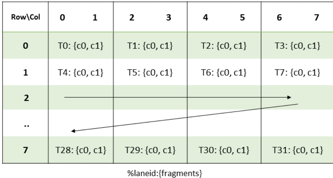
Figure 33: MMA .m8n8k16 fragment layout for accumulator matrix C/D with .s32 type
