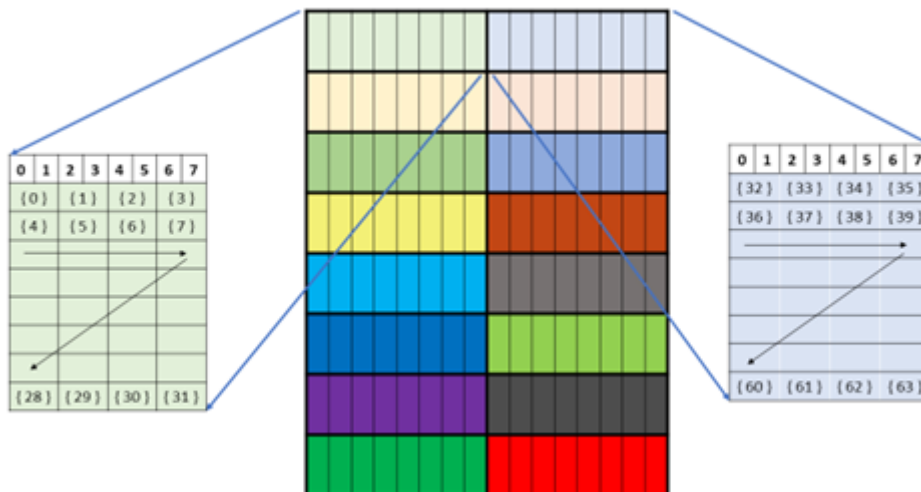
Figure 159: Sparse WGMMA .m64nNk16 core matrix layout for A
