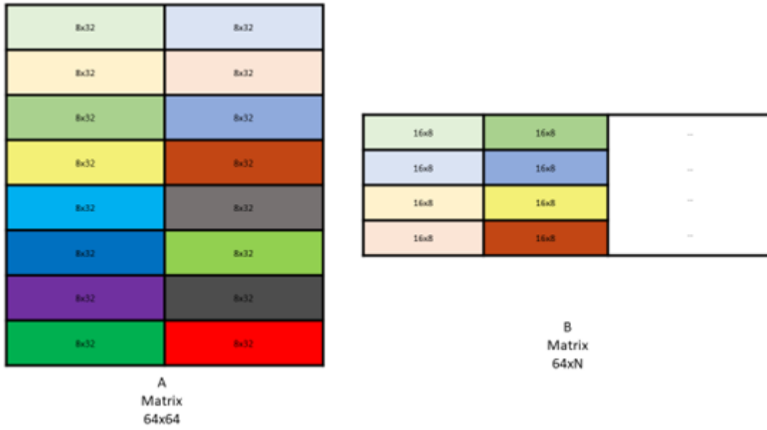
Figure 161: Sparse WGMMMA .m64nNk64 core matrices for A and B
