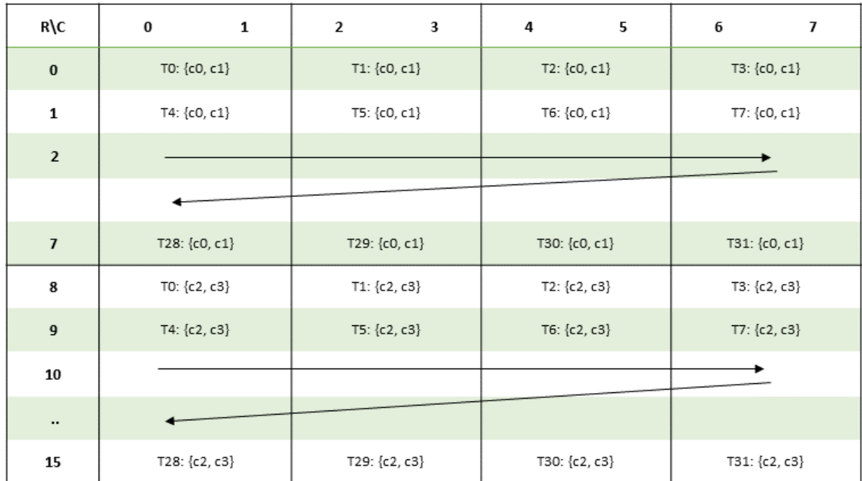
Figure 74: MMA .m16n8k128 fragment layout for accumulator matrix C/D with .s32 type.
