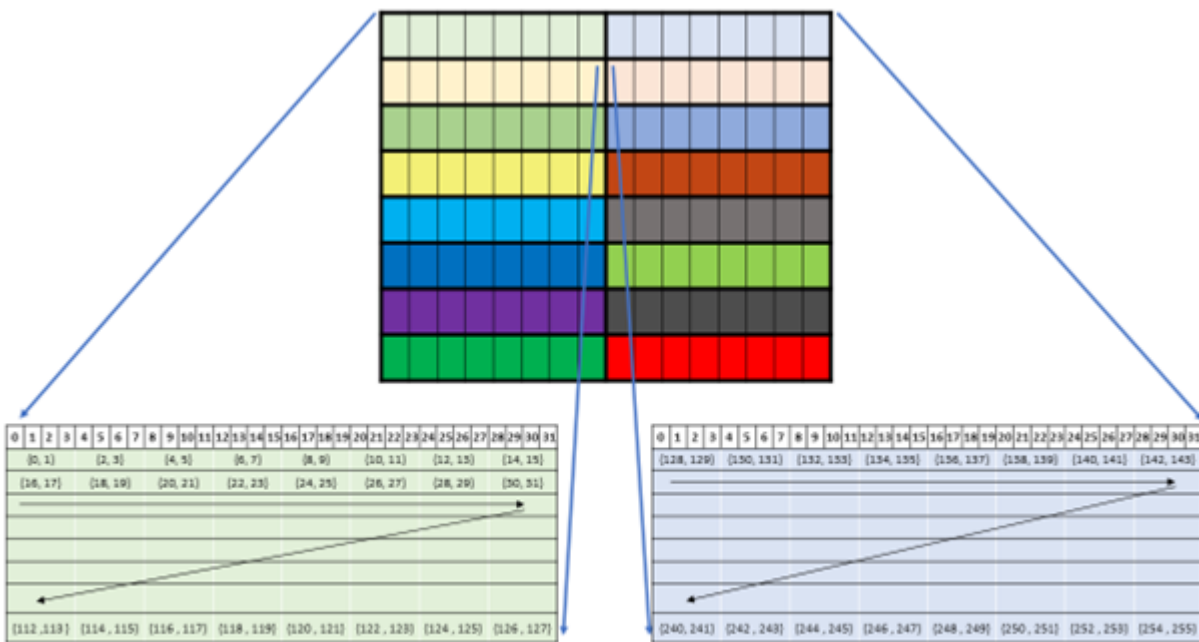
Figure 162: Sparse WGMMMA .m64nNk64 core matrix layout for A
