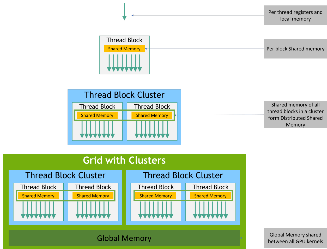
Fig. 3: Memory Hierarchy
