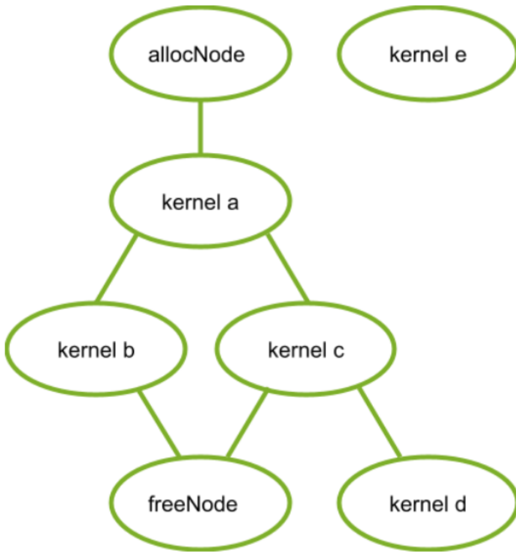
Fig. 1: Kernel Nodes
