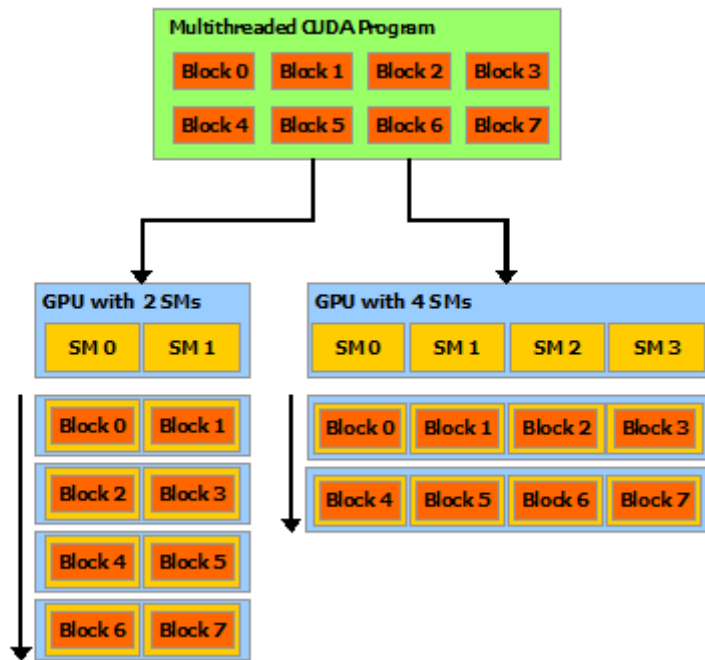
Fig. 1: Automatic Scalability
