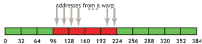
Fig. 3: Coalesced access
