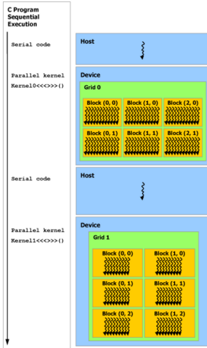
Figure 7: Heterogeneous Programming
