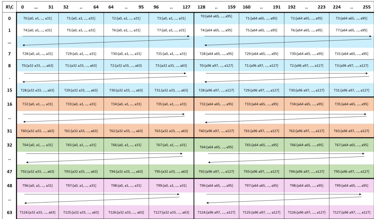
Figure 124: WGMMA .m64nNk256 register fragment layout for matrix A.
