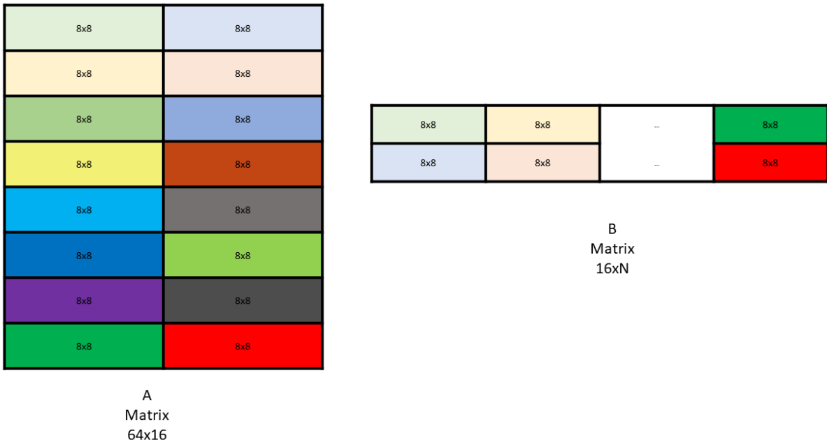
Figure 126: WGMMA .m64nNk16 core matrices for A and B
