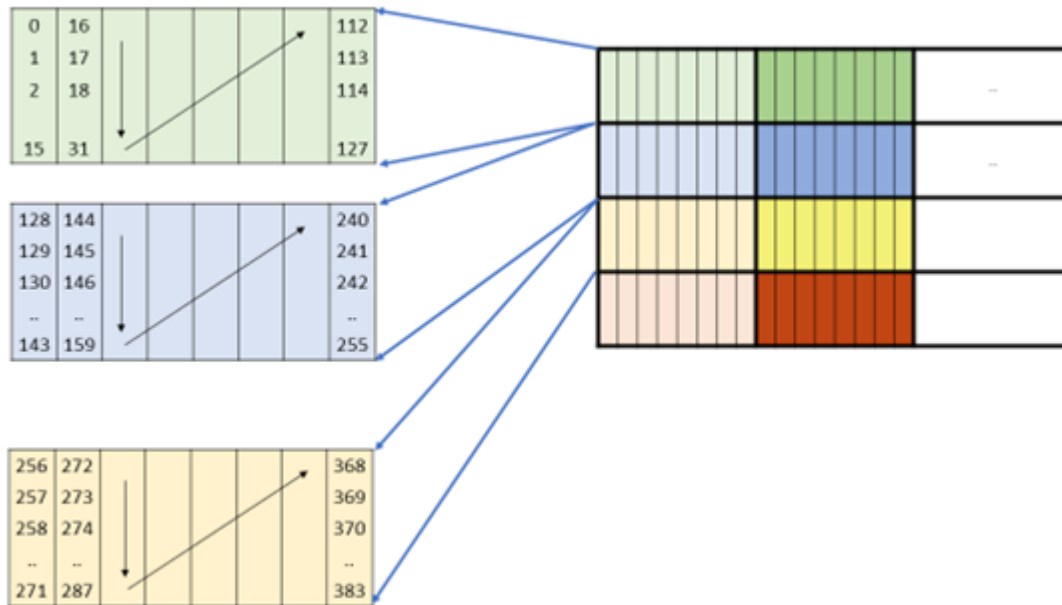
Figure 163: Sparse WGMMA .m64nNk64 core matrix layout for B
