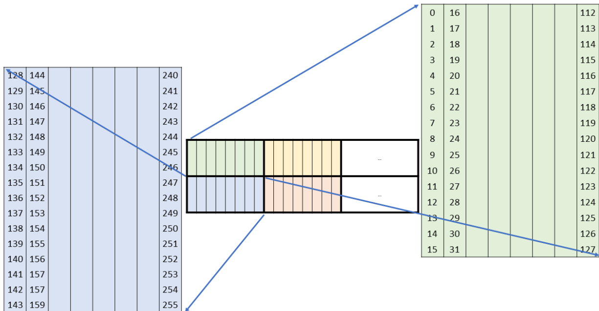
Figure 134: WGMMA .m64nNk32 core matrix layout for B
