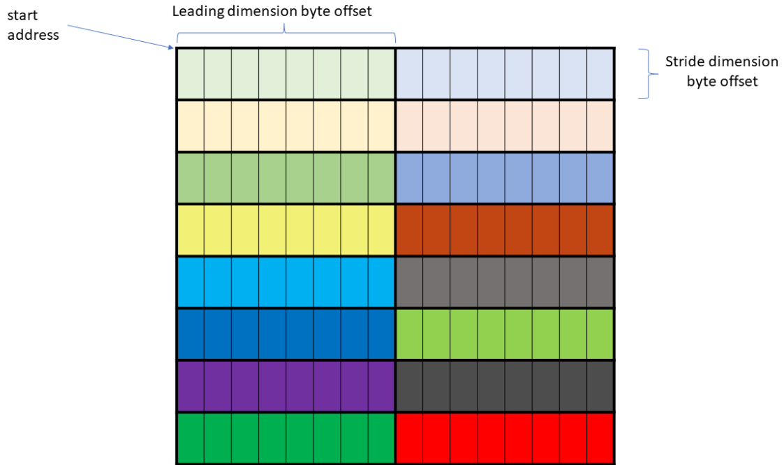
Figure 138: WGMMA stride and leading dimension byte offset for matrix A
