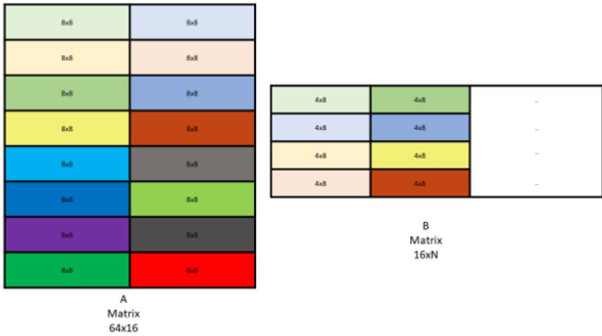
Figure 158: Sparse WGMMMA .m64nNk16 core matrices for A and B
