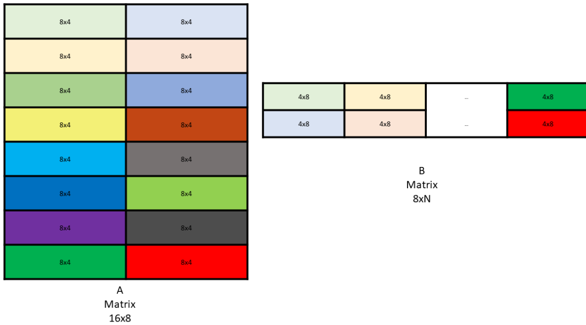
Figure 129: WGMMMA .m64nNk8 core matrices for A and B
