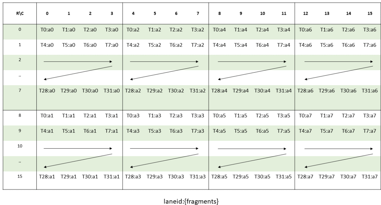
Figure 55: MMA .m16n8k16 fragment layout for matrix A with .f64 type.
