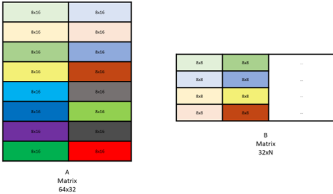
Figure 155: Sparse WGMMA .m64nNk32 core matrices for A and B
