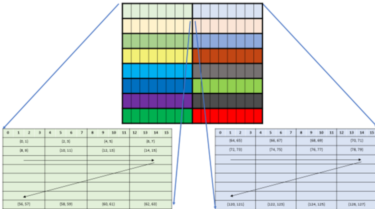
Figure 156: Sparse WGMMA .m64nNk32 core matrix layout for A
