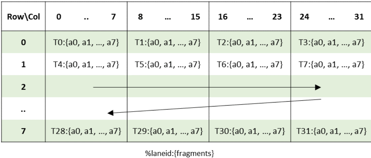
Figure 34: MMA .m8n8k32 fragment layout for matrix A with .u4/.s4 type
