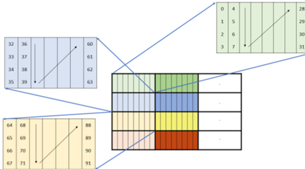
Figure 160: Sparse WGMMA .m64nNk16 core matrix layout for B
