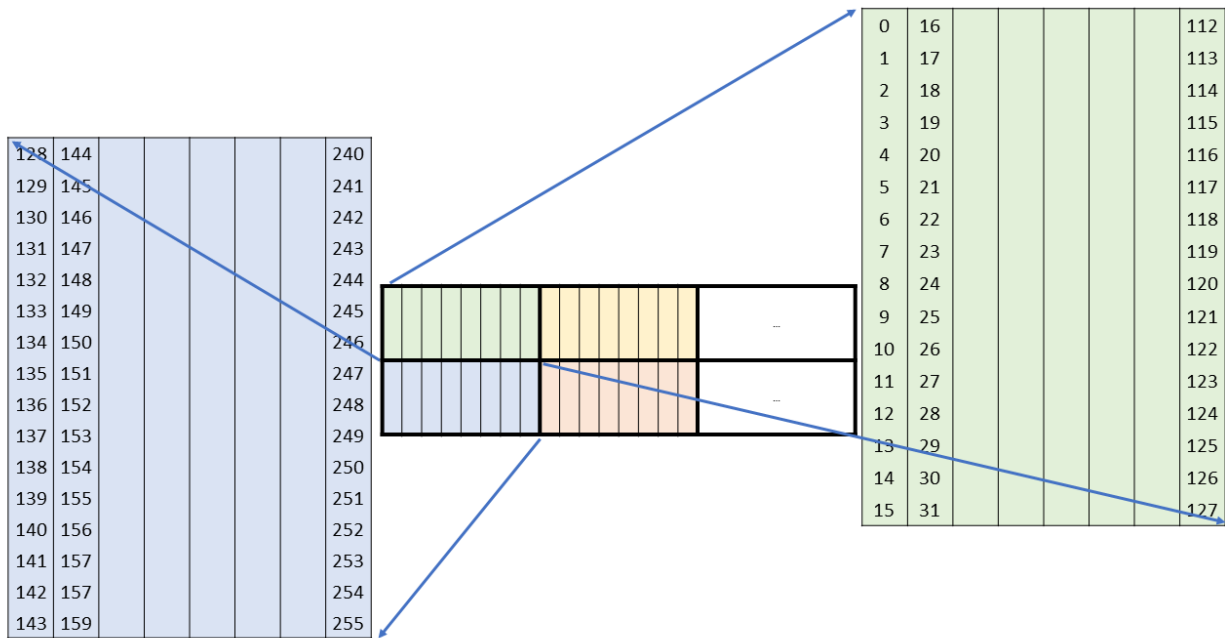
Figure 134: WGMMMA .m64nNk32 core matrix layout for B
