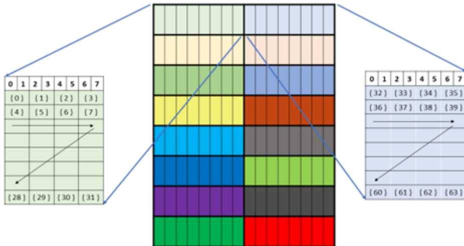
Figure 159: Sparse WGMMMA .m64nNk16 core matrix layout for A
