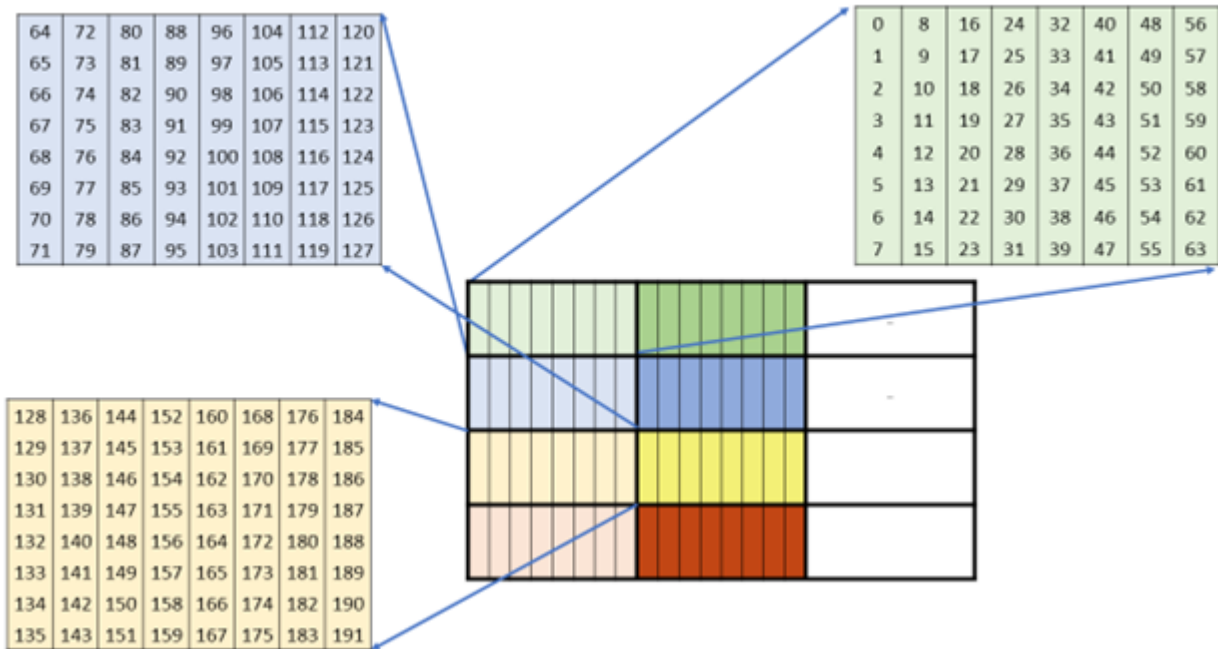
Figure 157: Sparse WGMMA .m64nNk32 core matrix layout for B
