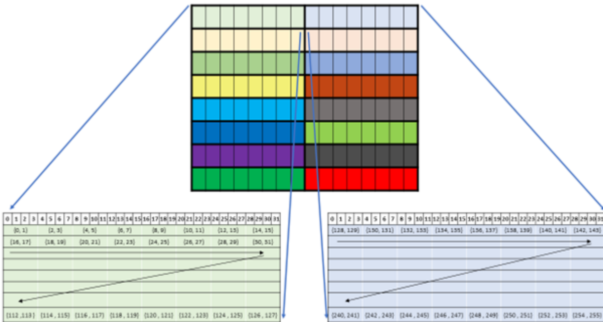
Figure 162: Sparse WGMMA .m64nNk64 core matrix layout for A
