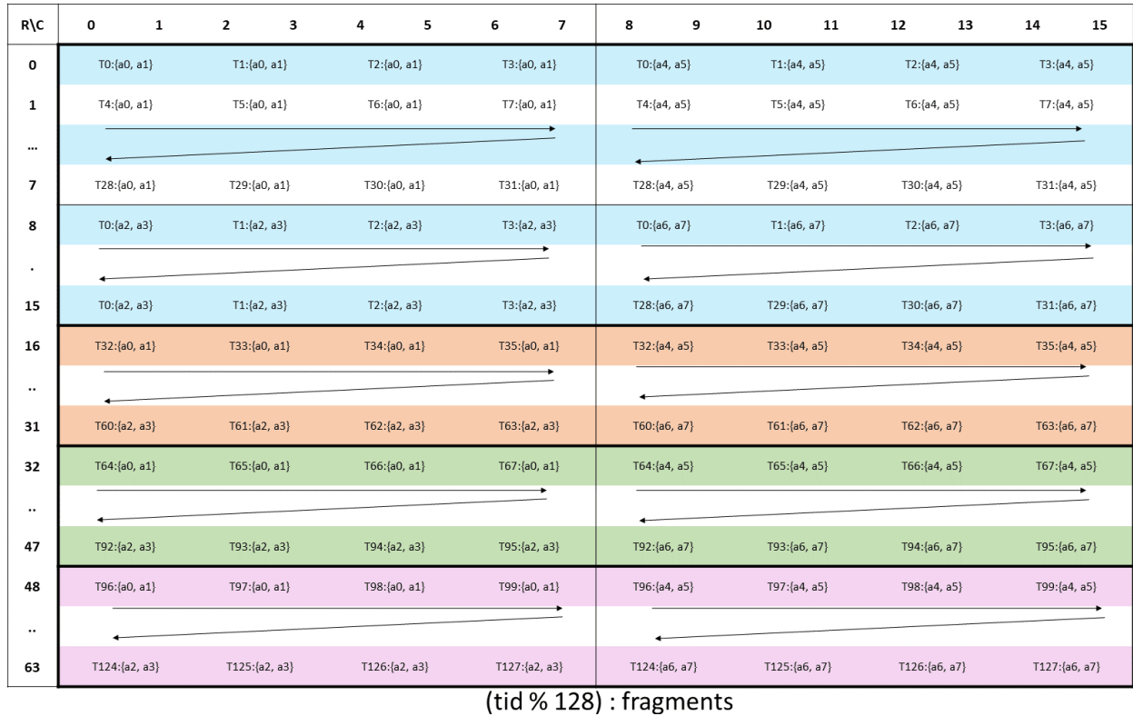
Figure 118: WGMMA .m64nNk16 register fragment layout for matrix A.
