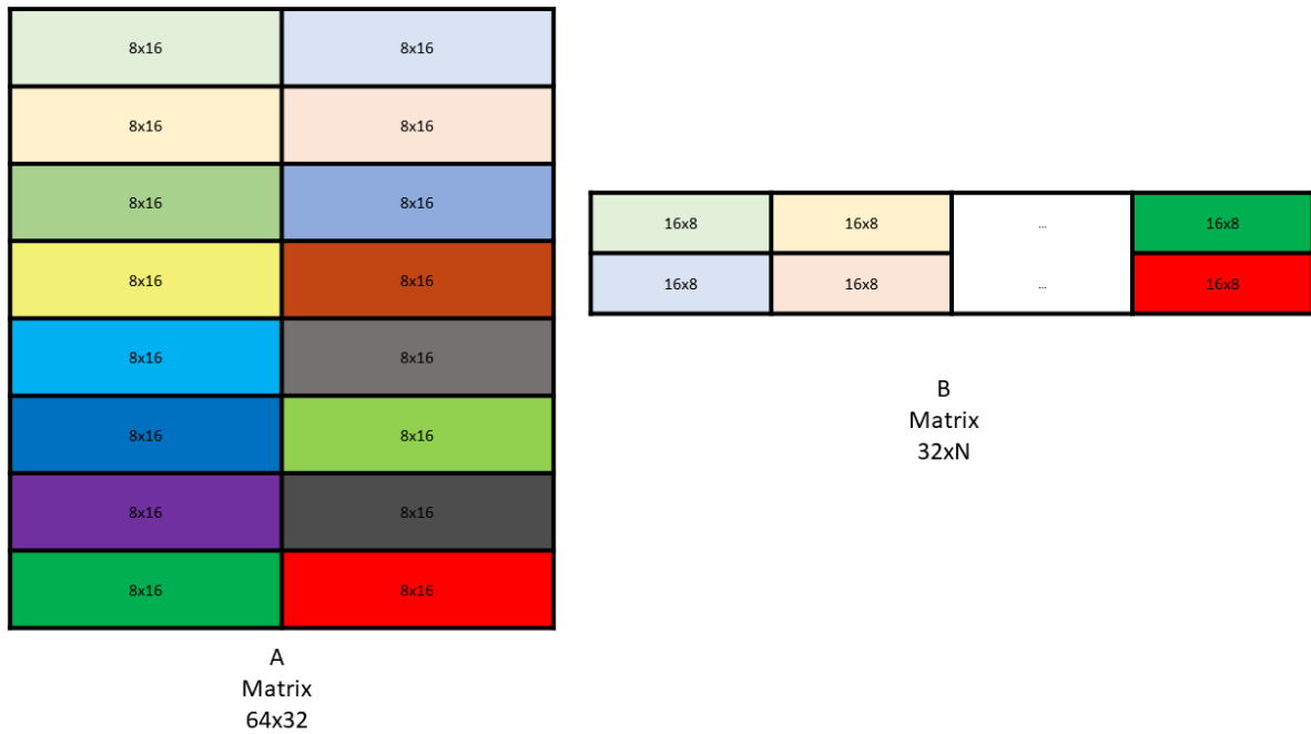
Figure 132: WGMMMA .m64nNk32 core matrices for A and B
