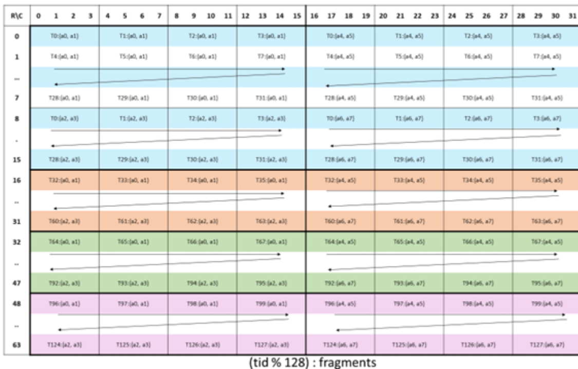
Figure 148: Sparse WGMMA .m64nNk32 fragment layout for matrix A with .f16/.bf16 type.
