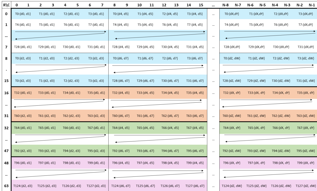
Figure 121: WGMMA .m64nNk8 register fragment layout for accumulator matrix D.
