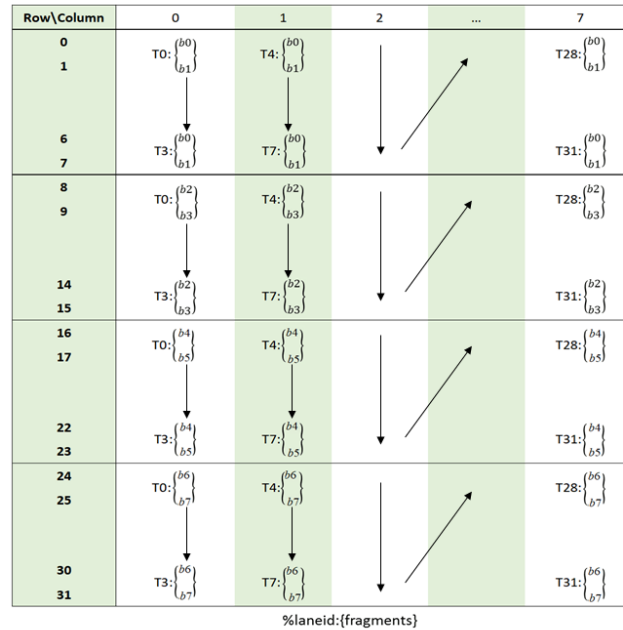
Figure 91: Sparse MMA .m16n8k32 fragment layout for matrix B with .f16/.bf16 type.
