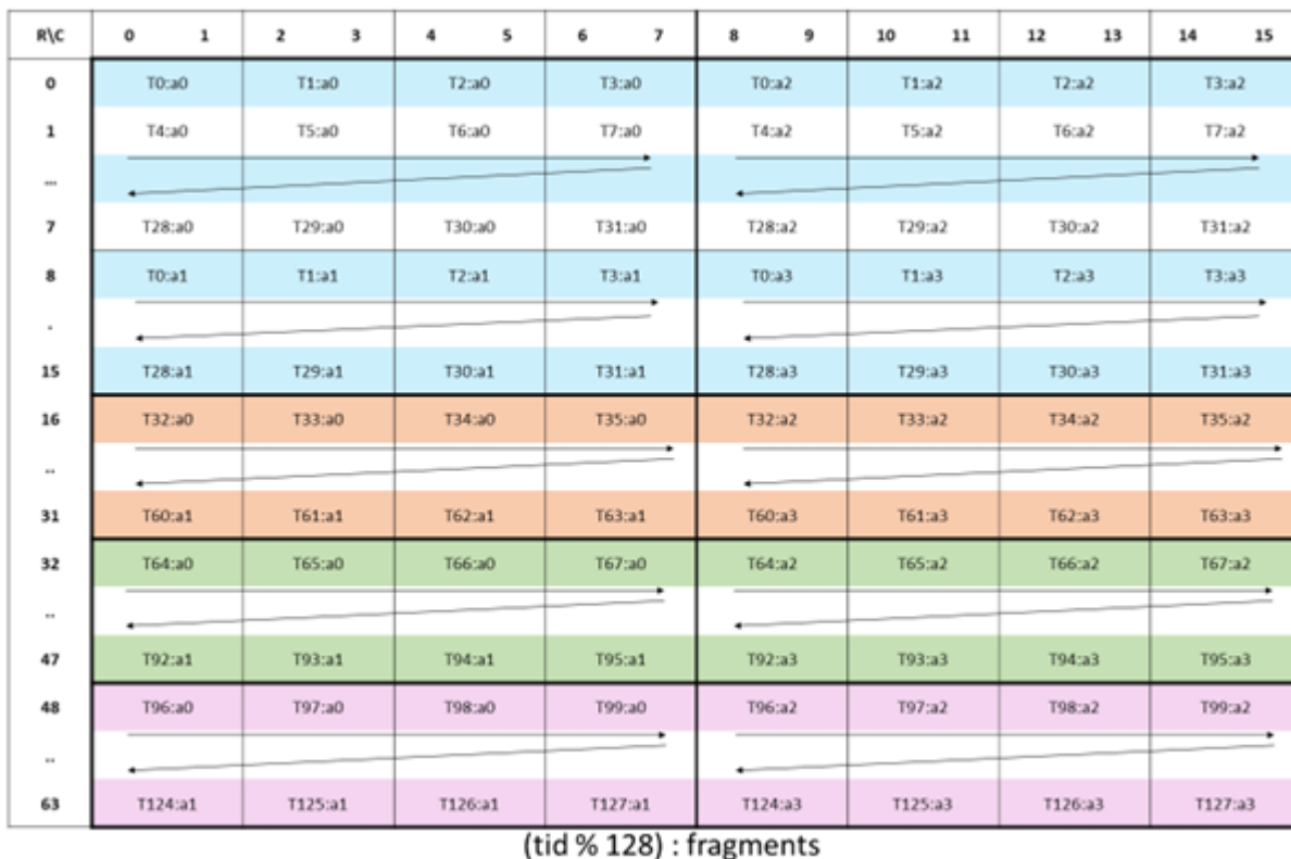
Figure 150: Sparse WGMMA .m64nNk16 fragment layout for matrix A with .tf32 type.
