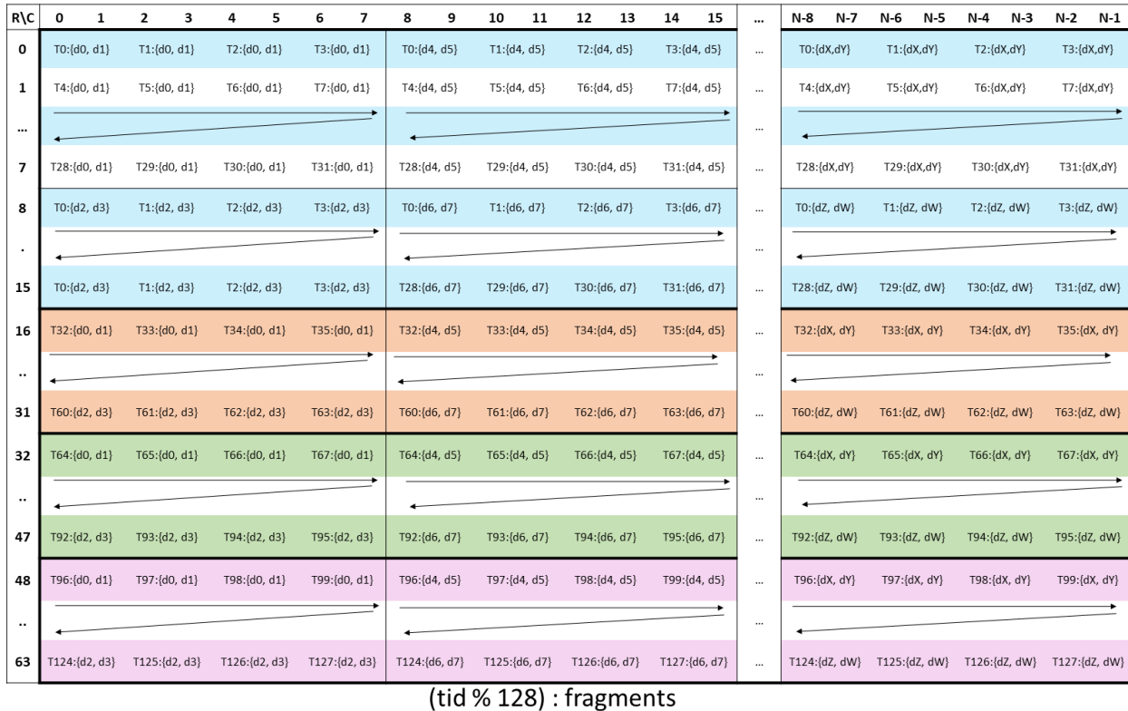
Figure 123: WGMMA .m64nNk32 register fragment layout for accumulator matrix D.
