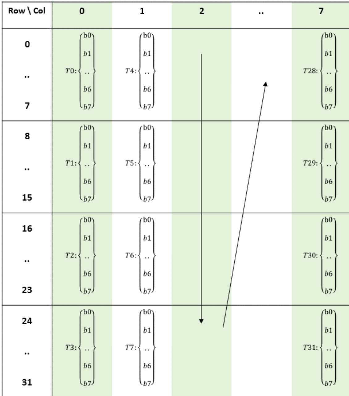
Figure 64: MMA .m16n8k32 fragment layout for matrix B with .u4 / .s4 type.
