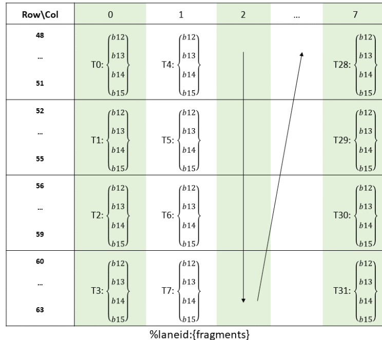
Figure 105: Sparse MMA .m16n8k64 fragment layout for rows 48–63 of matrix B with .u8/.s8 type.
