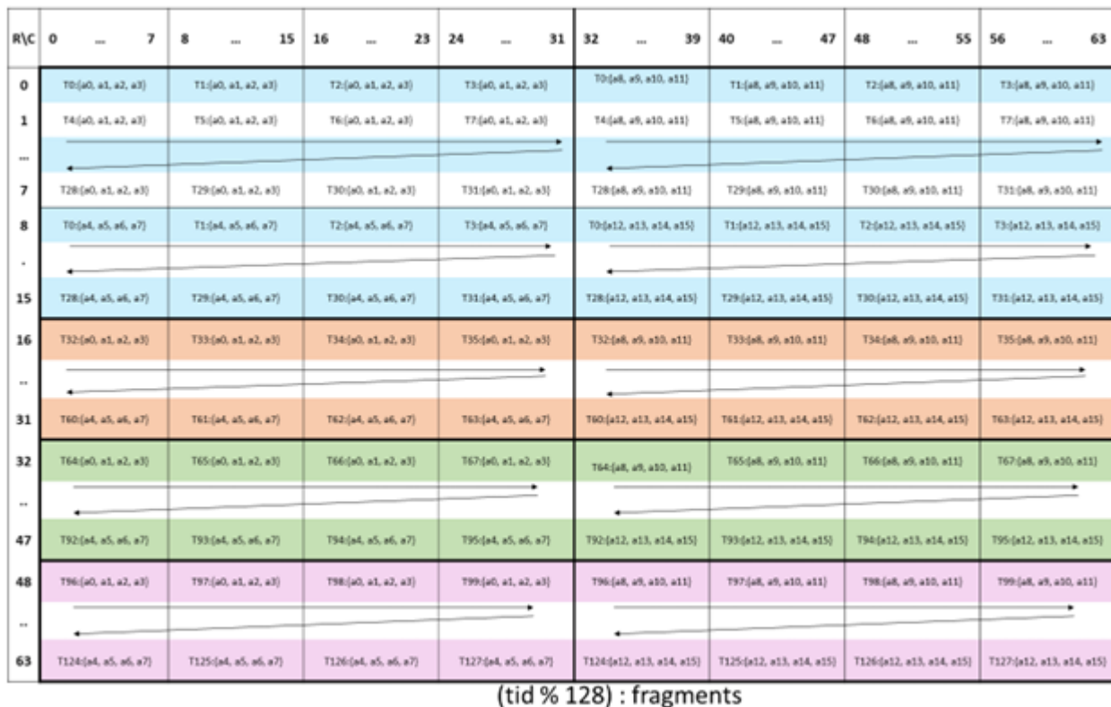
Figure 152: Sparse WGMMMA .m64nNk64 fragment layout for matrix A with .e4m3/ .e5m2/ .s8/ .u8 type.
