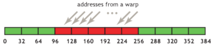
Fig. 4: Misaligned sequential addresses that fall within five 32-byte segments
