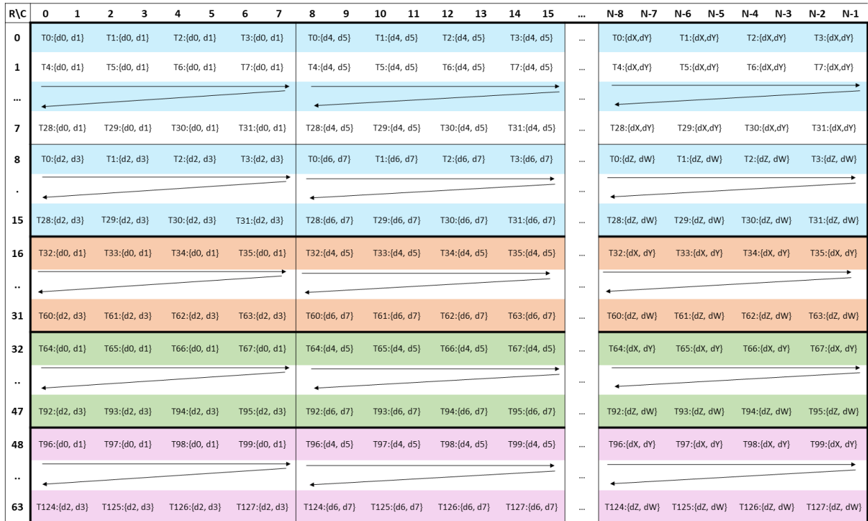
Figure 122: WGMMA .m64nNk8 register fragment layout for accumulator matrix D.
