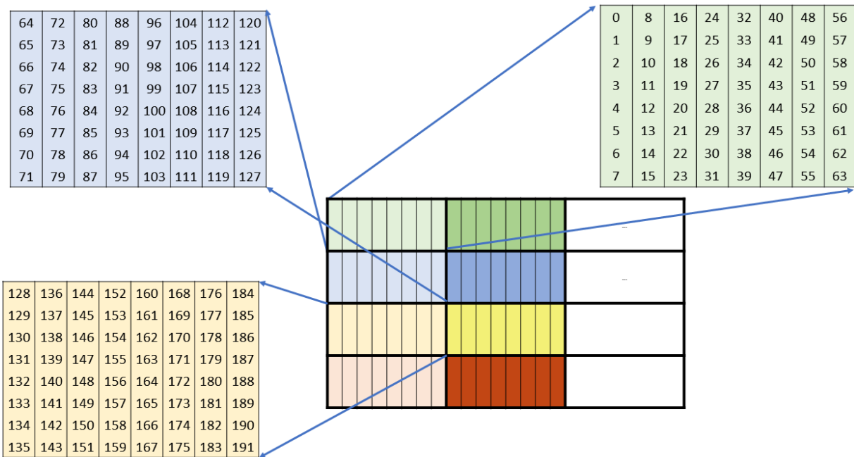
Figure 158: Sparse WGMMA .m64nNk32 core matrix layout for B
