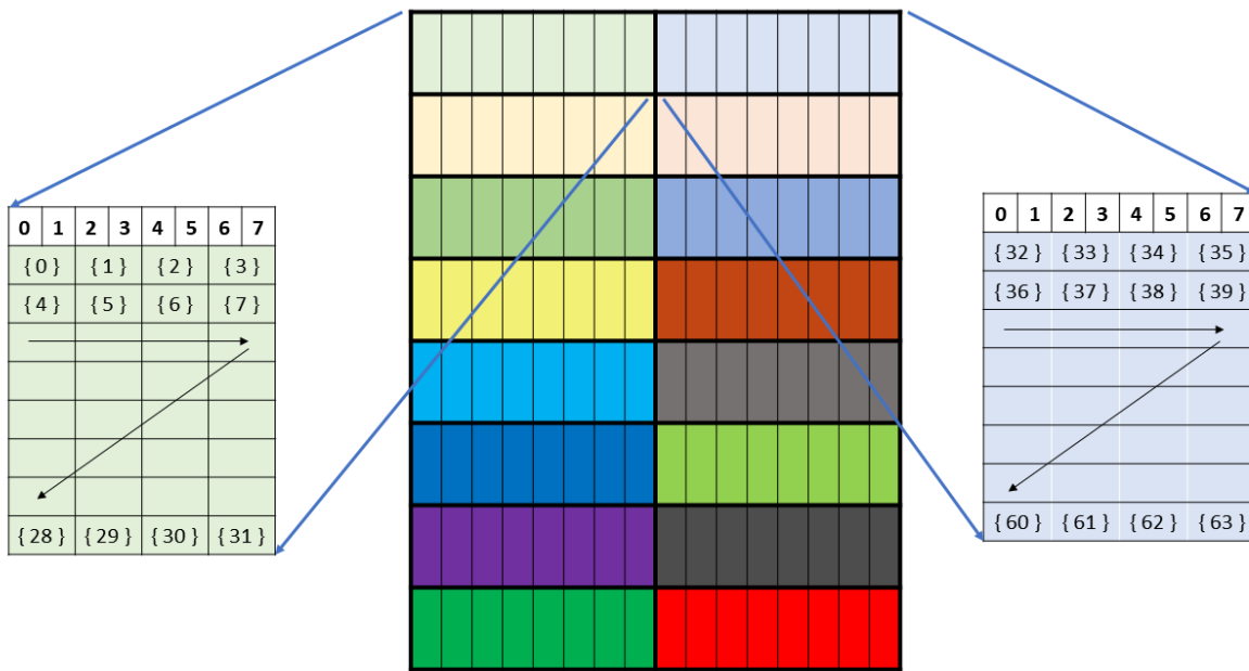
Figure 160: Sparse WGMMA .m64nNk16 core matrix layout for A
