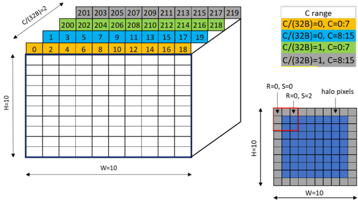
Figure 12: 32-byte swizzle mode example
