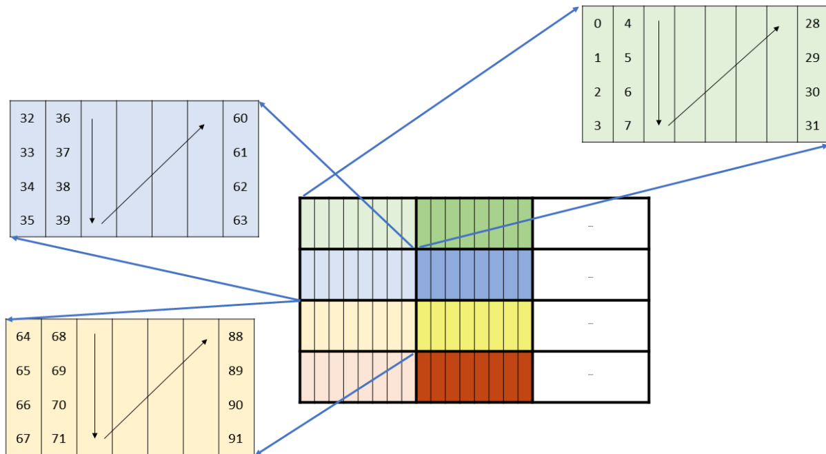
Figure 161: Sparse WGMMMA .m64nNk16 core matrix layout for B
