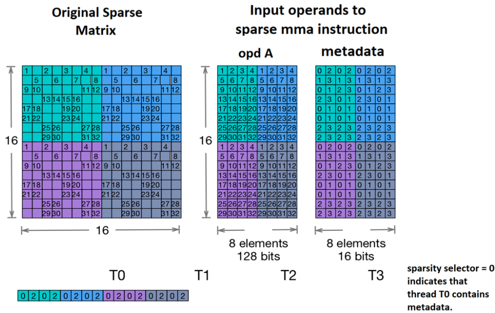
Figure 83: Sparse MMA storage example
