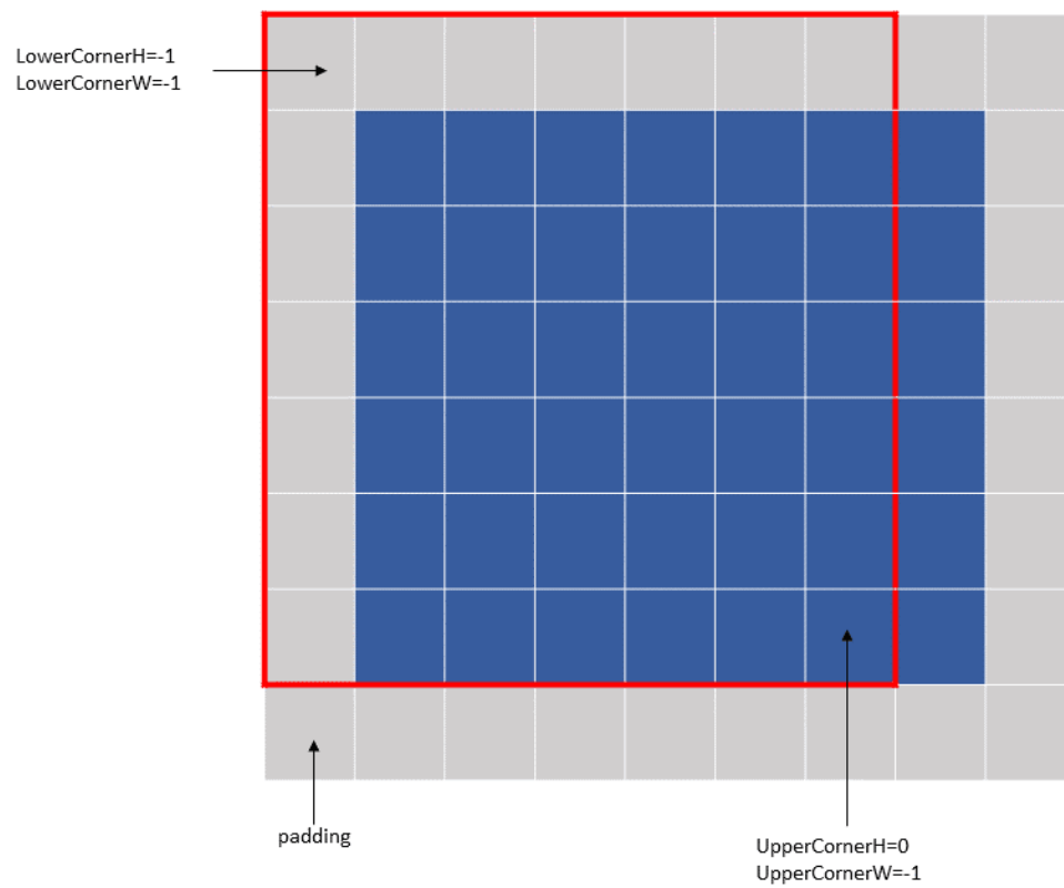
Figure 8: im2col mode bounding box example 2
