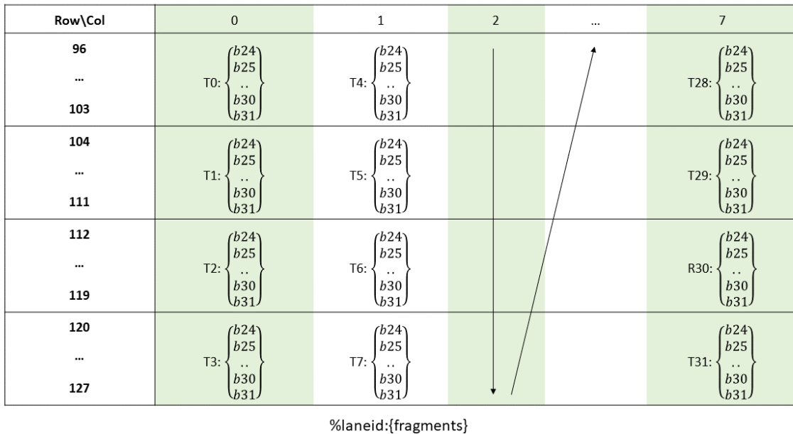
Figure 116: Sparse MMA .m16n8k128 fragment layout for rows 96–127 of matrix B with .u4/.s4 type.
