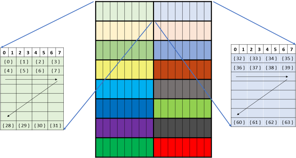
Figure 160: Sparse WGMMMA .m64nNk16 core matrix layout for A
