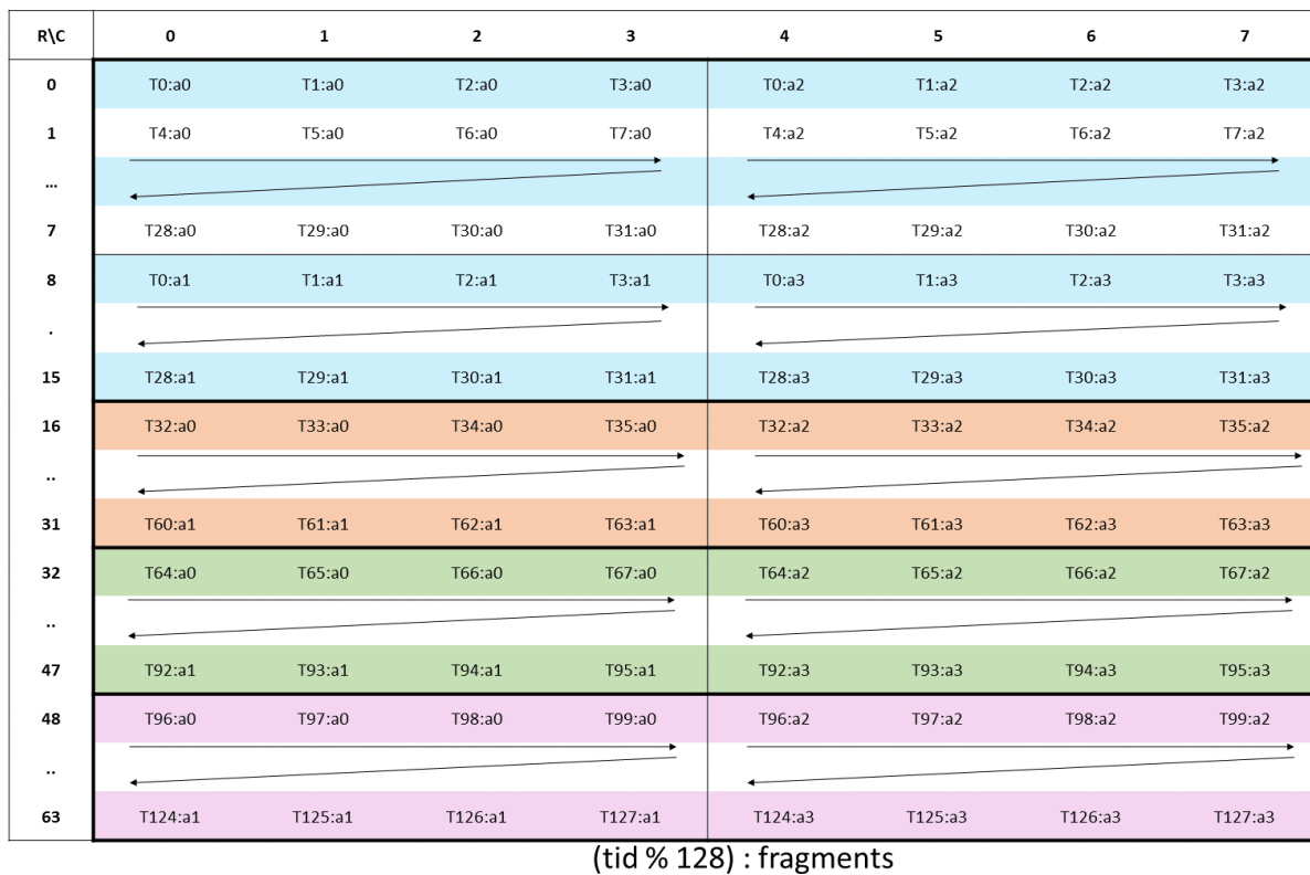
Figure 121: WGMMMA .m64nNk8 register fragment layout for matrix A.
