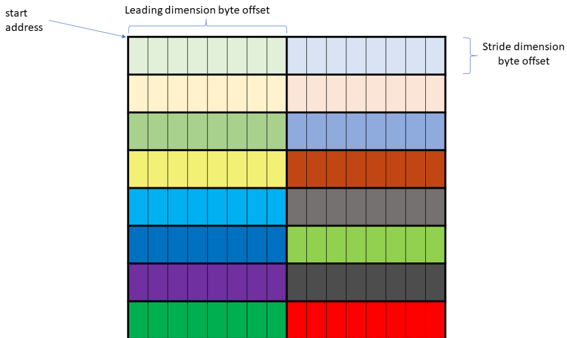
Figure 139: WMMA stride and leading dimension byte offset for matrix A
