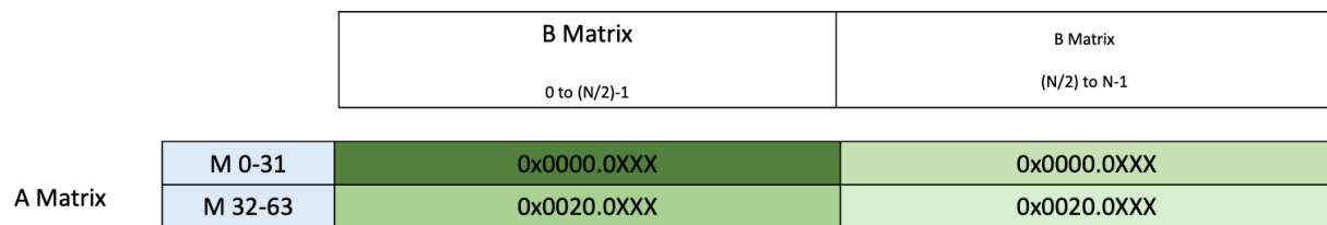
Figure 214: Addresses to use in tcgen05.ld / tcgen05.st
