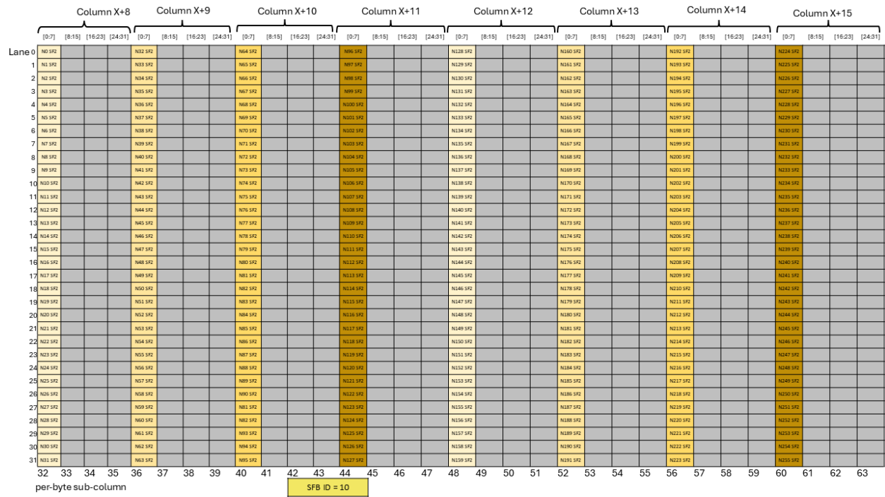
Figure 250: Layout of scale factor B matrix with block32 with K=96 and N>128 with SFA_ID=10
