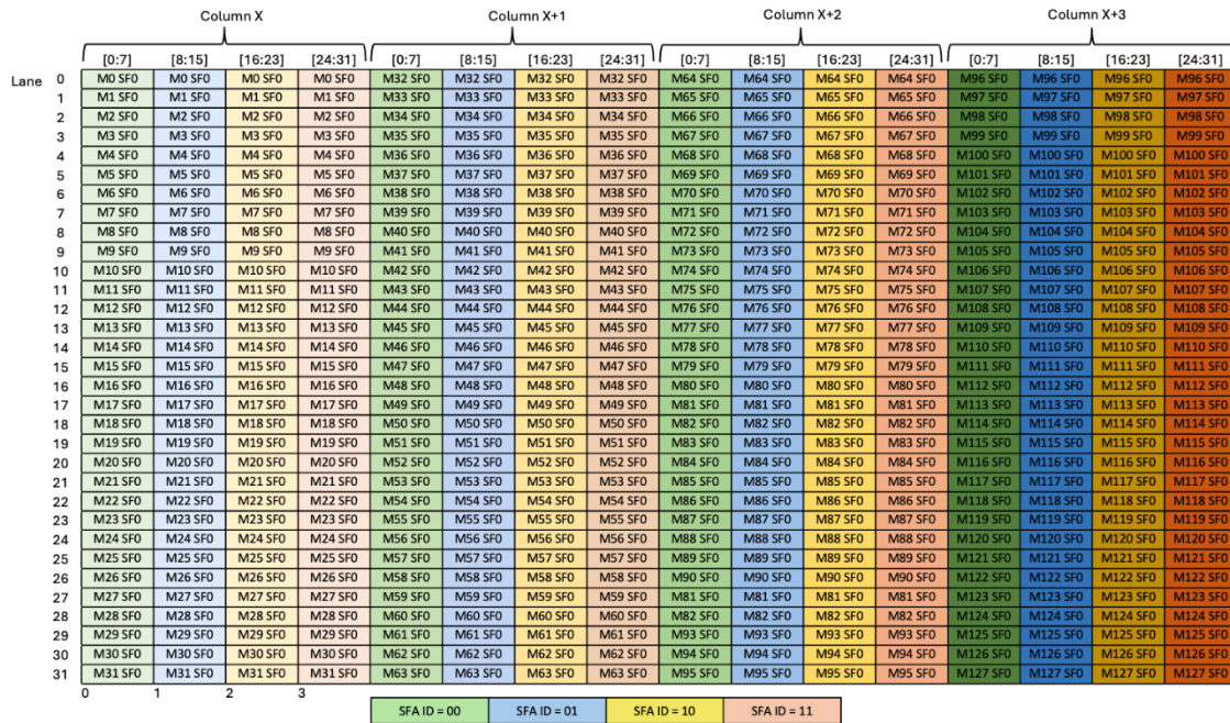
Figure 231: Layout of scale factor A matrix with scale_vec::1X/block32 with K=32/K=64
