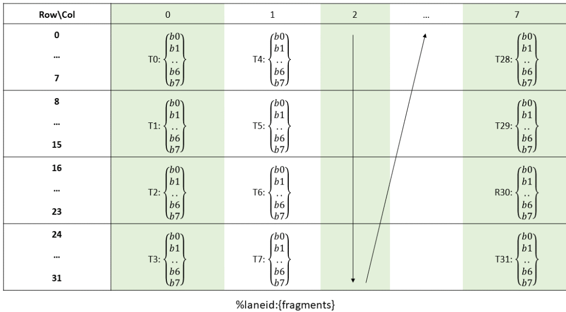
Figure 142: Sparse MMA .m16n8k128 fragment layout for rows 0–31 of matrix B with .u4/.s4/.e2m1 type.
