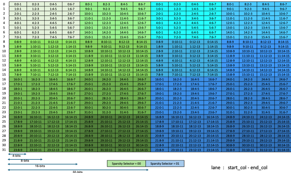
Figure 265: Sparsity Metadata Layout for M = 128 / M = 256 for .kind::tf32
