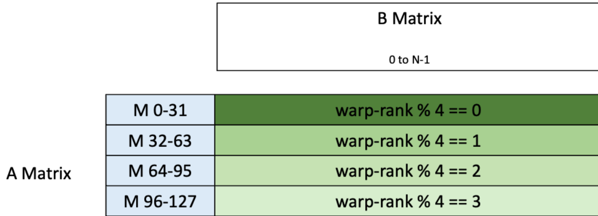
Figure 211: Layout organization for M = 128 + .cta_group::1
