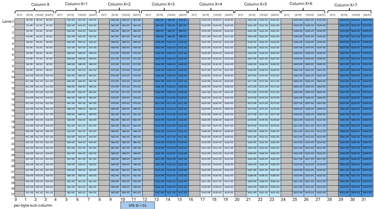
Figure 248: Layout of scale factor B matrix with block32 with K=96 and N>128 with SFA_ID=01
