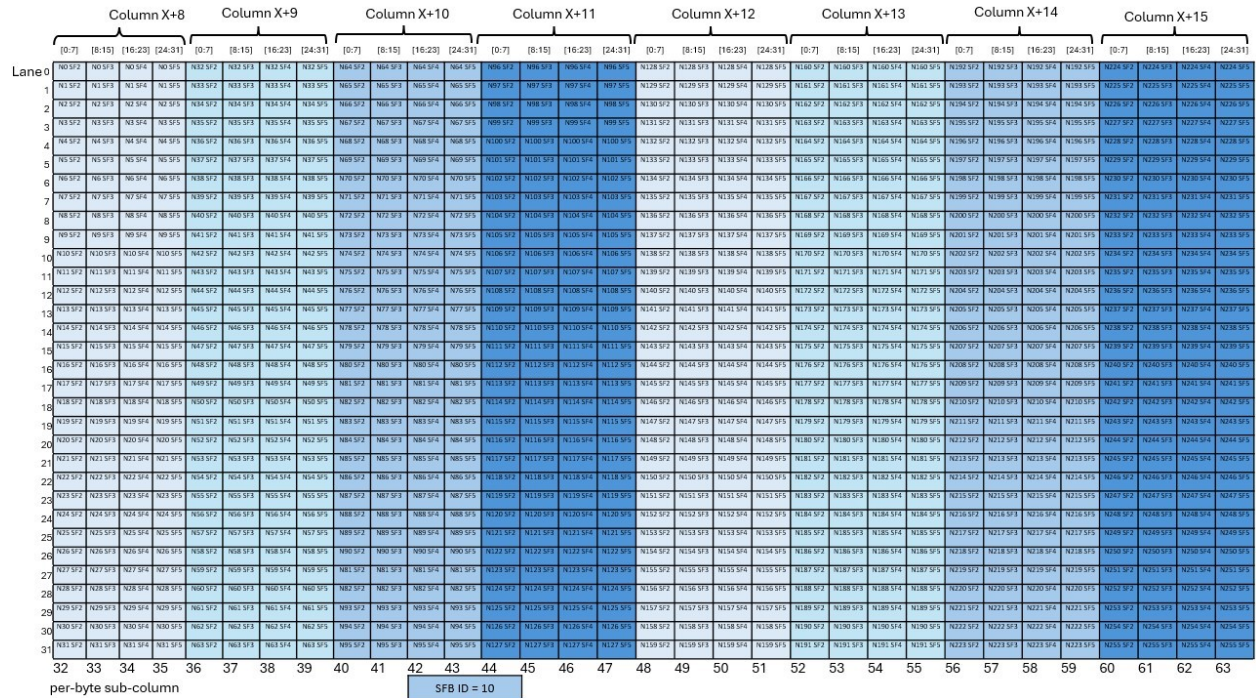
Figure 258: Layout of scale factor B matrix with block16 with K=96 and N>128 with SFA_ID=10
