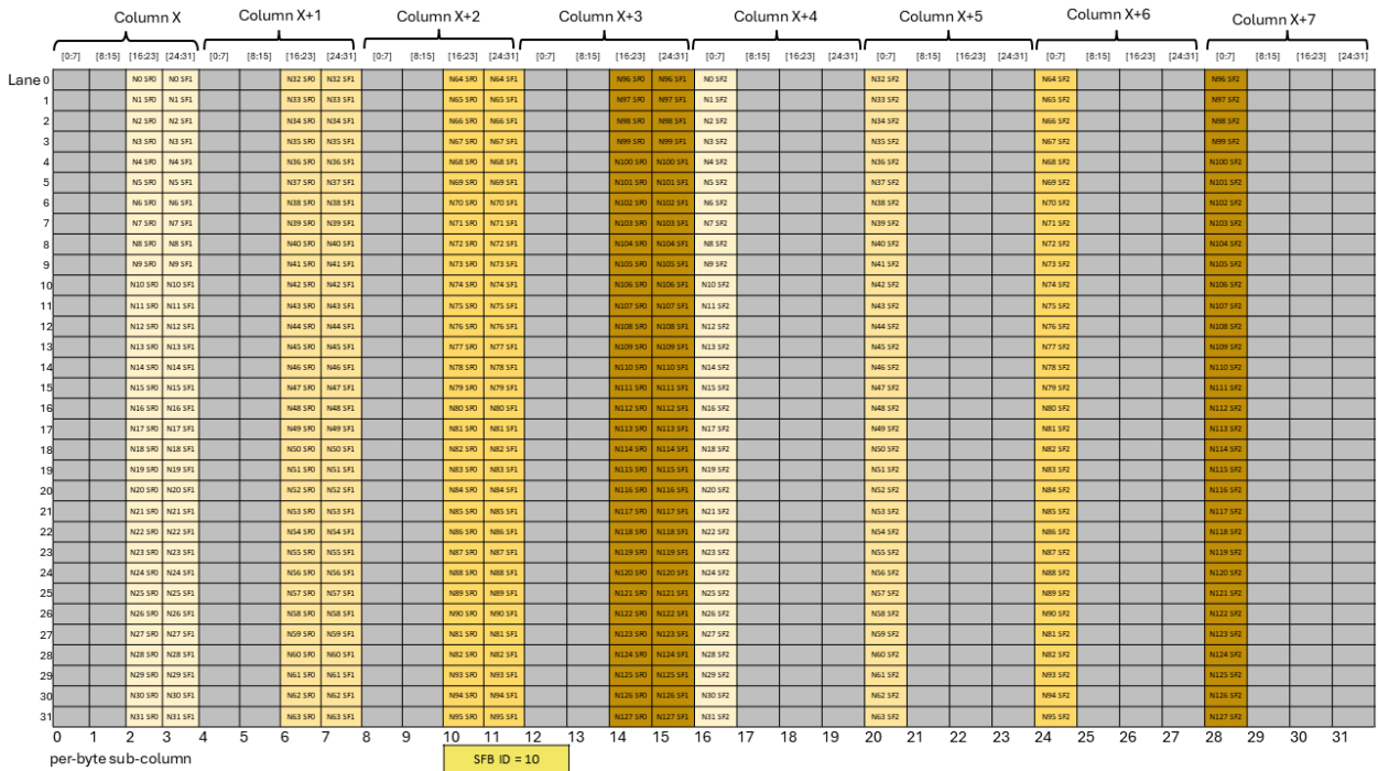
Figure 245: Layout of scale factor B matrix with block32 with K=96 and N<= 128 with SFA_ID=10
