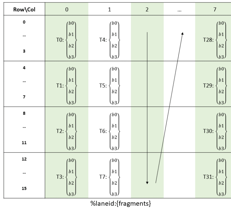
Figure 132: Sparse MMA .m16n8k64 fragment layout for rows 0–15 of matrix B with .u8/.s8/.e4m3/.e5m2/.e3m2/.e2m3/.e2m1 type.
