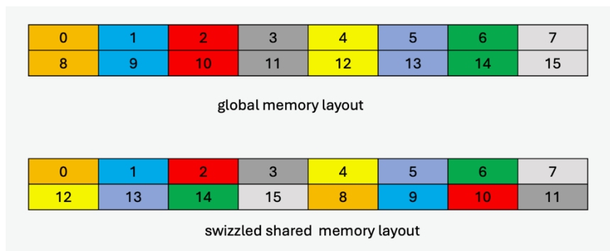
Figure 37: 128-byte swizzle mode example with 64-byte atomicity
