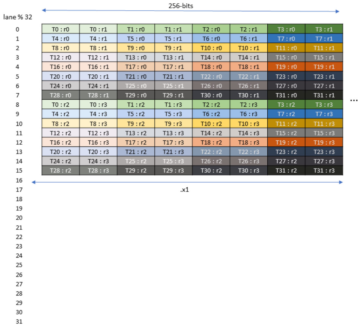
Figure 186: Matrix Fragment for shape .16x256b
