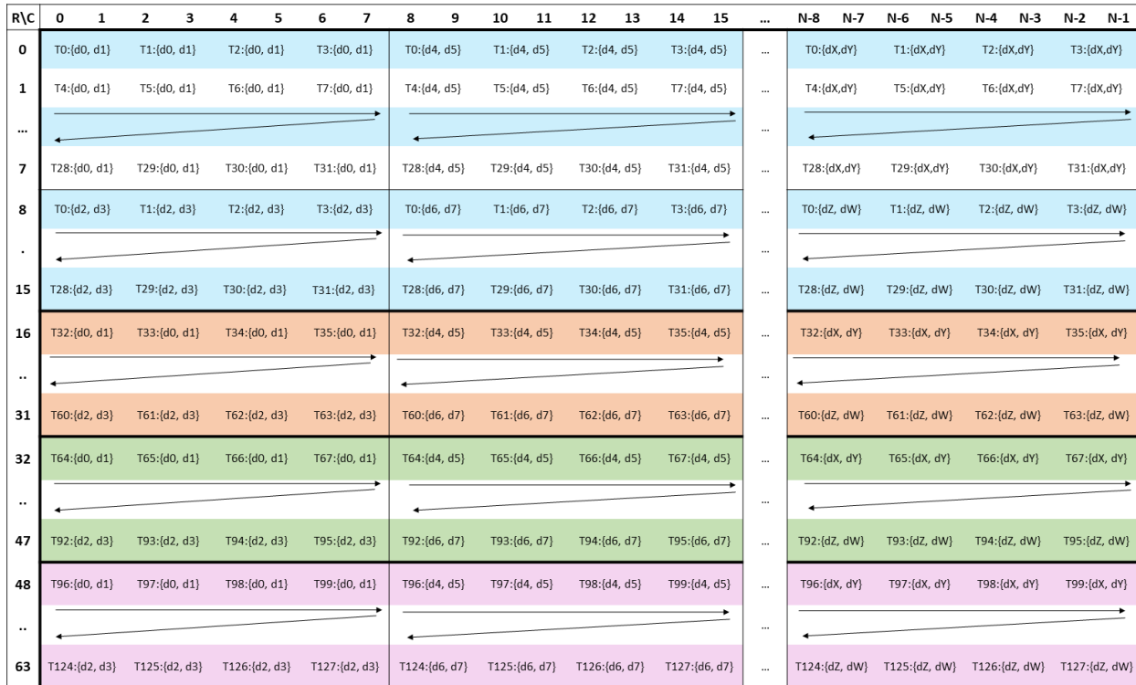
Figure 149: WGMMA .m64nNk16 register fragment layout for accumulator matrix D.
