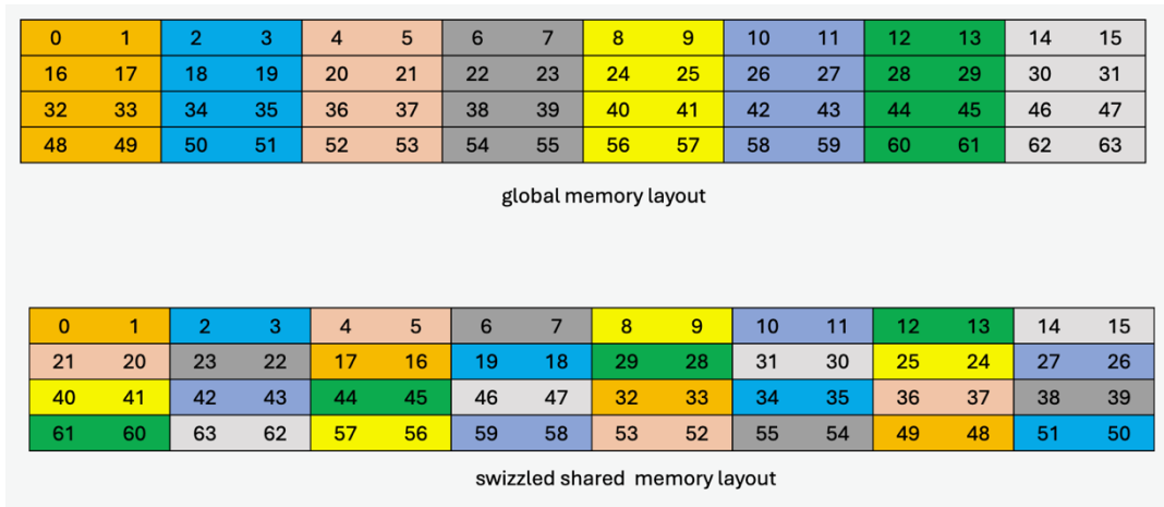
Figure 36: 128-byte swizzle mode example with 32-byte atomicity with 8-byte flip
