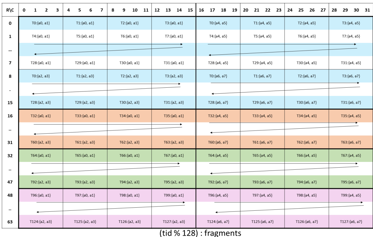
Figure 175: Sparse WGMMA .m64nNk32 fragment layout for matrix A with .f16/.bf16 type.
