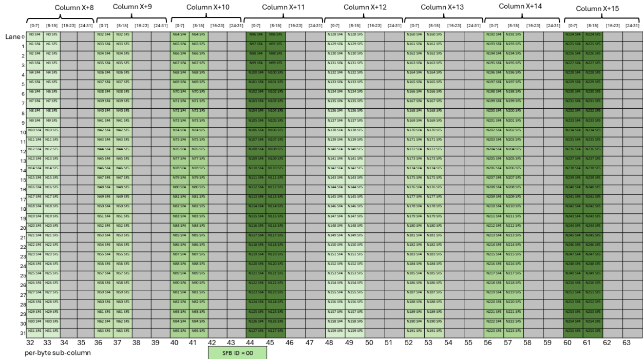
Figure 256: Layout of scale factor B matrix with block16 with K=96 and N>128 with SFA_ID=00
