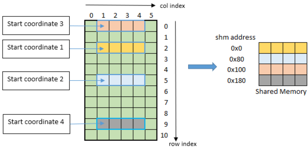
Figure 10: tiled::scatter4/tiled::gather4 mode bounding box example
