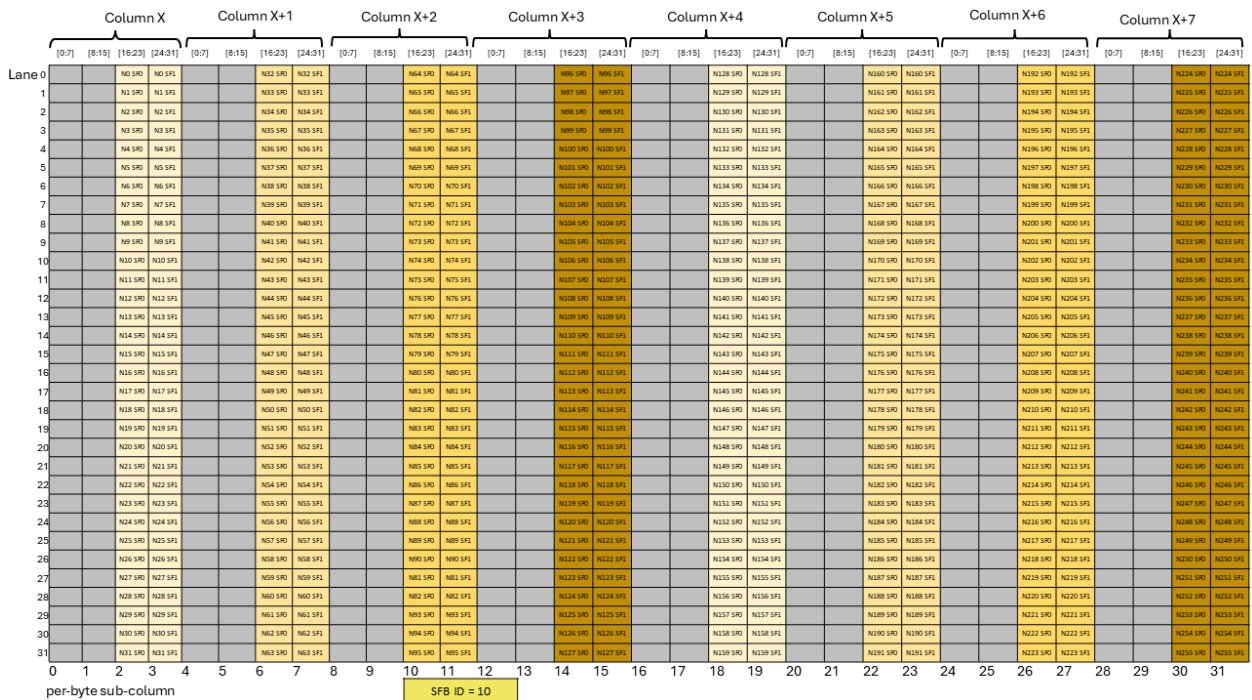
Figure 249: Layout of scale factor B matrix with block32 with K=96 and N>128 with SFA_ID=10
