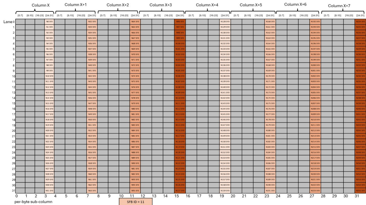
Figure 251: Layout of scale factor B matrix with block32 with K=96 and N>128 with SFA_ID=11
