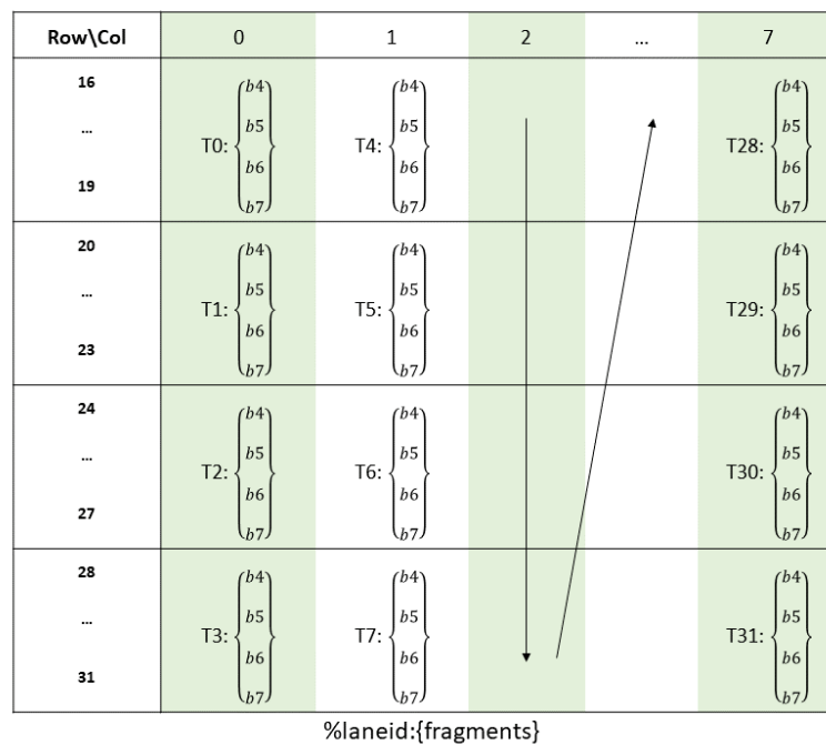
Figure 133: Sparse MMA .m16n8k64 fragment layout for rows 16–31 of matrix B with .u8/.s8/.e4m3/.e5m2/.e3m2/.e2m3/.e2m1 type.
