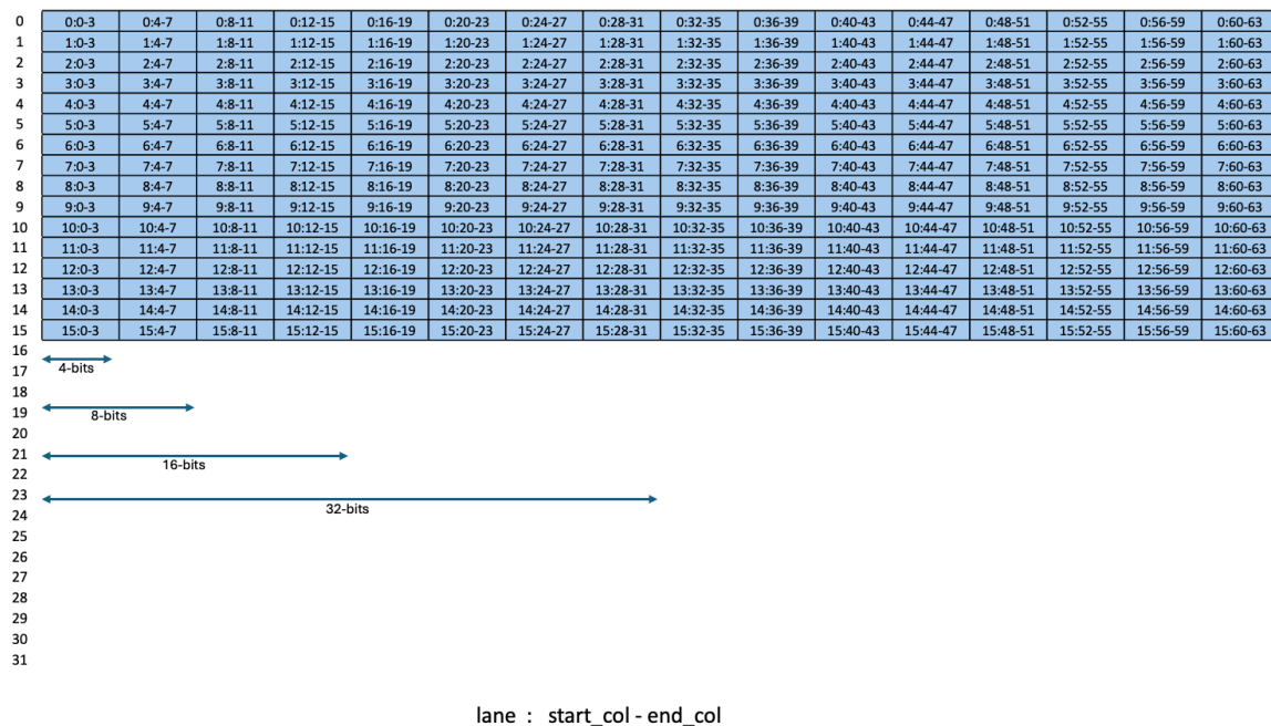
Figure 266: Sparsity Metadata Layout for M = 64 for .kind::f8f6f4, .kind::mx4f8f6f4, .kind::i8, .kind::mx4f4, .kind::mx4f4nvf4
