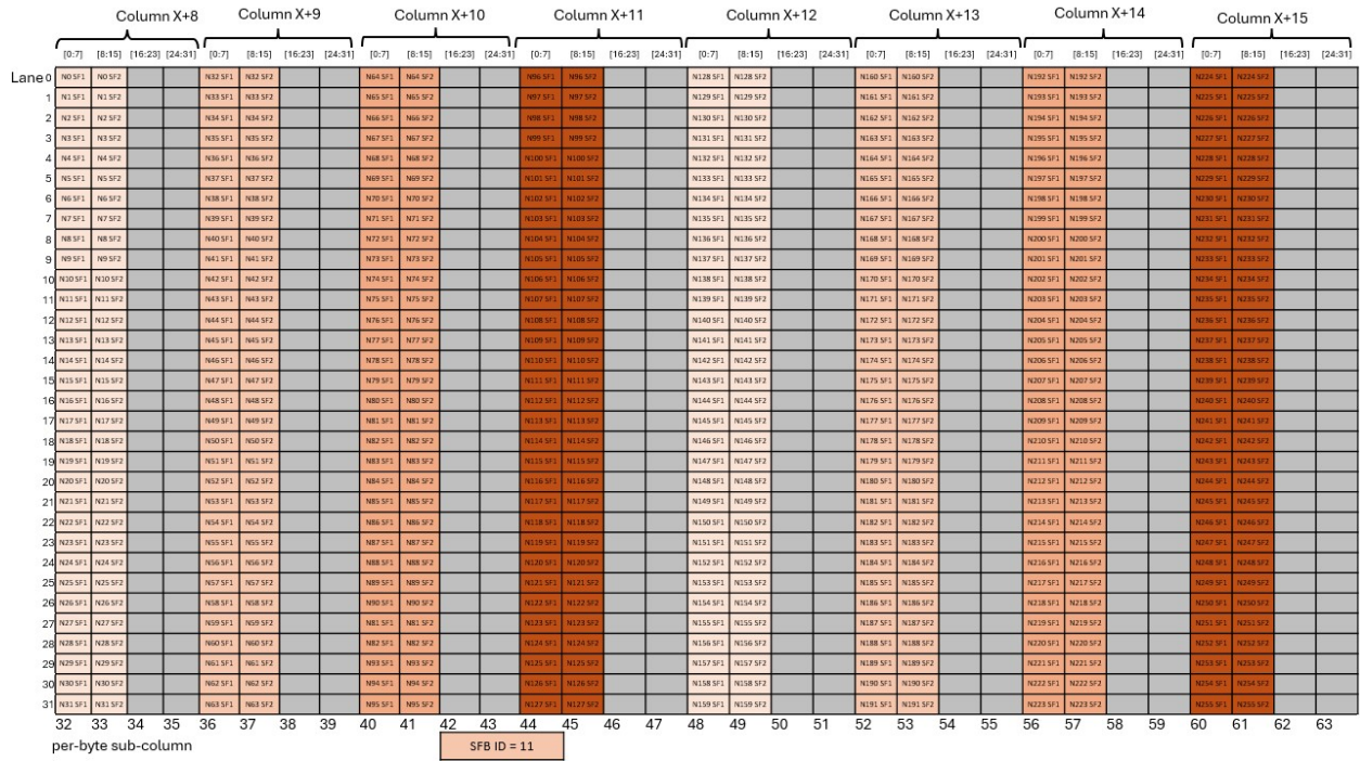
Figure 252: Layout of scale factor B matrix with block32 with K=96 and N>128 with SFA_ID=11
