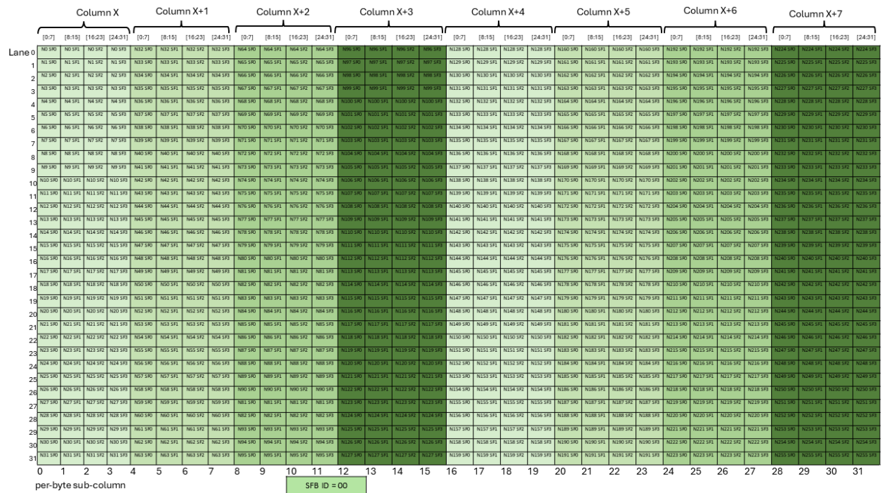
Figure 255: Layout of scale factor B matrix with block 16 with K=96 and N>128 with SFA_ID=00
