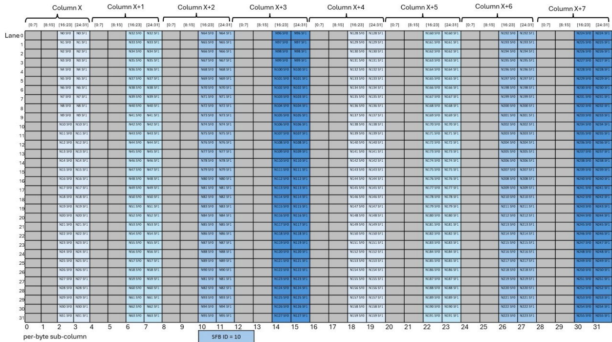
Figure 257: Layout of scale factor B matrix with block16 with K=96 and N>128 with SFA_ID=10
