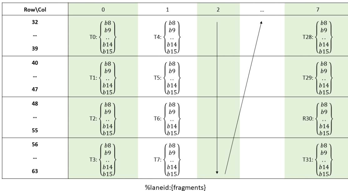
Figure 143: Sparse MMA .m16n8k128 fragment layout for rows 32–63 of matrix B with .u4/.s4/.e2m1 type.
