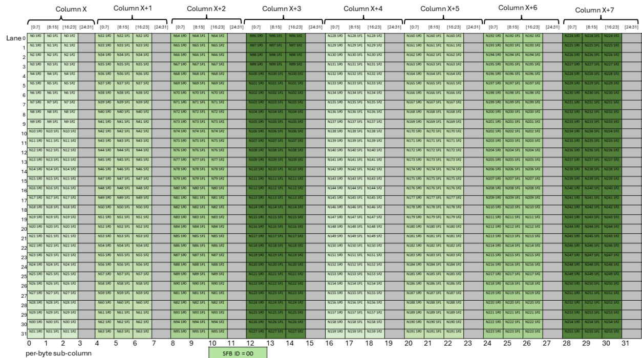
Figure 247: Layout of scale factor B matrix with block32 with K=96 and N>128 with SFA_ID=00
