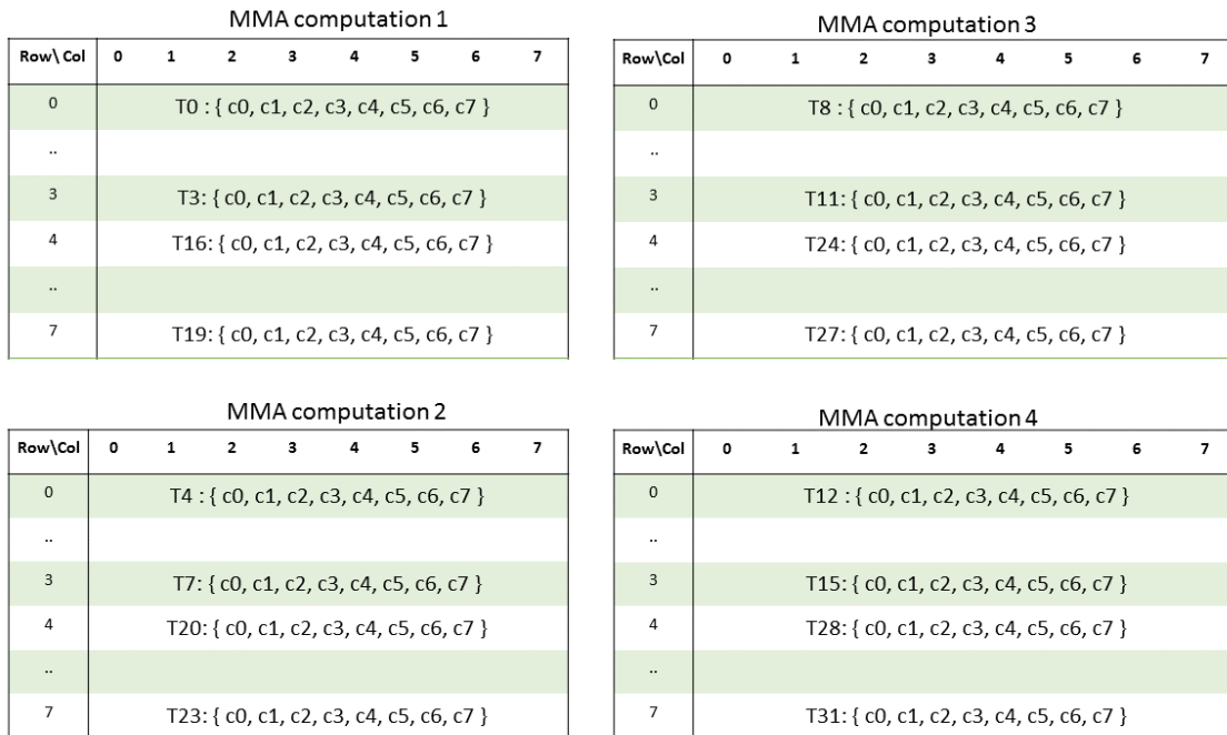
Figure 50: MMA .m8n8k4 fragment layout for matrix C/D with .ctype = .f16
