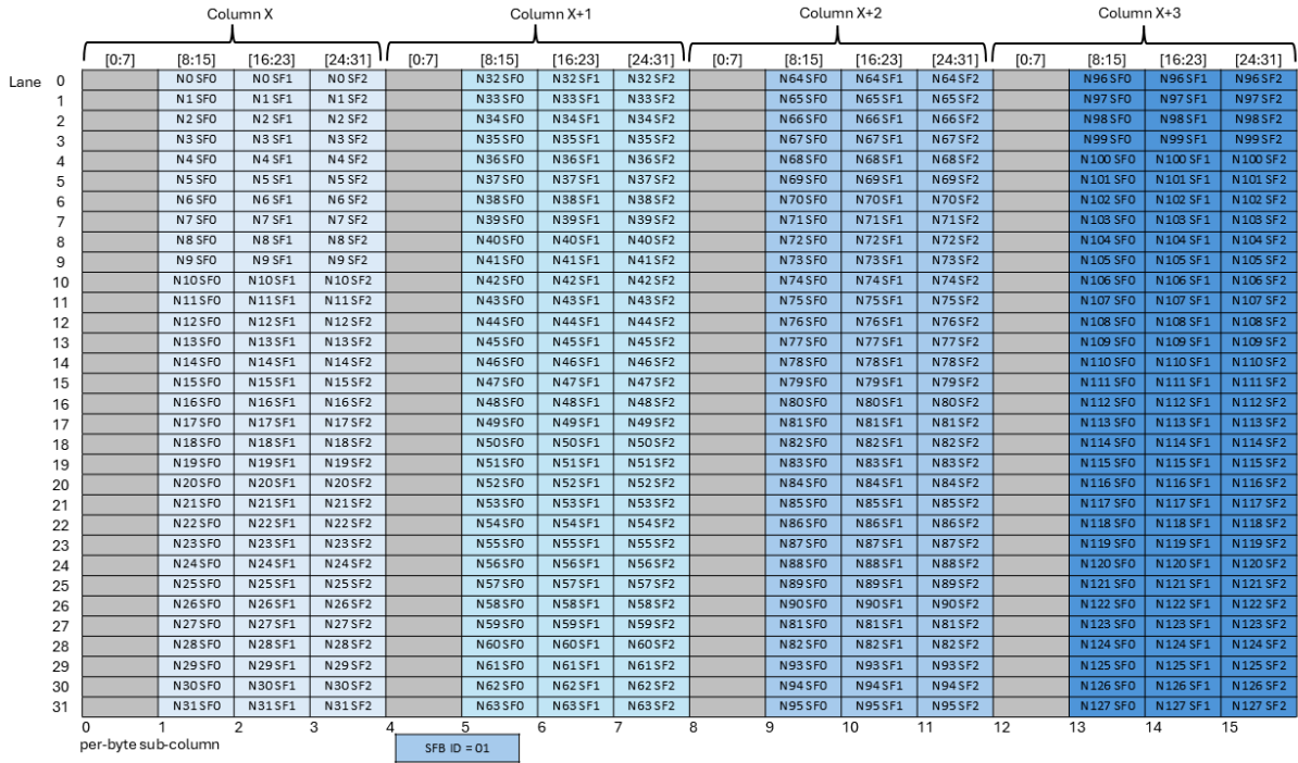
Figure 244: Layout of scale factor B matrix with block32 with K=96 and N<= 128 with SFA_ID=01
