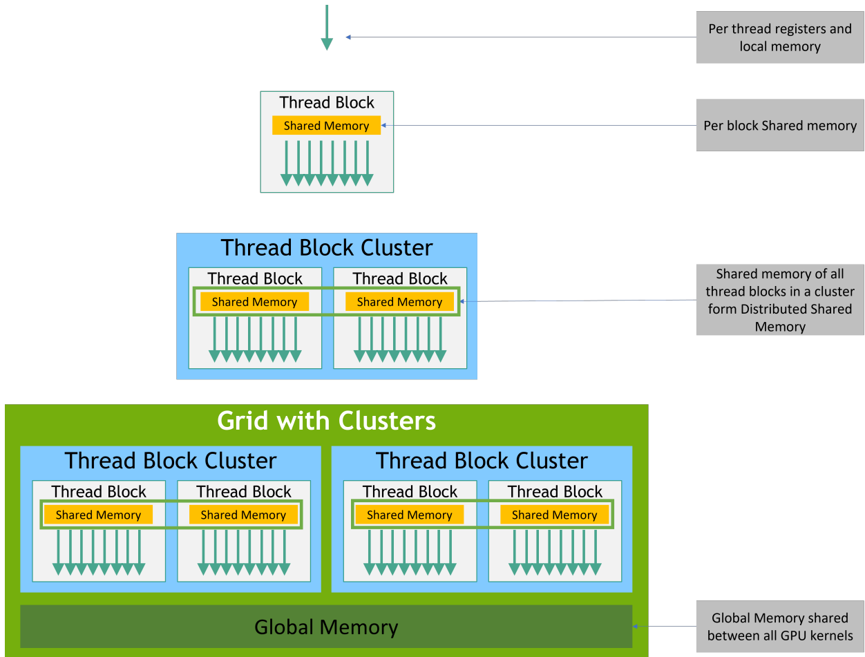
Figure 6: Memory Hierarchy
