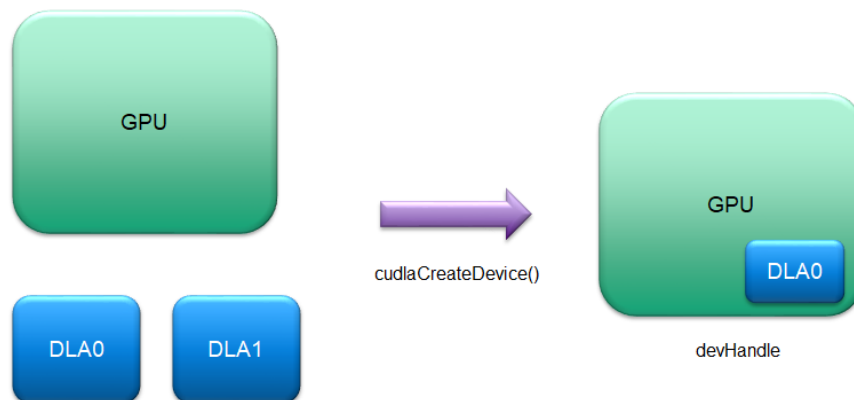
Figure 6: Device model
