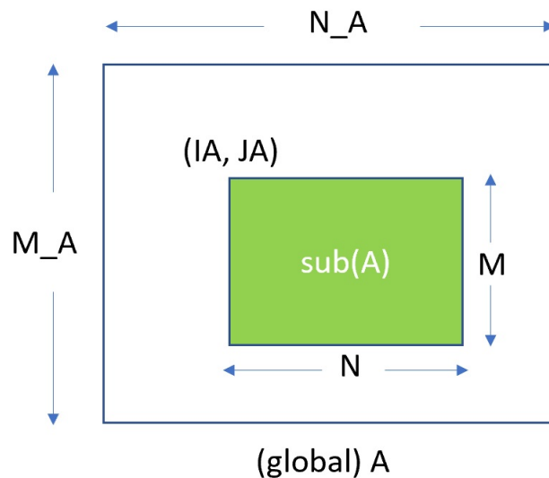
Fig. 2: global matrix and local matrix
