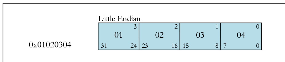
Figure 1 Bit Numbering
