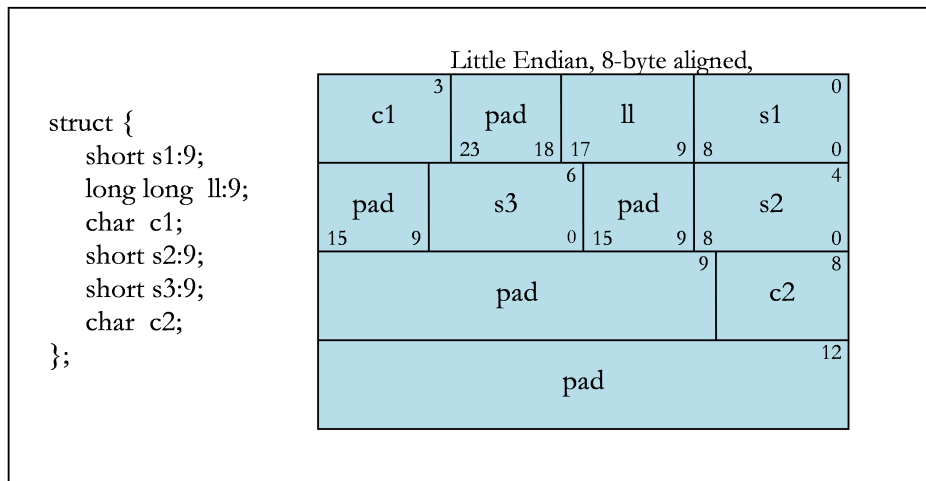
Figure 3 Boundary Alignment
