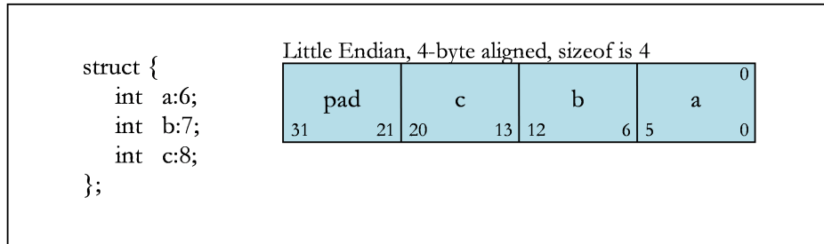
Figure 2 Bit-field Allocation
