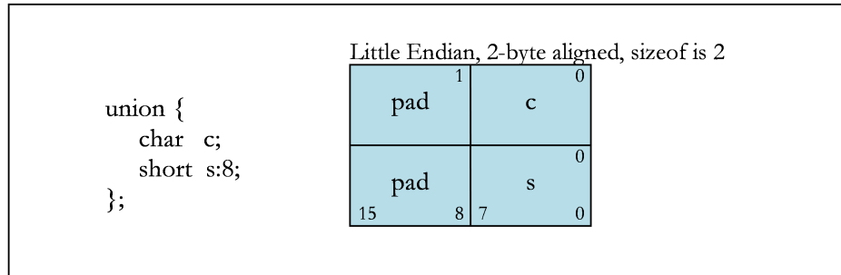
Figure 5 Union Allocation
