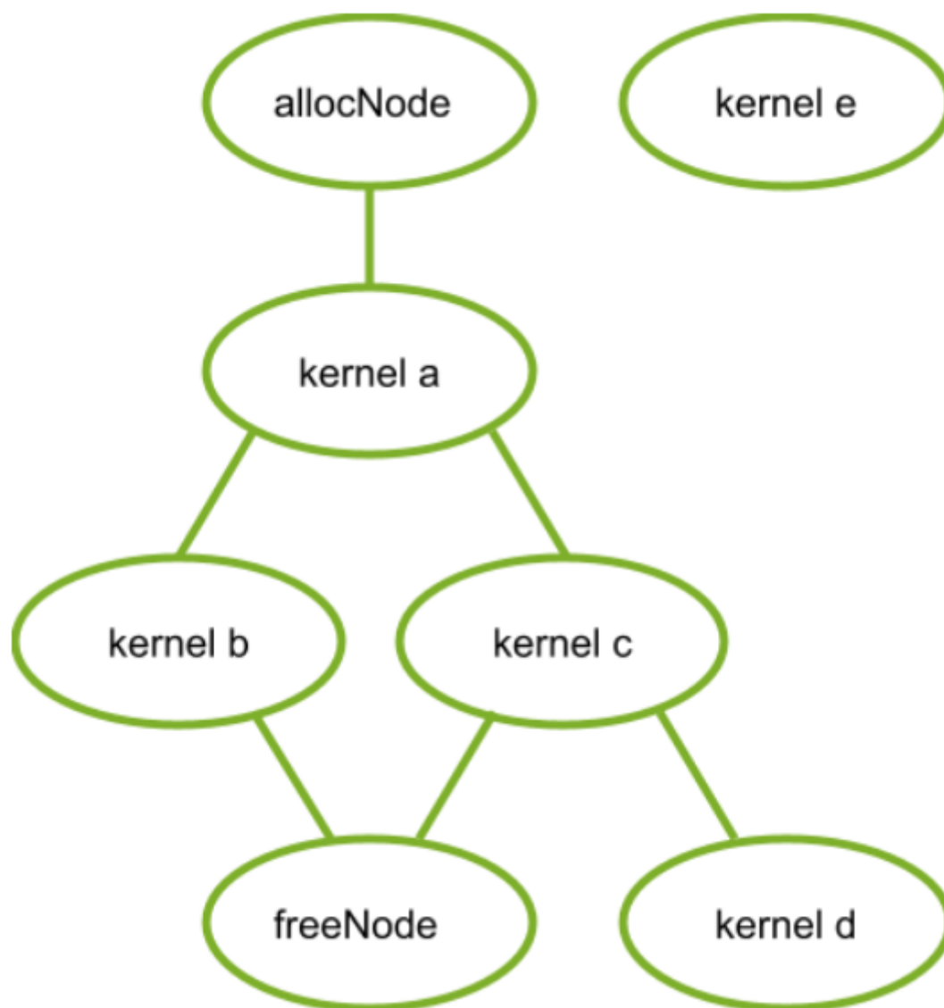
Figure 27: Kernel Nodes
