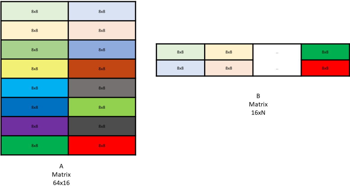
Figure 127: WGMMA .m64nNk16 core matrices for A and B
