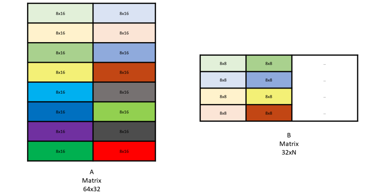
Figure 156: Sparse WGMMA .m64nNk32 core matrices for A and B
