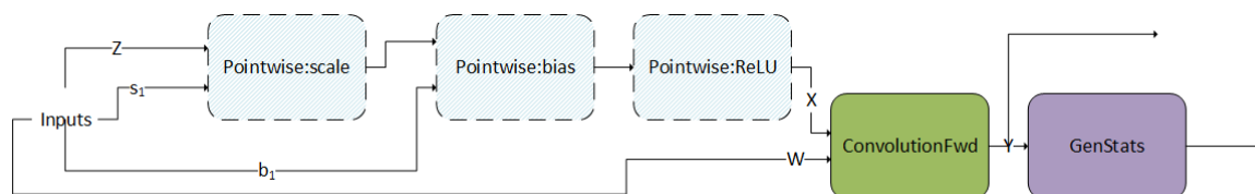
Figure 20. The pre-compiled ConvBNfprop engine fuses several pointwise operations with ConvolutionFwd and GenStats .
