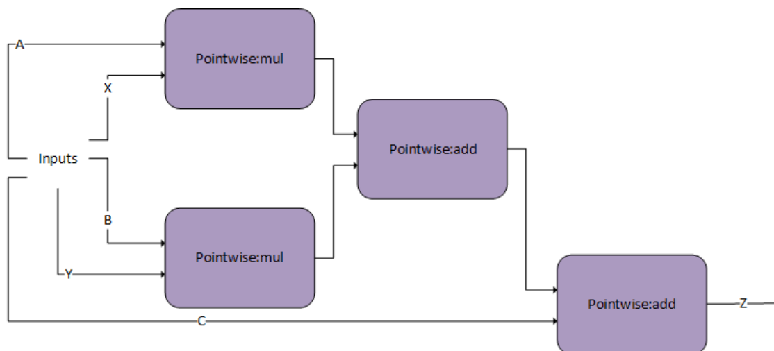
Figure 24. The pre-compiled engine, dBNApplY
