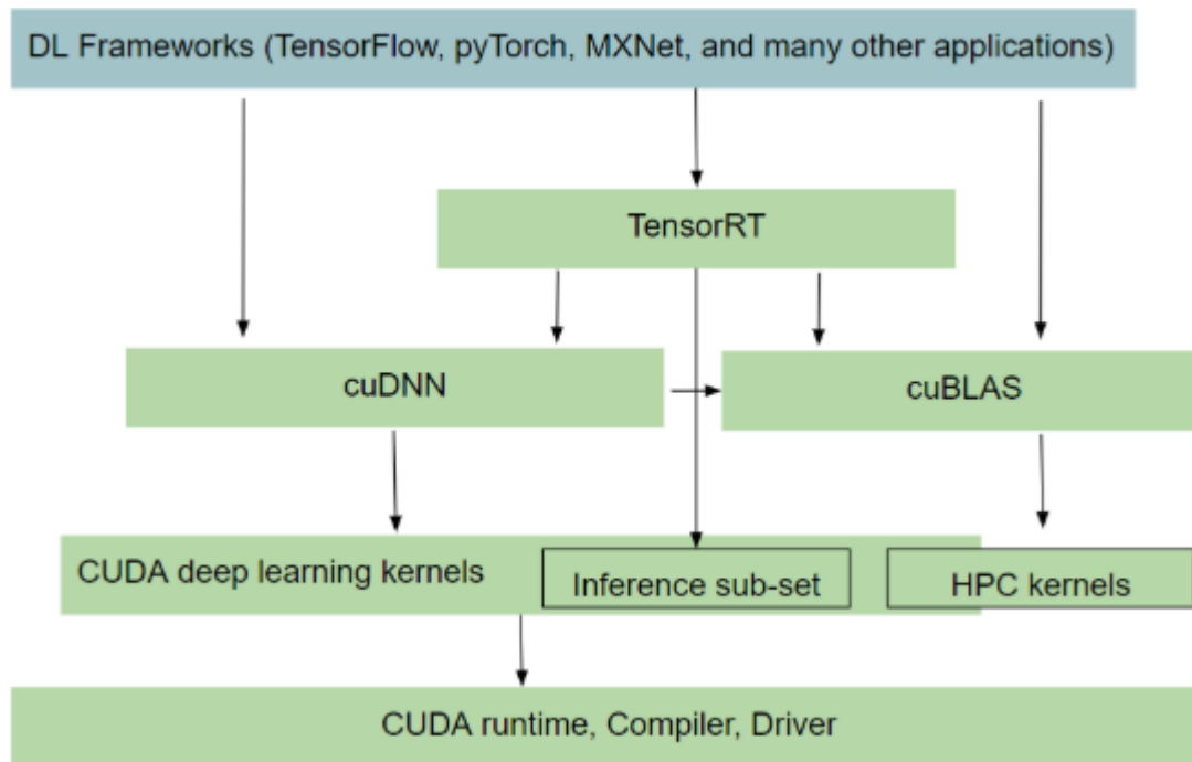
Figure 27. Software stack with cuDNN.
