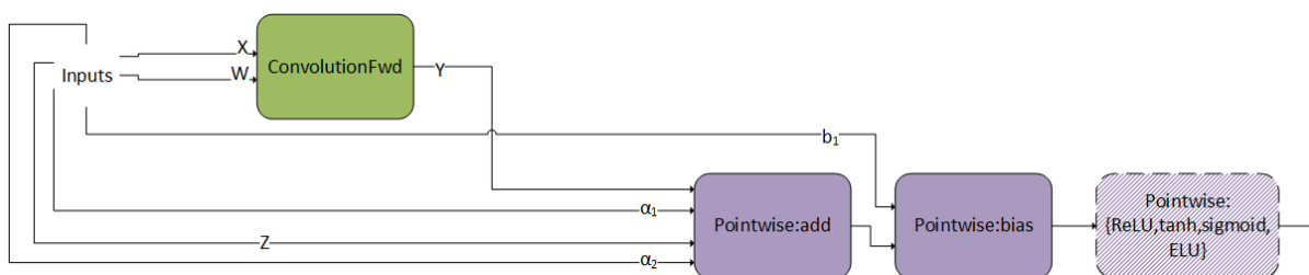
Figure 22. ConvBiasAct , another pre-compiled engine, fuses ConvolutionFwd with several pointwise operations.
