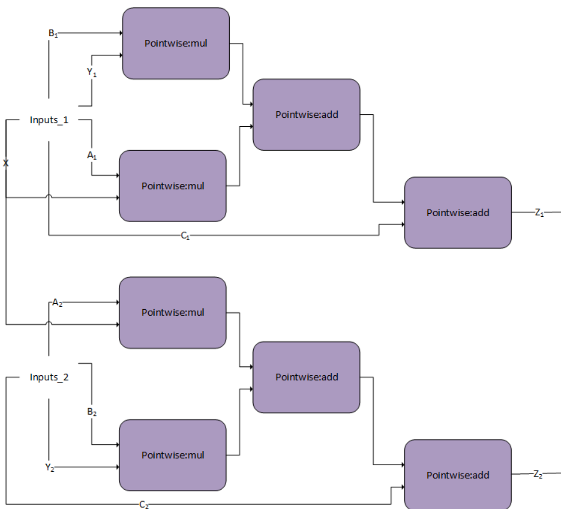
Figure 25. The DualdBNapply engine
