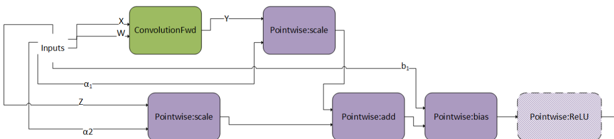
Figure 23. The pre-compiled engine, ConvScaleBiasAct
