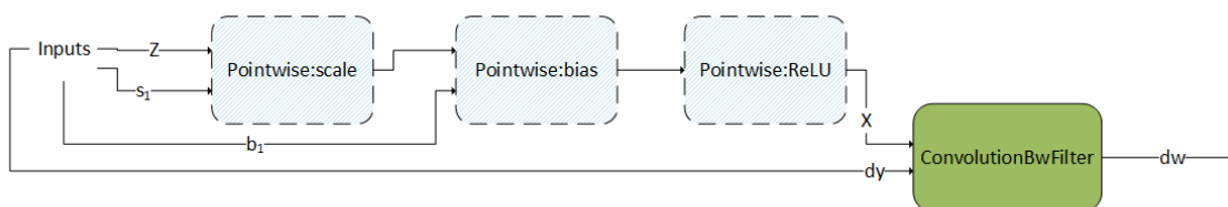
Figure 21. The ConvBNwgrad pre-compiled engine fuses several (optional) pointwise operations with ConvolutionBwFilter .
