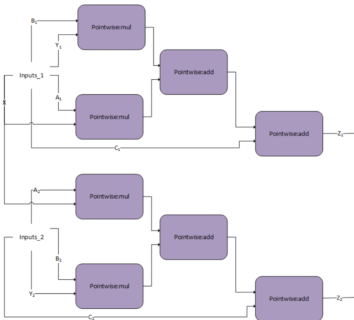
Figure 26. The DualdBNapply engine
