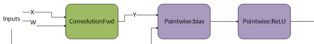
Figure 16. ConvolutionFwd Followed by a DAG with Two Operations
