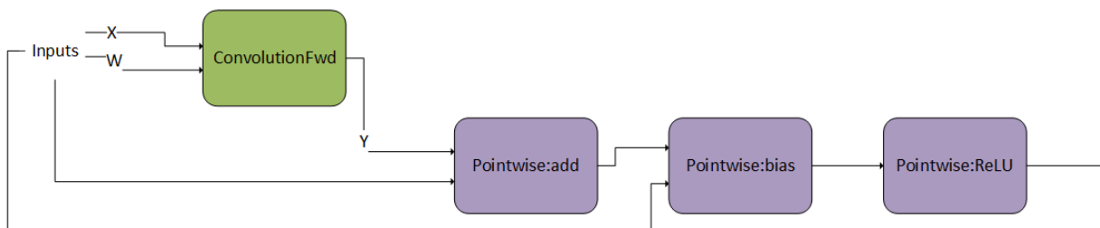
Figure 17. ConvolutionFwd Followed by a DAG with Three Operations
