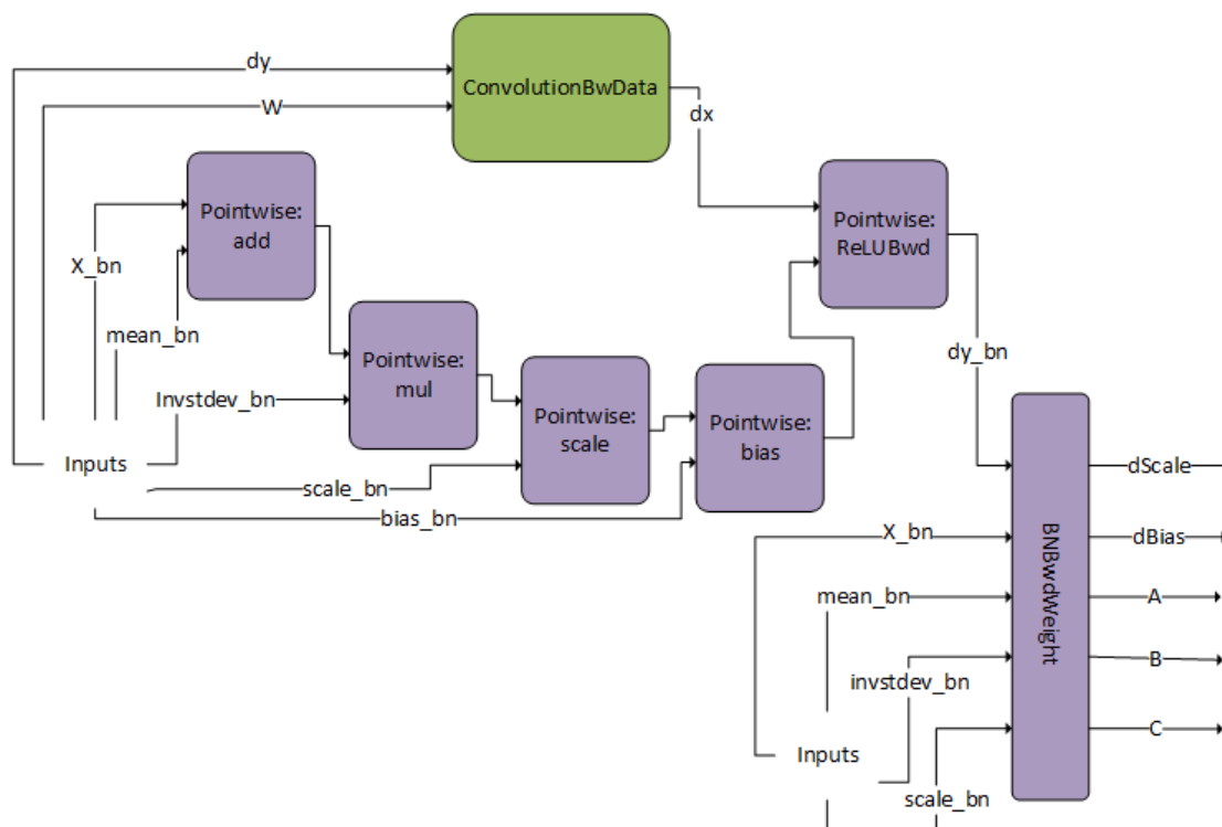
Figure 27. DgradDreluBNBwdWeight is a pre-compiled engine that can be used in conjunction with the dBNApplY pattern to compute the backwards path of batch norm.
