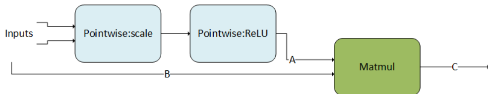
Figure 18. MatMul Preceded by a DAG with Two Operations
