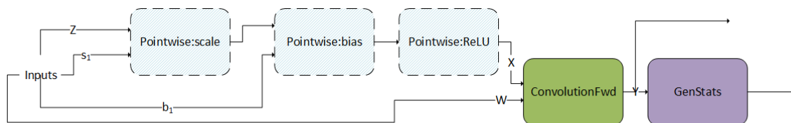
Figure 26. The pre-compiled ConvBNfprop engine fuses several pointwise operations with ConvolutionFwd and GenStats .
