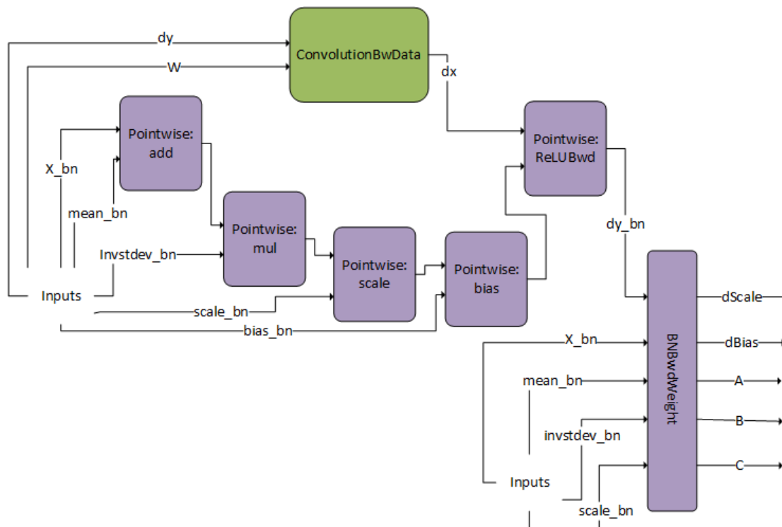
Figure 32. DgradDreluBNBwdWeight is a pre-compiled engine that can be used in conjunction with the dBNAApply pattern to compute the backwards path of batch norm.
