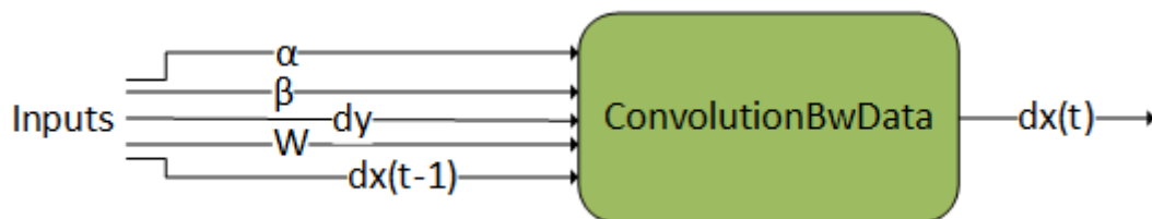
Figure 10. ConvolutionBwData Engine
