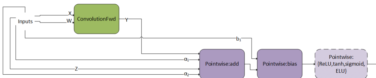
Figure 41. ConvBiasAct, A Pre-Compiled Engine, Fuses ConvolutionFwd With Several Pointwise Operations
