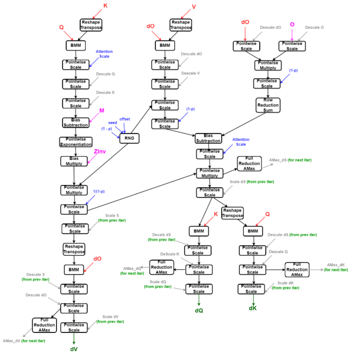
Figure 46. FP8 Fused Multi-Head Attention Backward Pass Operation Graph
