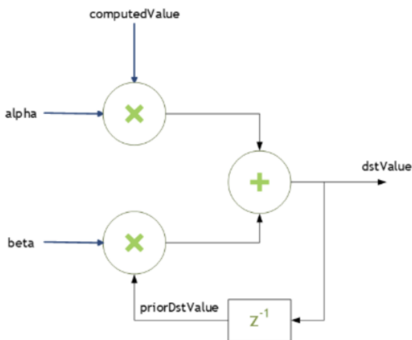
Figure 48. Scaling Parameters for Convolution
