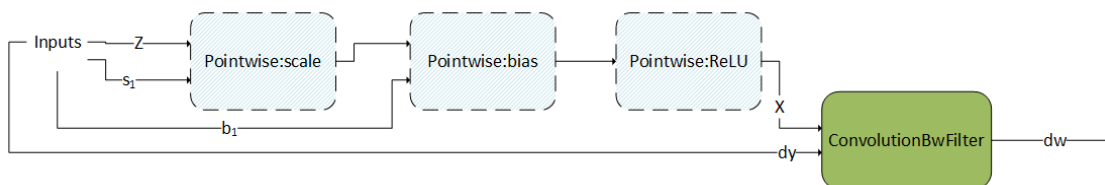
Figure 40. ConvBNwgrad, A Pre-Compiled Engine, Fuses ConvolutionBwFilter With Several (Optional) Pointwise Operations
