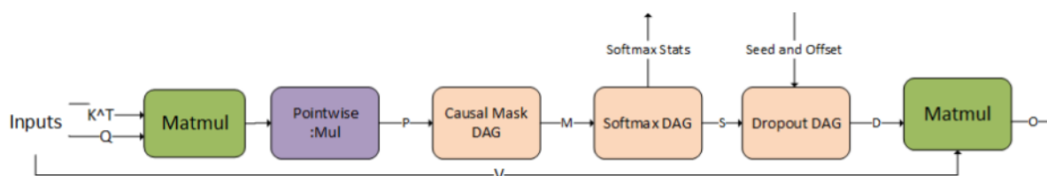
Figure 33. Flash fprop cuDNN Operation Graph
