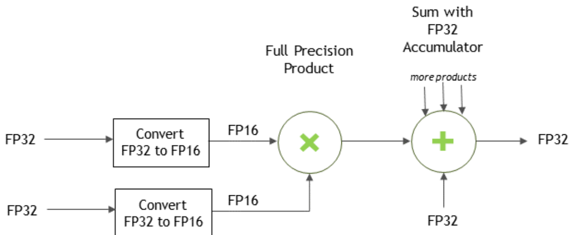
Figure 47. Tensor Operation with FP32 Inputs
