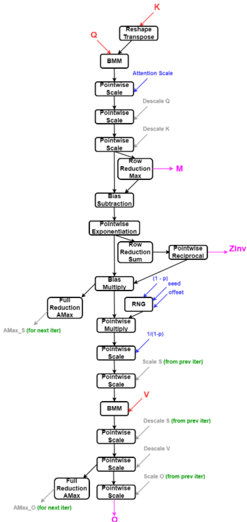
Figure 45. FP8 Fused Multi-Head Attention Forward Pass Operation Graph
