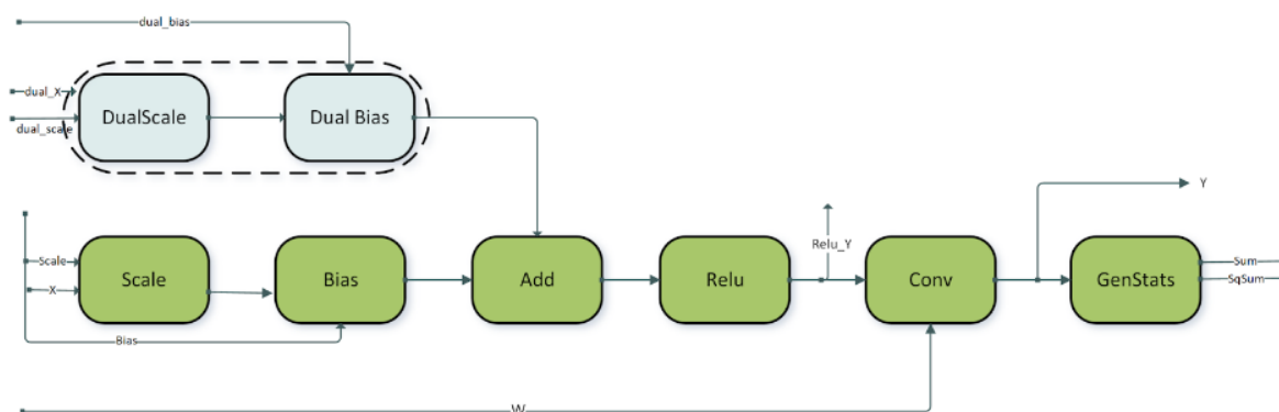
Figure 39. DBARCS In The convBNfprop Series For Supporting Fusions Across Skip Connections
