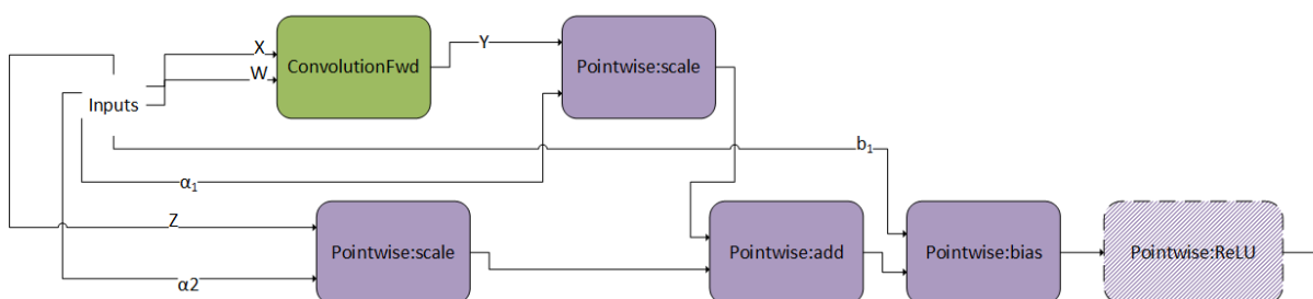
Figure 42. ConvScaleBiasAct, A Pre-Compiled Engine
