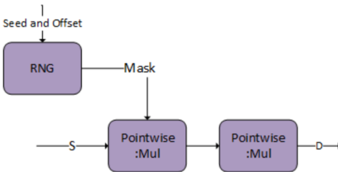
Figure 36. Flash _{fprop} Dropout Operation Graph
