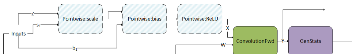
Figure 38. ConvBNfprop, A Pre-Compiled Engine, Fuses ConvolutionFwd and GenStats With Several Pointwise Operations
