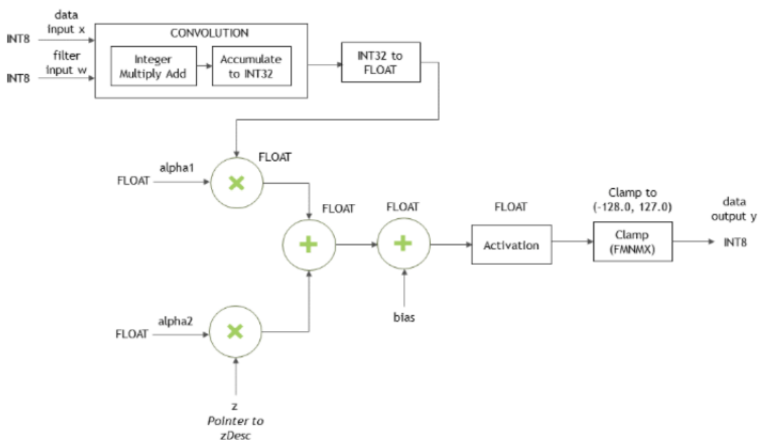
Figure 49. INT8 for cudaConvolutionBiasActivationForward
