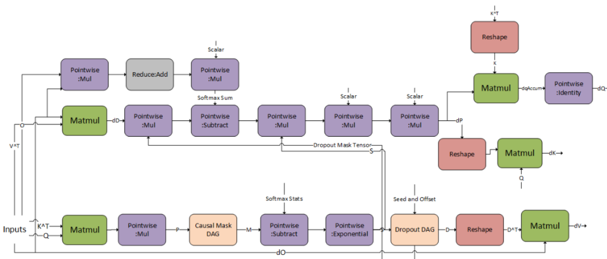
Figure 37. Flash bprop cuDNN Operation Graph
