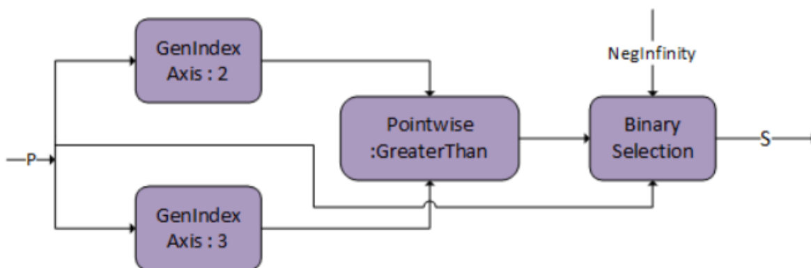
Figure 34. Flash fprop Causal Mask Operation Graph
