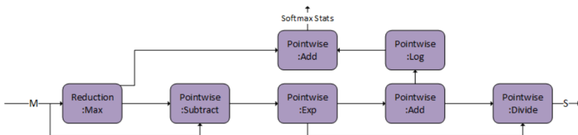
Figure 35. Flash _{fprop} Softmax Operation Graph
