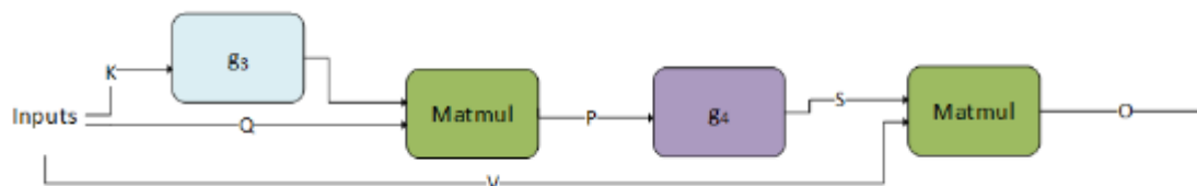
Figure 23. Mha-fprop cuDNN Operation Graph
