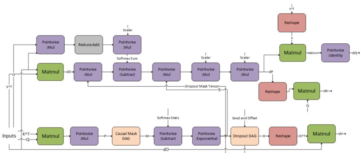
Figure 39. Flash bprop cuDNN Operation Graph
