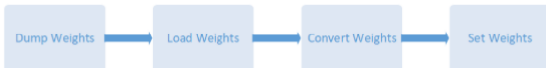
Figure 12 TensorFlow RNN Workflow
