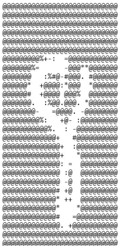
Figure 3 ASCII output
