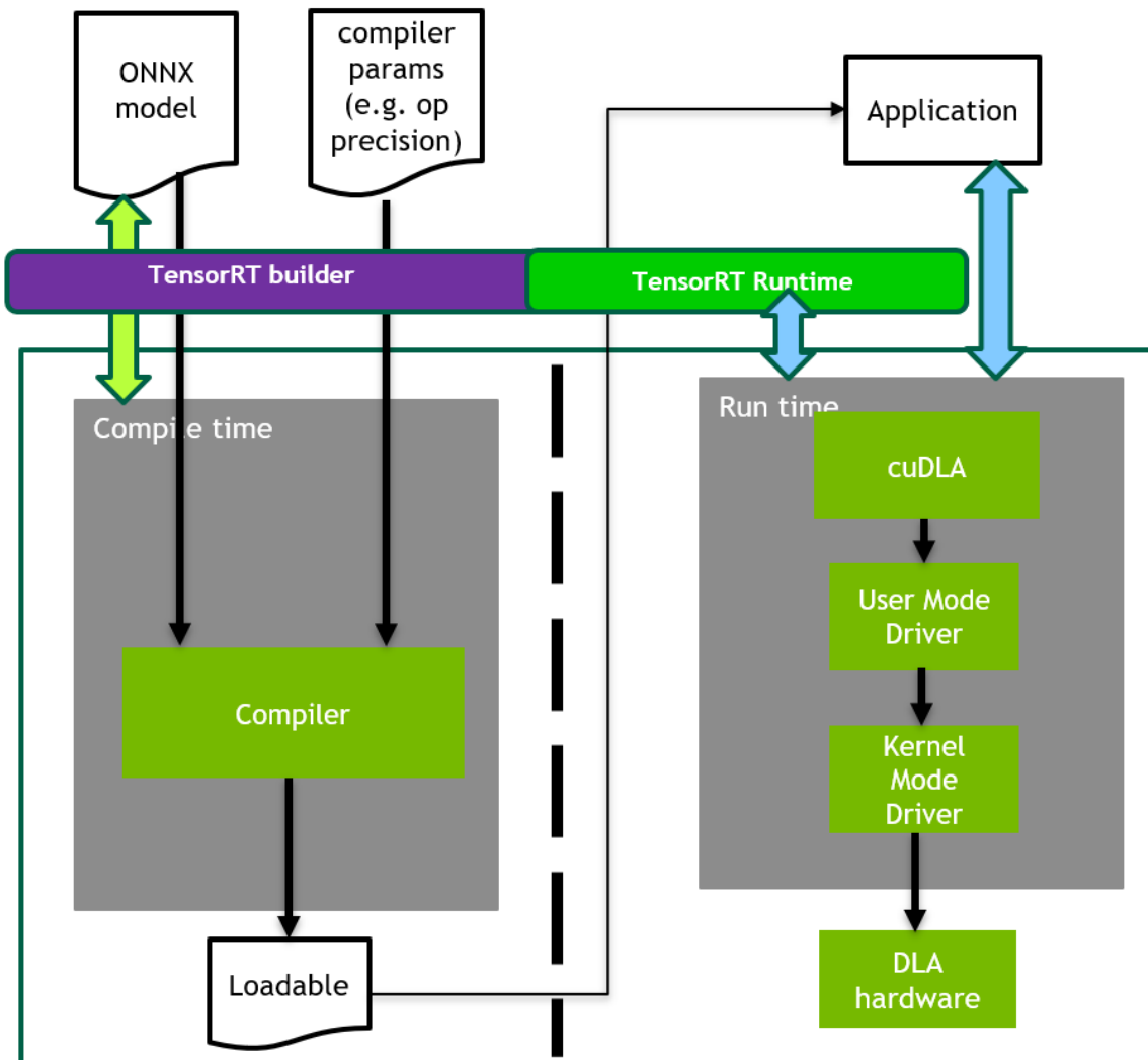
Figure 17. Workflow for the Building and Runtime Phases of DLA
