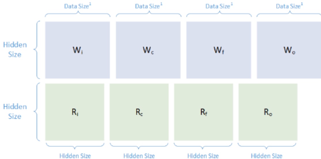
Figure 7 Converted tensors
